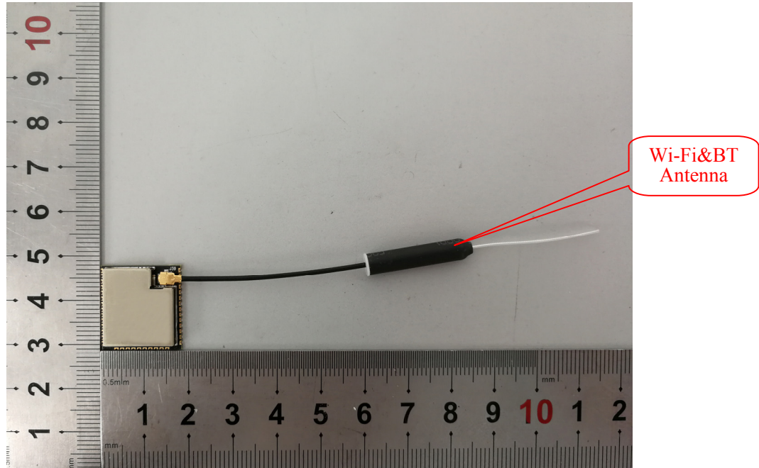
EUT with Dipole Antenna View
