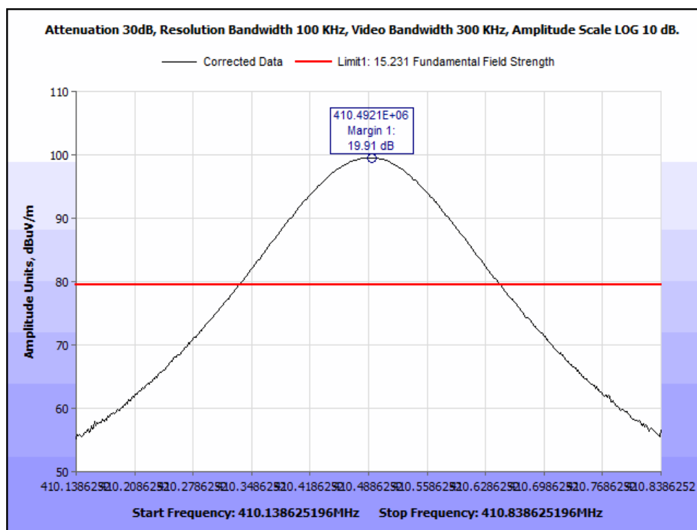
Plot 4. Field Strength of Fundamental, 410.5 MHz Low Channel
