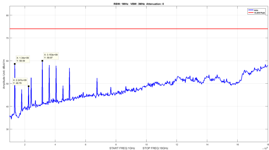
Plot 15. Radiated Emissions, 1 – 18 GHz, 450 MHz, High Channel Peak
