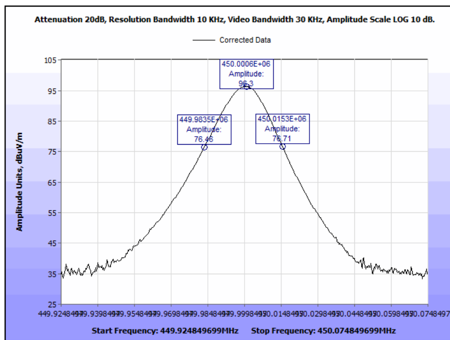
Plot 8. 20 dB Bandwidth Plot, 450 MHz High Channel
