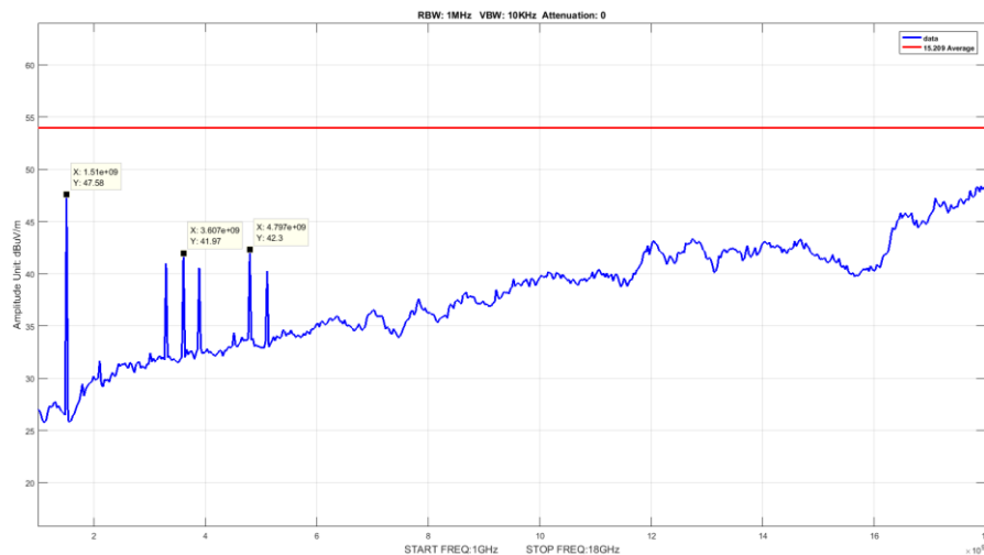
Plot 10. Radiated Emissions, 1 – 18 GHz, 410.5 MHz, Low Channel Average
