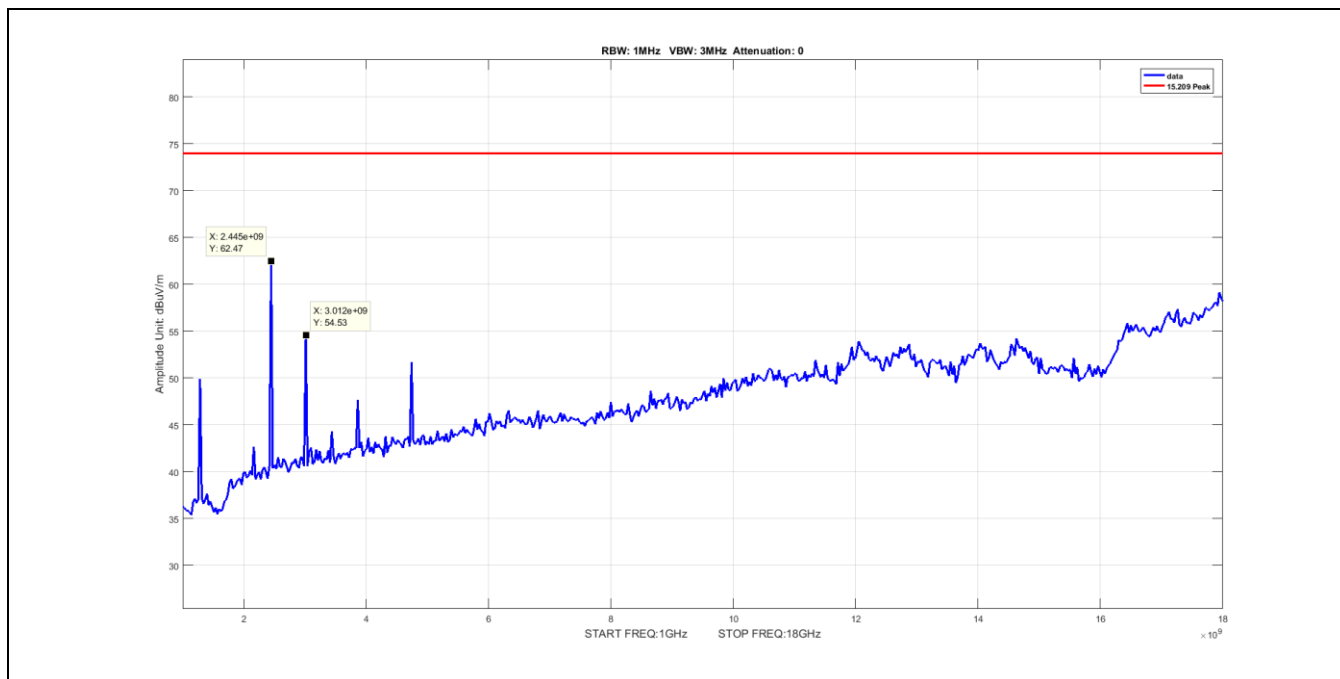
Plot 13. Radiated Emissions, 1 – 18 GHz, 430.25 MHz, Mid Channel Peak
