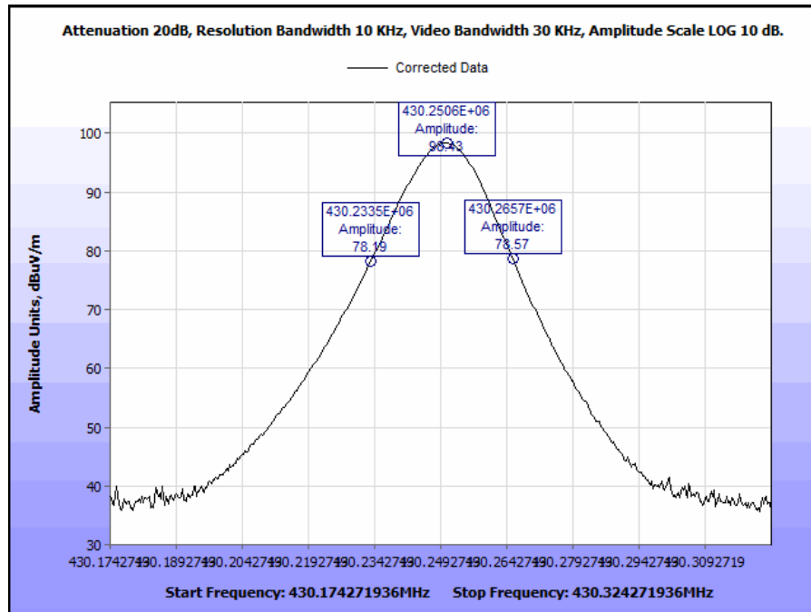
Plot 8. 20 dB Bandwidth Plot, 430.25 MHz Mid Channel
