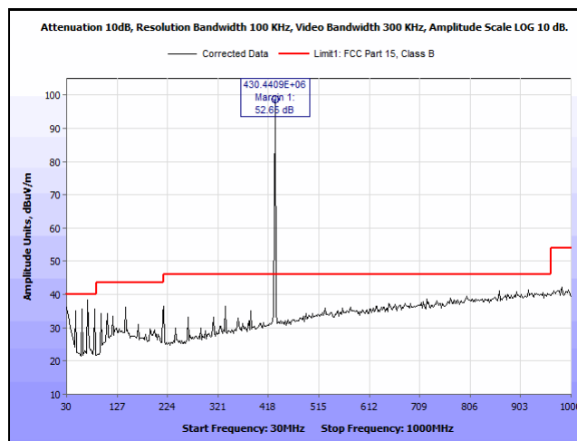
Plot 8. Radiated Emissions, 30 MHz – 1 GHz, 430.25 MHz, Mid Channel
