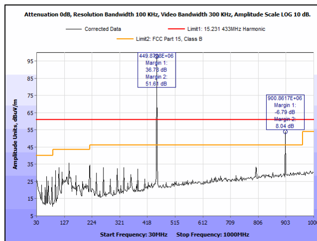
Plot 9. Radiated Emissions, 30 MHz – 1 GHz, 450 MHz, High Channel with 15.231 harmonics limit
