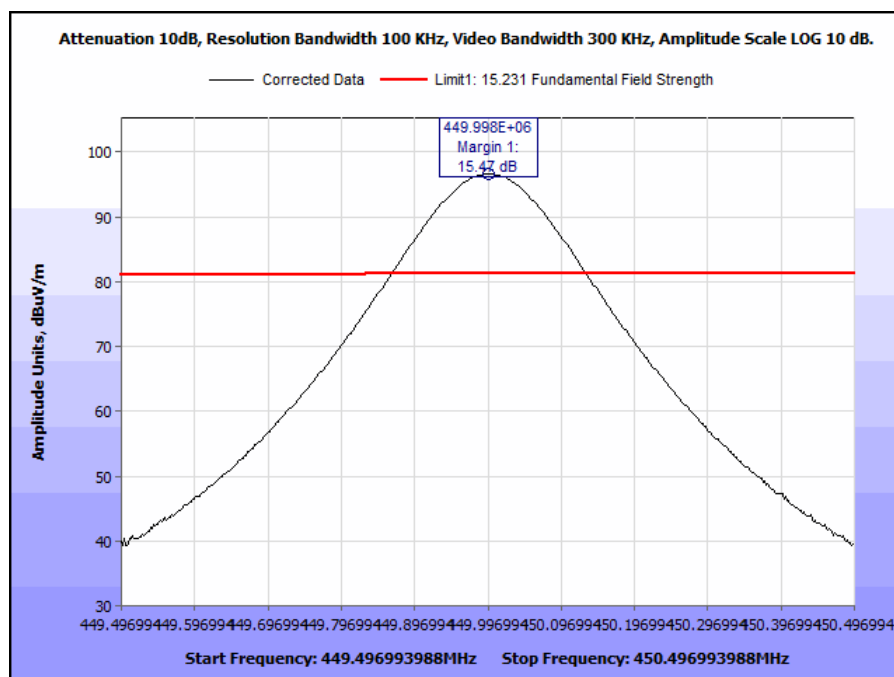
Plot 6. Field Strength of Fundamental, 450 MHz High Channel
