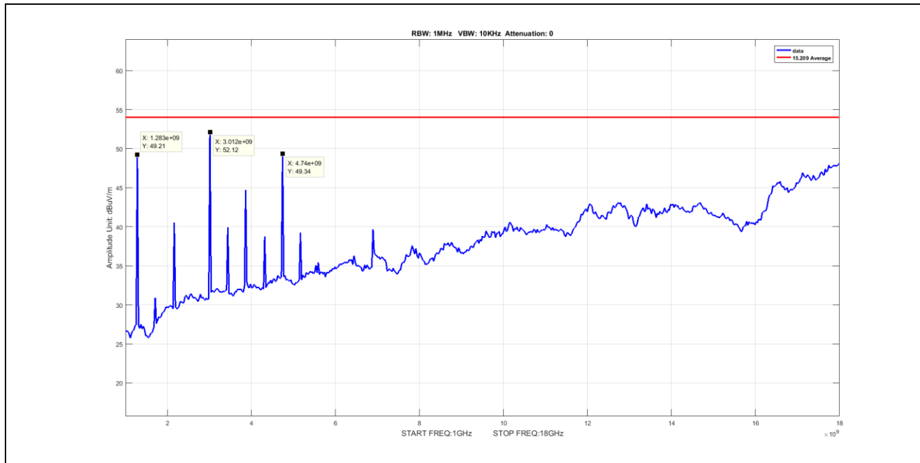
Plot 12. Radiated Emissions, 1 – 18 GHz, 430.25 MHz, Mid Channel Average
