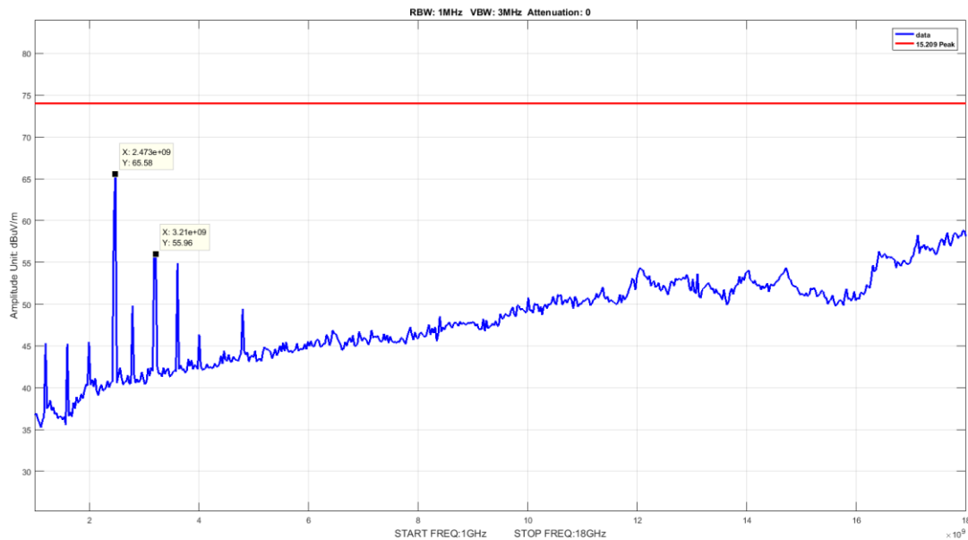
Plot 11. Radiated Emissions, 1 – 18 GHz, 410.5 MHz, Low Channel Peak
