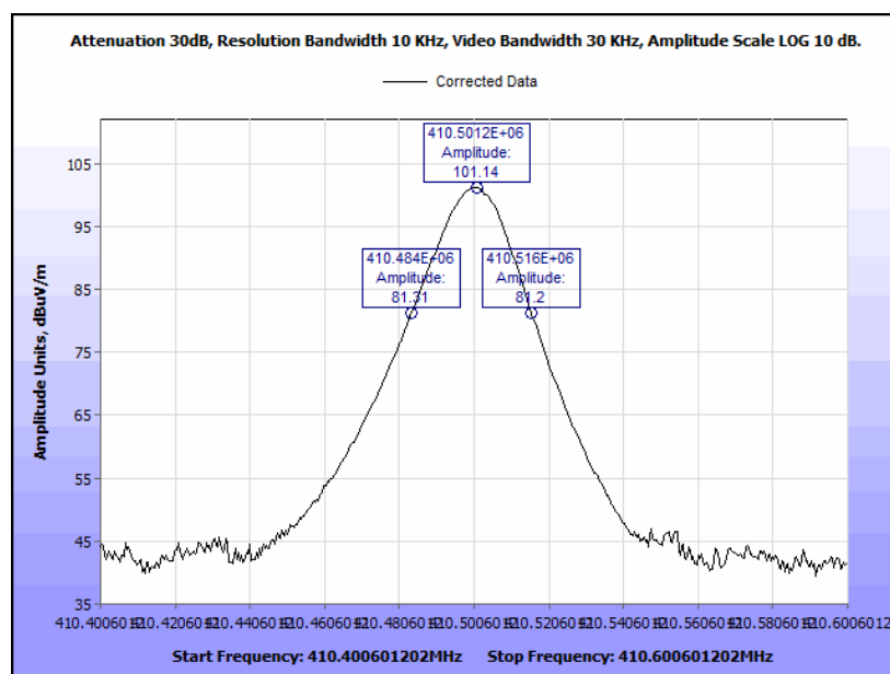
Plot 8. 20 dB Bandwidth Plot, 410.5 MHz Low Channel
