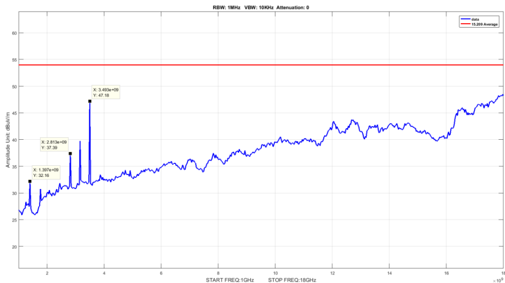
Plot 14. Radiated Emissions, 1 – 18 GHz, 450 MHz, High Channel Average
