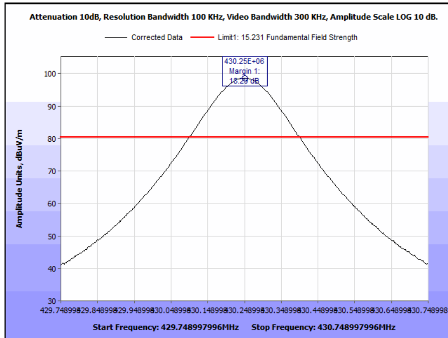
Plot 5. Field Strength of Fundamental, 430.25 MHz, Mid Channel
