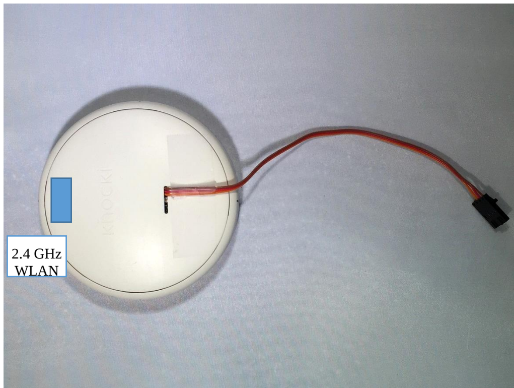
Photo 3: Antenna Location
