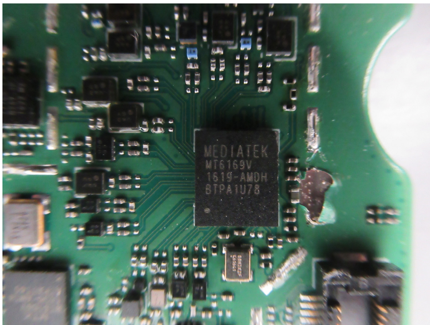
EUT – PCB-1 Chip View-9
