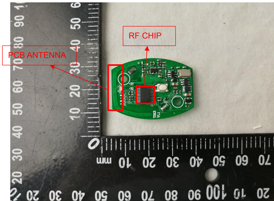
MAIN BOARD TOP VIEW 1
