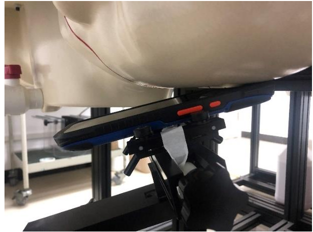
Left Tilted 15°
