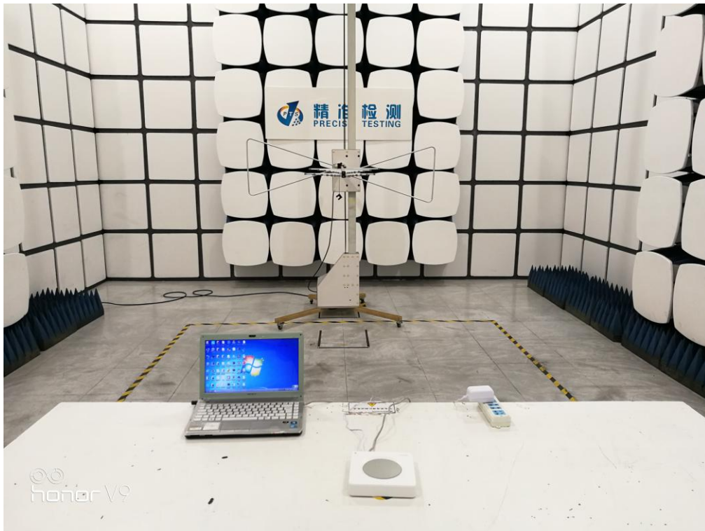
RADIATED EMISSION TEST SETUP BELOW 1GHz-CYY
