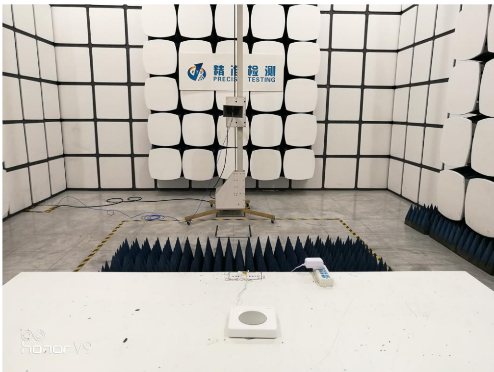
RADIATED EMISSION TEST SETUP ABOVE 1GHz-CYY
