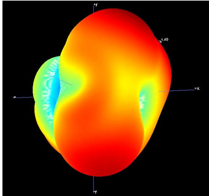
B1.1 3D Pattern for 2400MHz
