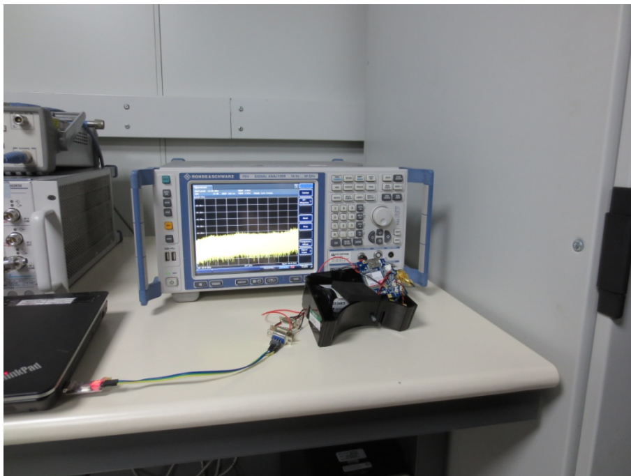
BLE RF Conducted Emissions Test setup
