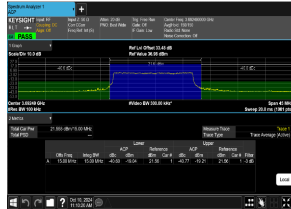
N48(15M)_DFT-s- OFDM_QPSK_Outer_Full_High_CH
