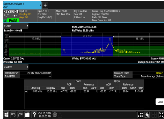
N48(15M)_DFT-s-OFDM_QPSK_Edge_1RB_Right_Low_CH
