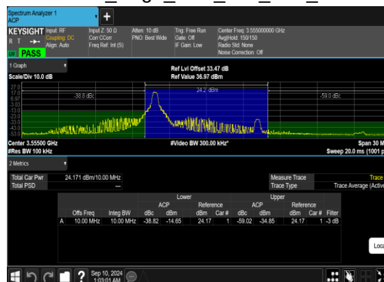
N48(10M)_DFT-s-OFDM_PI_2- BPSK_Edge_1RB_Left_Low_CH
