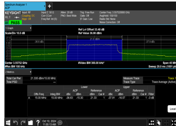
N48(15M)_DFT-s- OFDM_QPSK_Outer_Full_Low_CH
