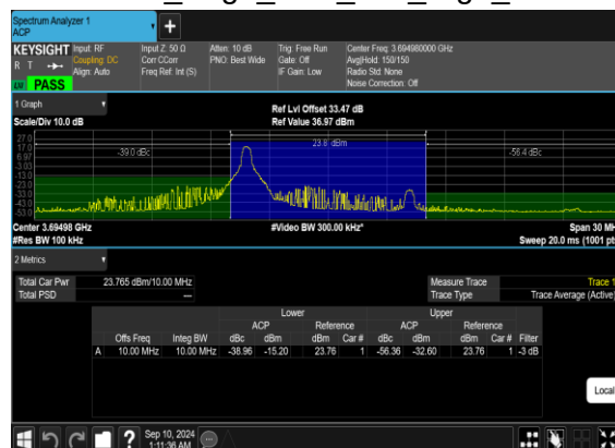
N48(10M)_DFT-s-OFDM_PI_2- BPSK_Edge_1RB_Left_High_CH
