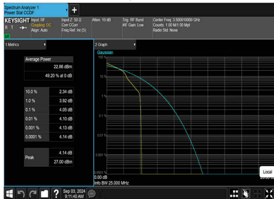
N77(20M)_DFT-s- OFDM_QPSK_Edge_1RB_Left_Mid_CH
