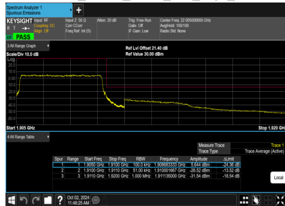
B5_N2(5M)_DFT-s- OFDM_QPSK_Outer_Full_High_CH
