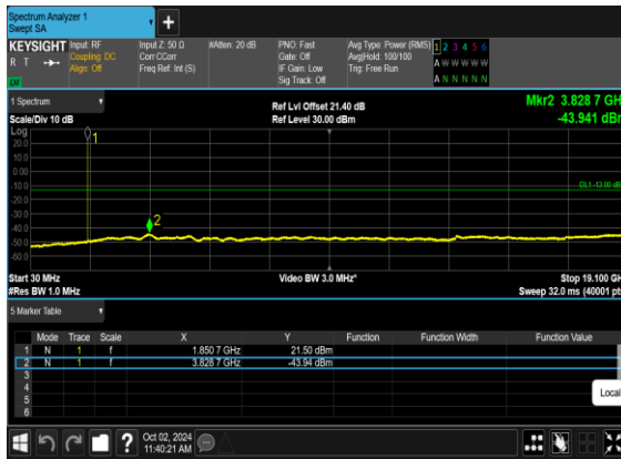
B5_N2(20M)_DFT-s- OFDM_BPSK_Edge_1RB_Left_Low_CH
