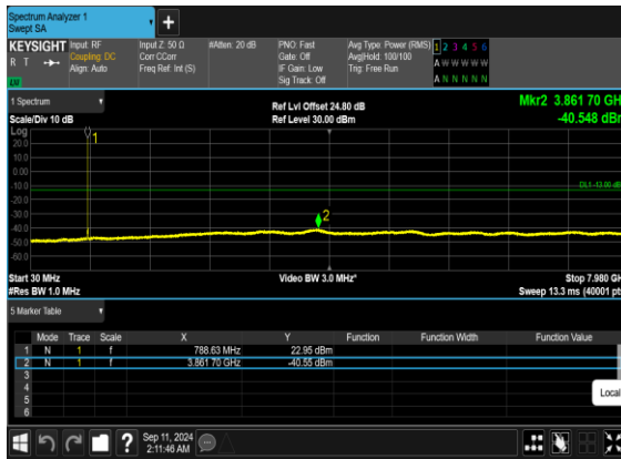
N14(5M)_DFT-s- OFDM_BPSK_Edge_1RB_Left_Low_CH
