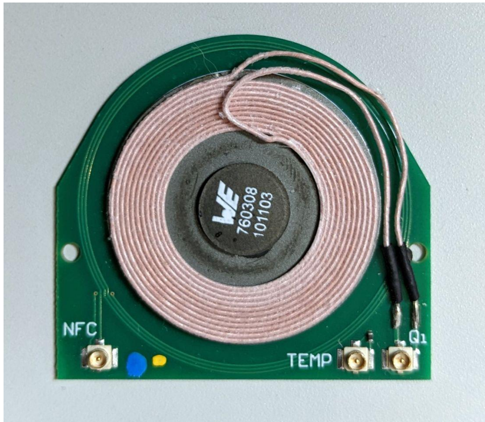
Antenna PCB
