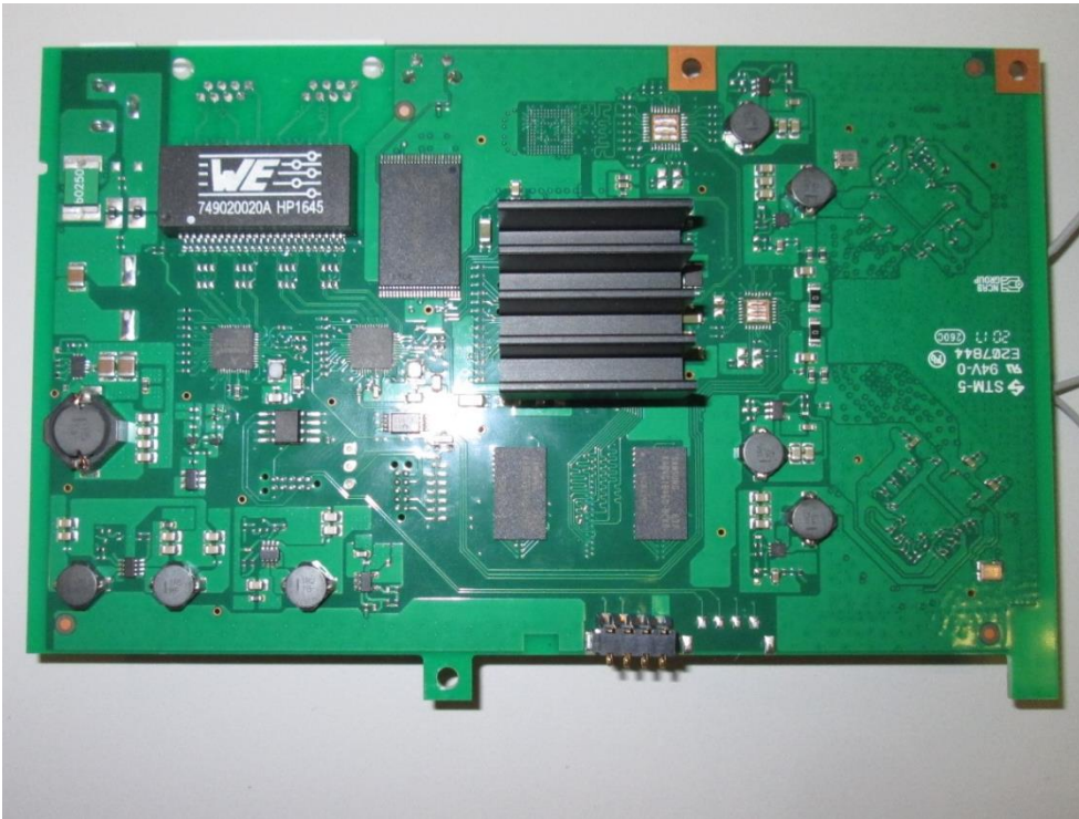
Photo A3-1: Main PCB, Top View
