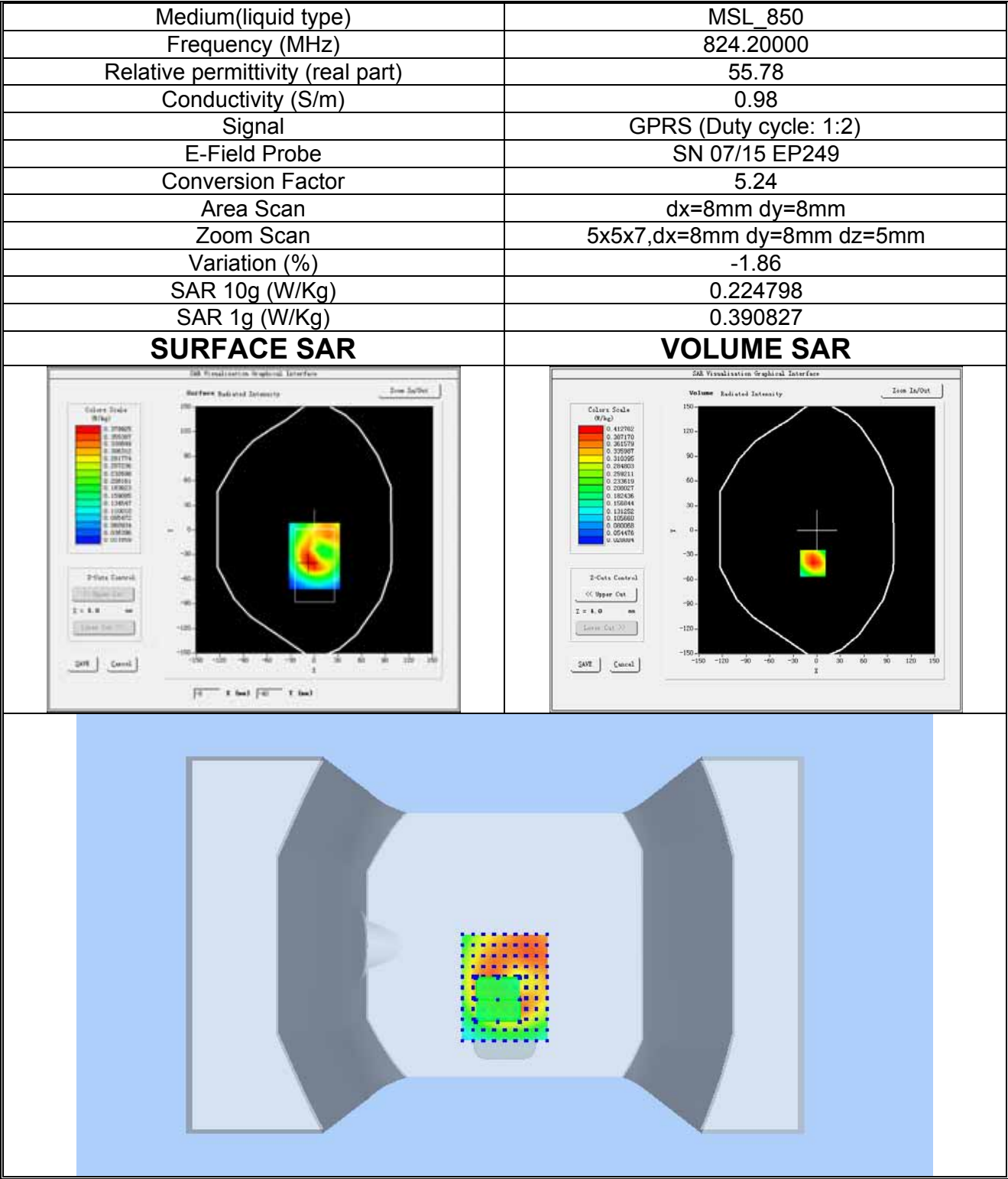
Plot 3: GPRS850MHz, Middle channel (Body-worn, Back Surface) Product Description: Smart Phone Test Date: 2018-06-25
