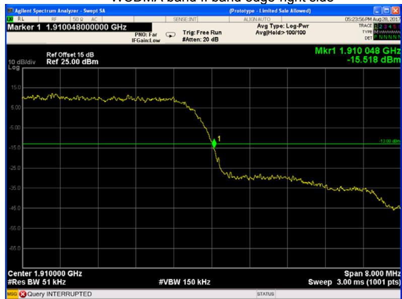
WCDMA band II band edge-right side
