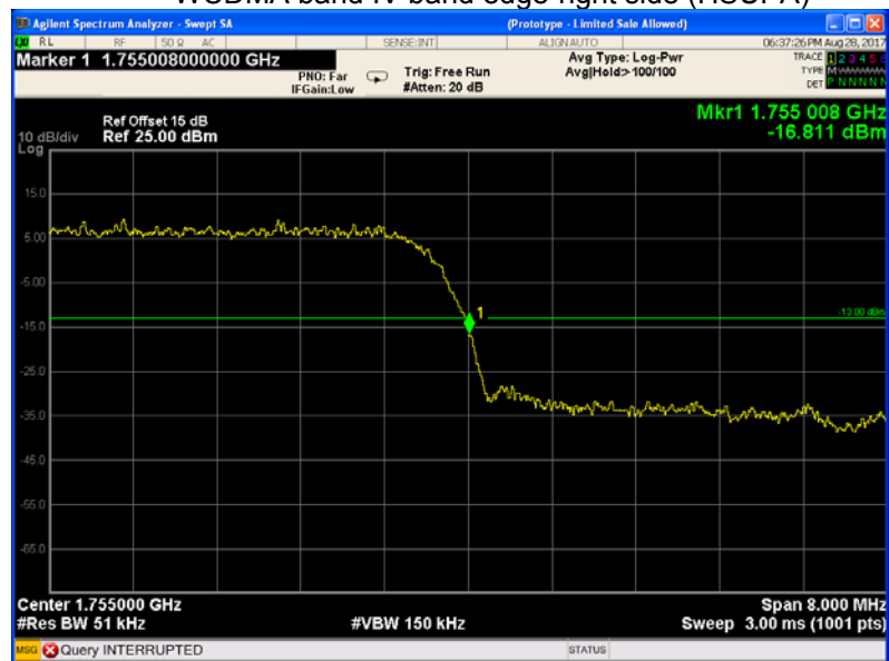
WCDMA band IV band edge-right side (HSUPA)
