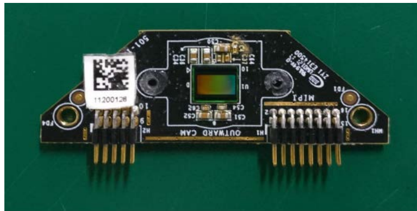
Outward PCB Top View
