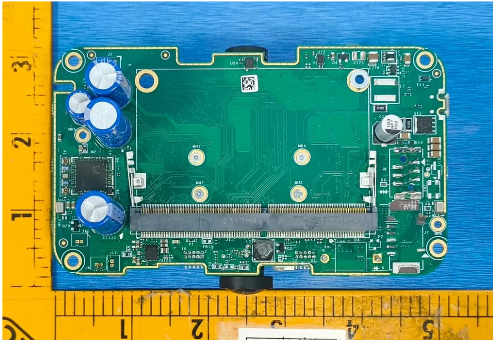
PCB Without Shielding Case
