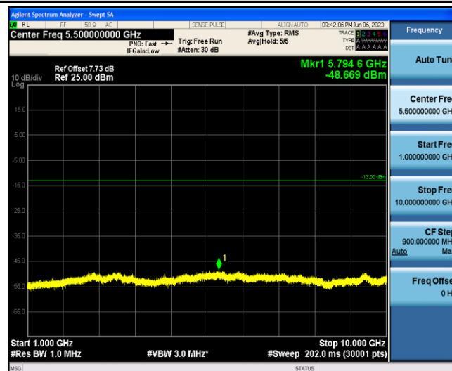
Band5-5MHz-16QAM-20425-1-0-Low-1000-10000--48.67-PASS
