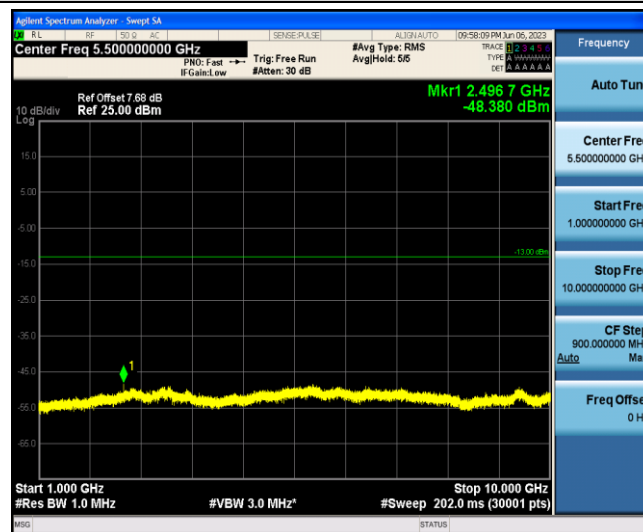
Band5-10MHz-QPSK-20525-1-0-Low-1000-10000--48.38-PASS
