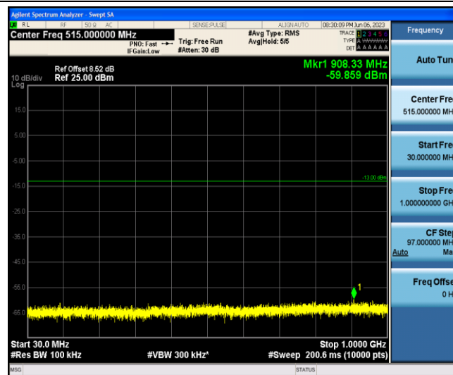
Band2-15MHz-16QAM-19125-1-0-Low-30-1000--59.86-PASS
