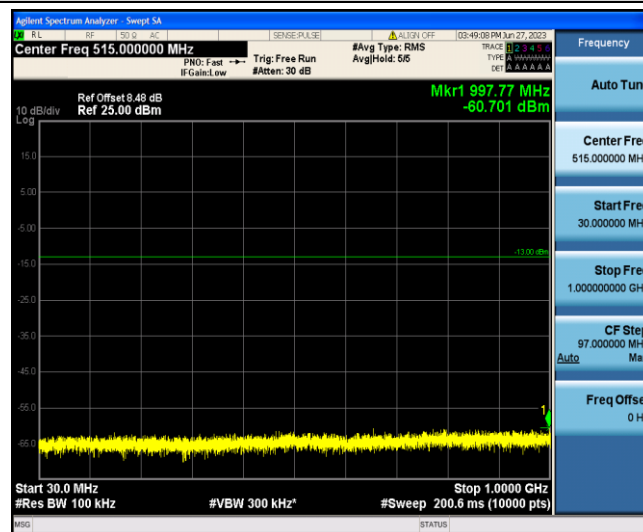
Band4-3MHz-16QAM-20385-1-0-Low-30-1000--60.7-PASS
