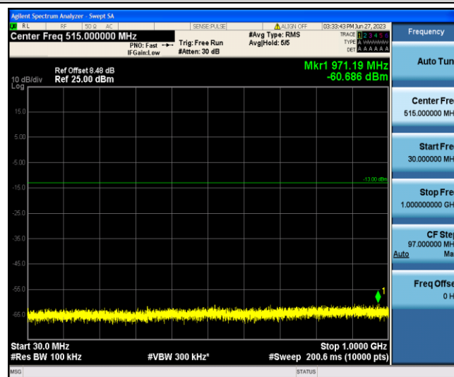
Band4-1.4MHz-QPSK-20393-1-0-Low-30-1000--60.69-PASS
