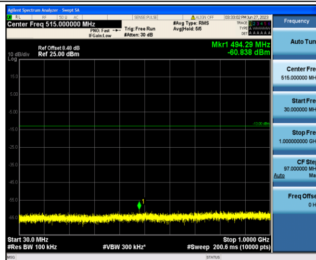
Band4-1.4MHz-QPSK-20175-1-0-Low-30-1000--60.84-PASS
