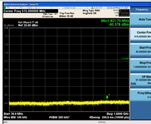
Band4-1.4MHz-16QAM-19957-1-0-Low-30-1000--60.38-PASS
