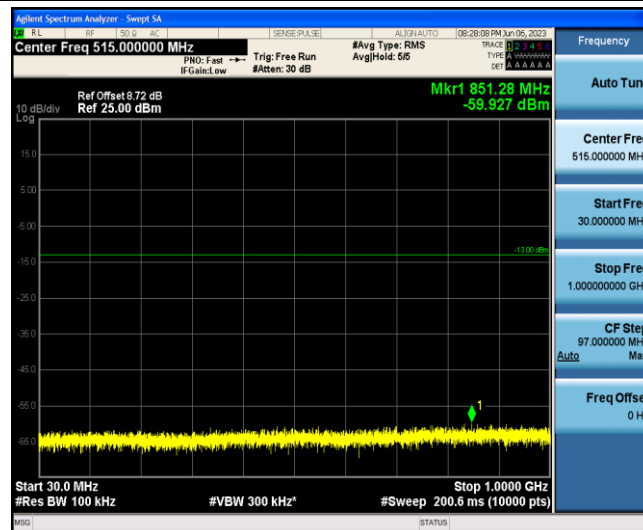
Band2-15MHz-16QAM-18675-1-0-Low-30-1000--59.93-PASS
