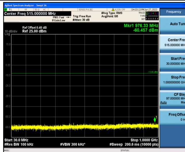
Band4-5MHz-QPSK-20175-1-0-Low-30-1000--60.46-PASS
