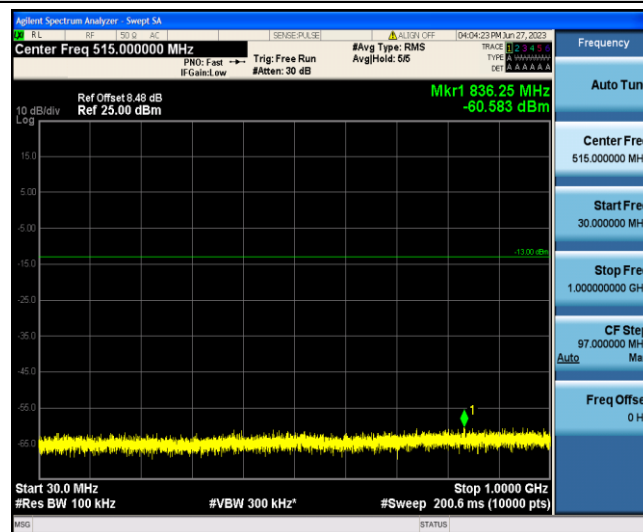
Band4-5MHz-16QAM-20375-1-0-Low-30-1000--60.58-PASS
