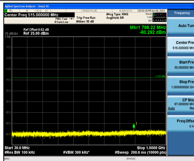
Band2-20MHz-16QAM-19100-1-0-Low-30-1000--60.29-PASS
