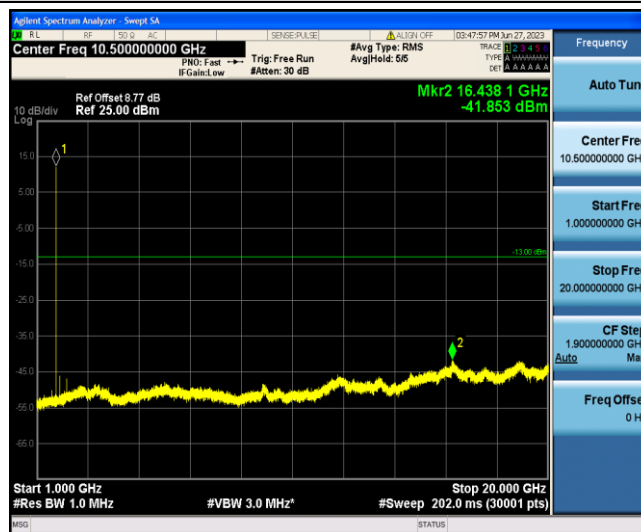
Band4-3MHz-16QAM-19965-1-0-Low-1000-20000--41.85-PASS
