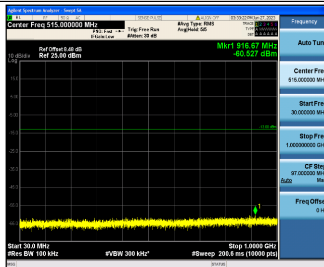
Band4-1.4MHz-16QAM-20175-1-0-Low-30-1000--60.53-PASS
