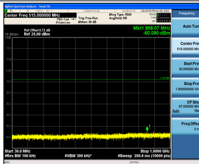
Band2-15MHz-16QAM-18900-1-0-Low-30-1000--60.09-PASS
