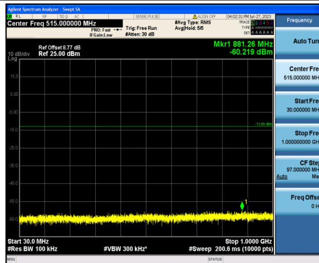
Band4-5MHz-QPSK-19975-1-0-Low-30-1000--60.22-PASS
