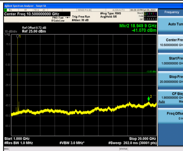
Band2-15MHz-16QAM-18675-1-0-Low-1000-20000--41.07-PASS
