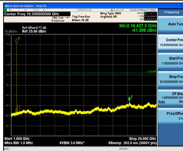
Band4-1.4MHz-16QAM-19957-1-0-Low-1000-20000--41.3-PASS
