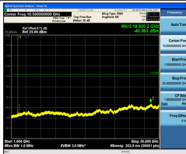
Band2-20MHz-QPSK-18700-1-0-Low-1000-20000--40.96-PASS
