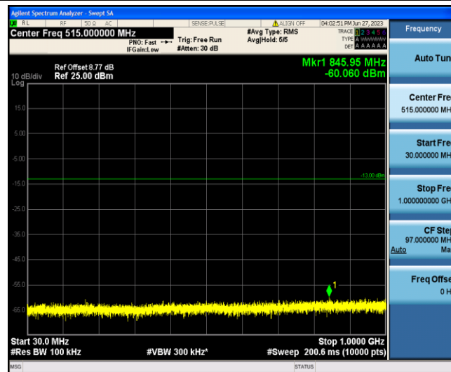
Band4-5MHz-16QAM-19975-1-0-Low-30-1000--60.06-PASS
