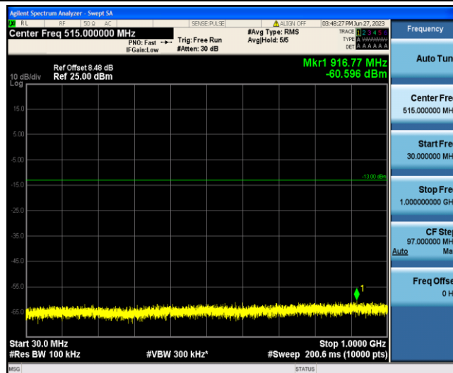
Band4-3MHz-16QAM-20175-1-0-Low-30-1000--60.6-PASS
