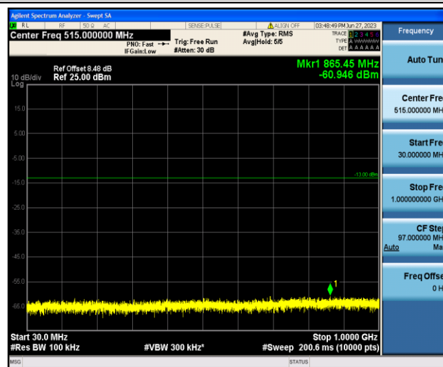
Band4-3MHz-QPSK-20385-1-0-Low-30-1000--60.95-PASS
