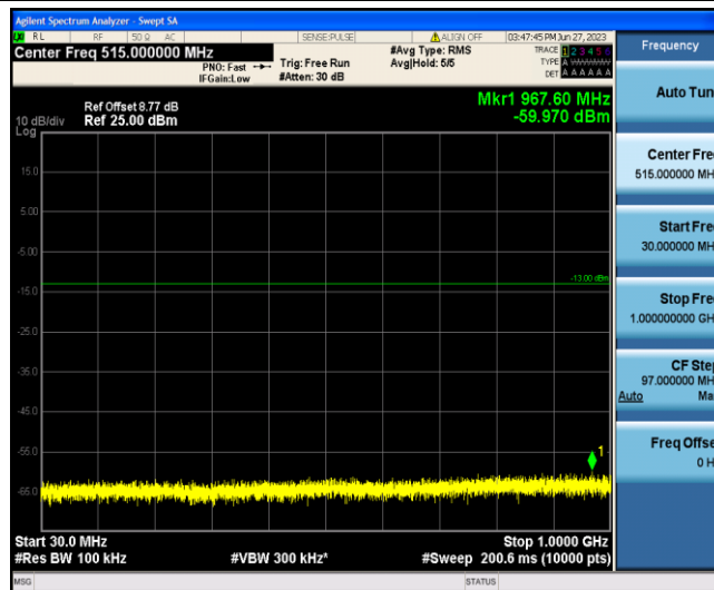
Band4-3MHz-16QAM-19965-1-0-Low-30-1000--59.97-PASS
