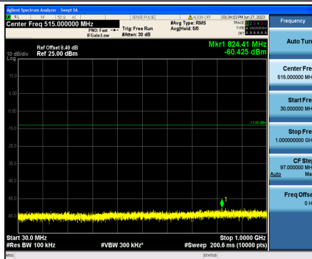
Band4-1.4MHz-16QAM-20393-1-0-Low-30-1000--60.43-PASS
