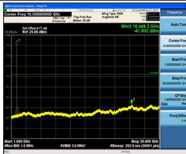
Band4-1.4MHz-QPSK-19957-1-0-Low-1000-20000--41.83-PASS
