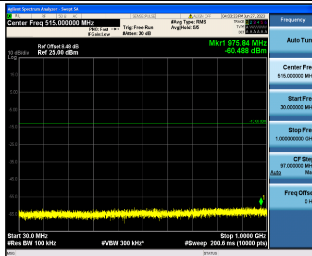
Band4-5MHz-16QAM-20175-1-0-Low-30-1000--60.49-PASS
