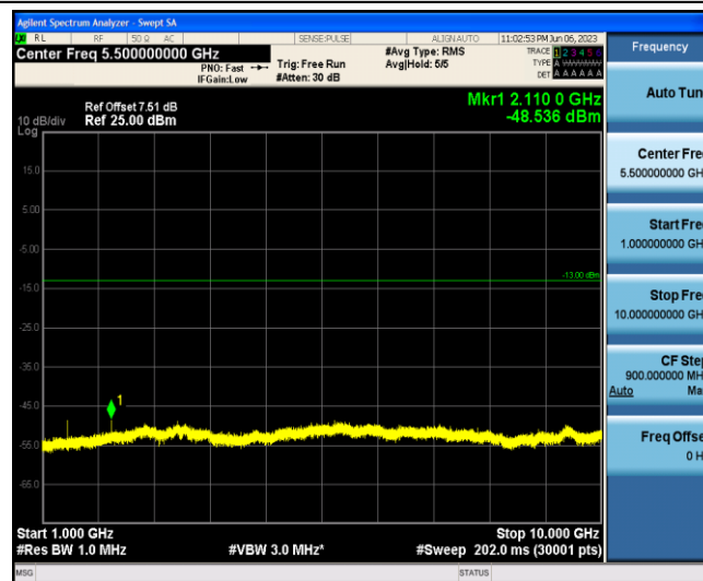
Band12-10MHz-QPSK-23095-1-0-Low-1000-10000--48.54-PASS
