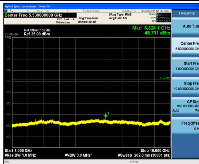
Band13-5MHz-QPSK-23205-1-0-Low-1000-10000--48.7-PASS
