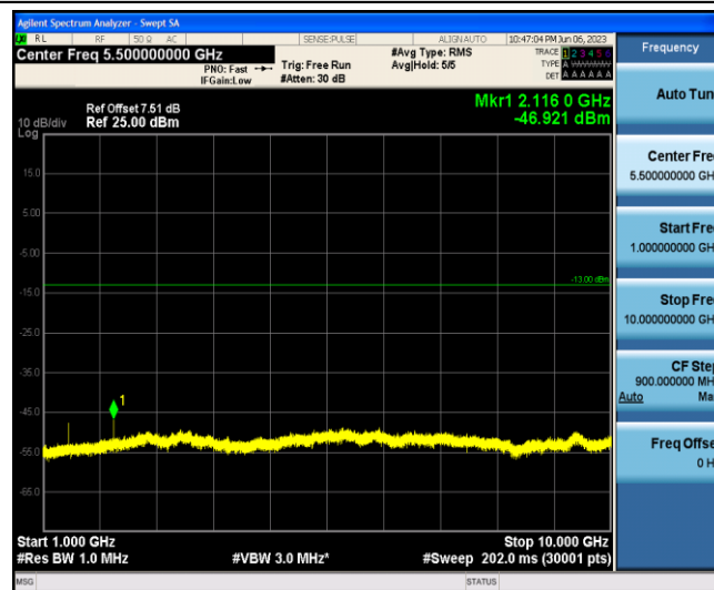
Band12-5MHz-QPSK-23095-1-0-Low-1000-10000--46.92-PASS
