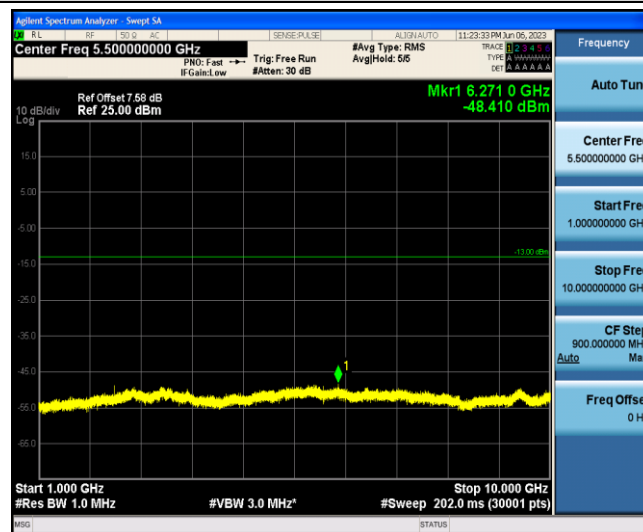
Band13-5MHz-16QAM-23205-1-0-Low-1000-10000--48.41-PASS
