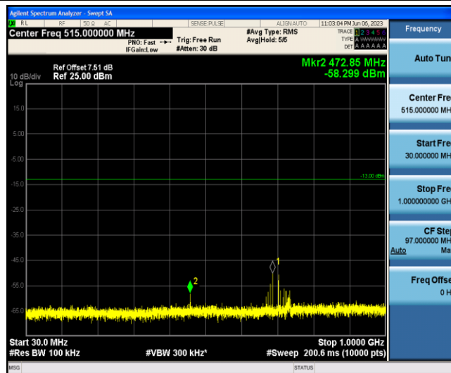
Band12-10MHz-16QAM-23095-1-0-Low-30-1000--58.3-PASS
