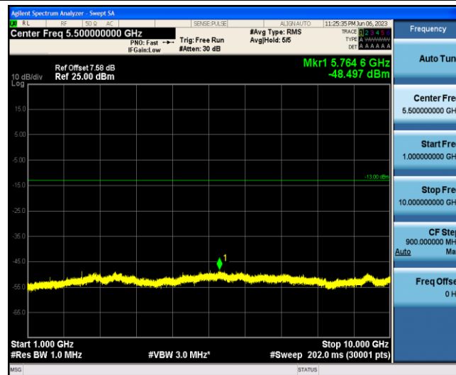
Band13-5MHz-16QAM-23255-1-0-Low-1000-10000--48.5-PASS
