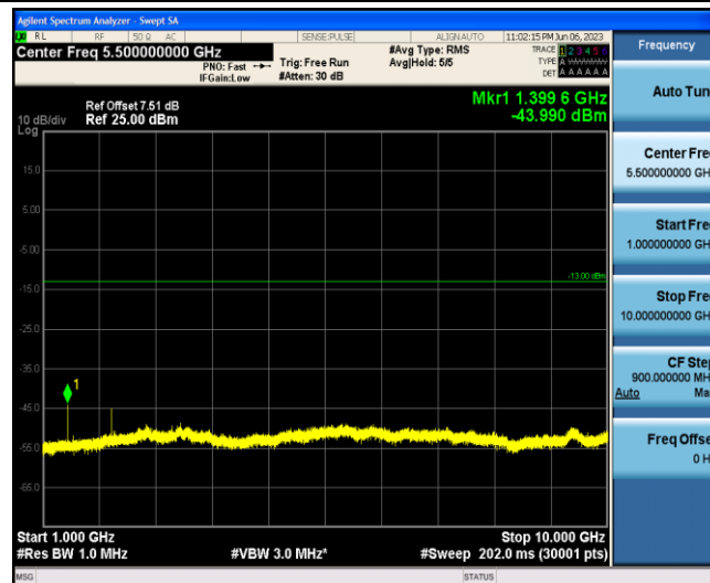
Band12-10MHz-QPSK-23060-1-0-Low-1000-10000--43.99-PASS
