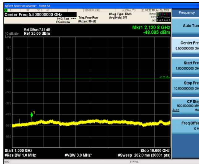
Band12-10MHz-QPSK-23130-1-0-Low-1000-10000--48.1-PASS
