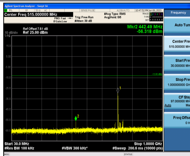
Band12-5MHz-16QAM-23155-1-0-Low-30-1000--56.32-PASS
