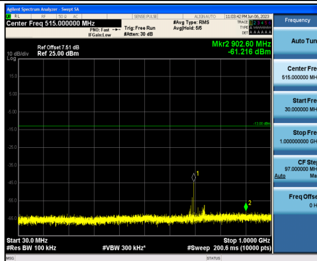
Band12-10MHz-16QAM-23130-1-0-Low-30-1000--61.22-PASS
