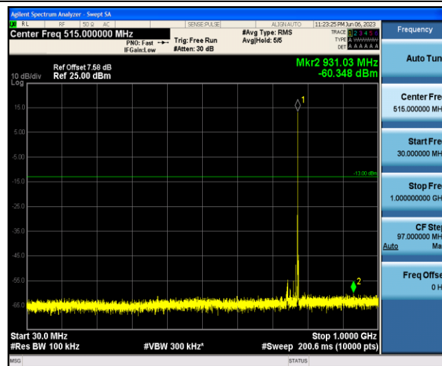
Band13-5MHz-16QAM-23205-1-0-Low-30-1000--60.35-PASS
