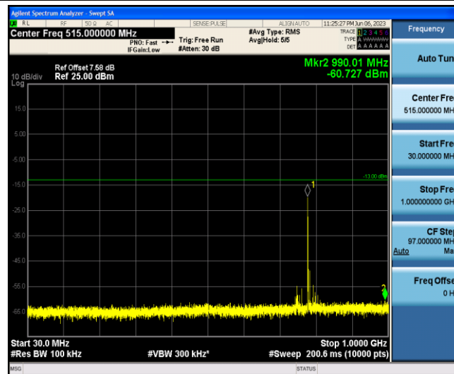
Band13-5MHz-16QAM-23255-1-0-Low-30-1000--60.73-PASS
