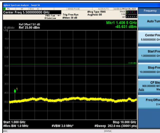
Band12-10MHz-16QAM-23095-1-0-Low-1000-10000--45.63-PASS
