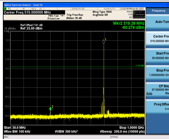
Band12-10MHz-QPSK-23095-1-0-Low-30-1000--60.28-PASS
