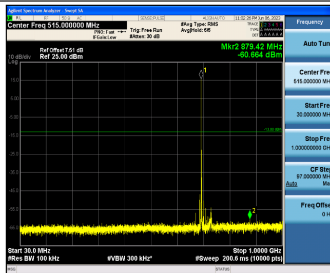
Band12-10MHz-16QAM-23060-1-0-Low-30-1000--60.66-PASS
