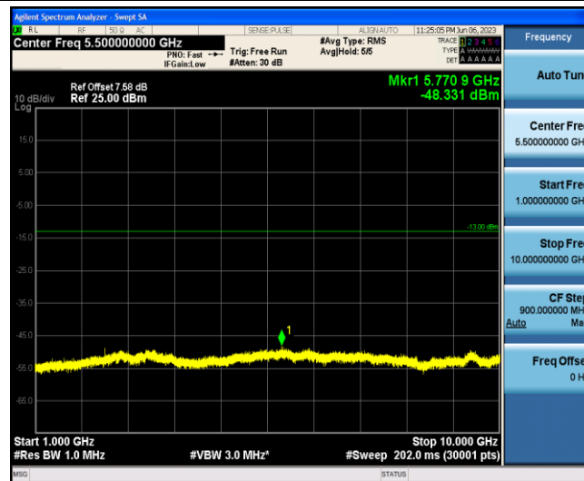
Band13-5MHz-QPSK-23255-1-0-Low-1000-10000--48.33-PASS
