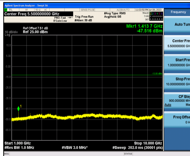
Band12-10MHz-16QAM-23130-1-0-Low-1000-10000--47.52-PASS
