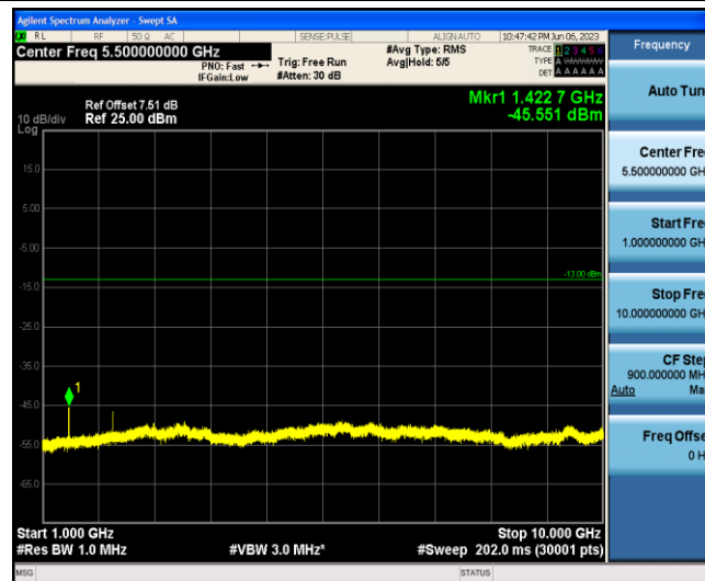
Band12-5MHz-QPSK-23155-1-0-Low-1000-10000--45.55-PASS
