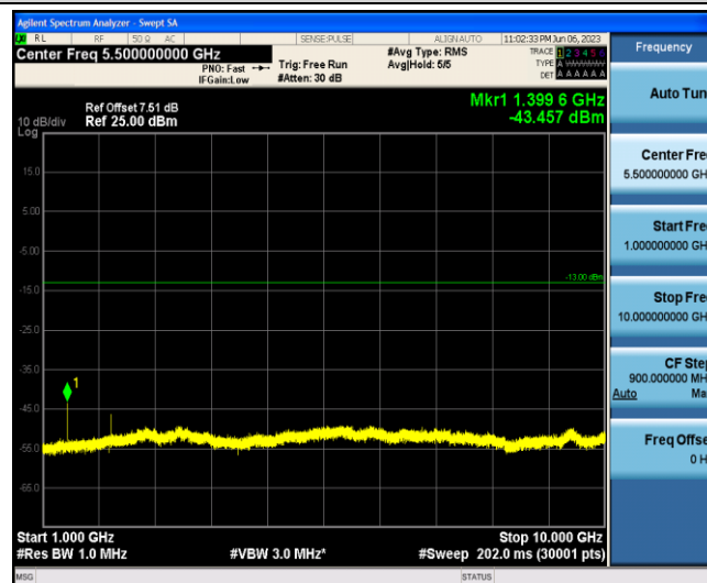
Band12-10MHz-16QAM-23060-1-0-Low-1000-10000--43.46-PASS
