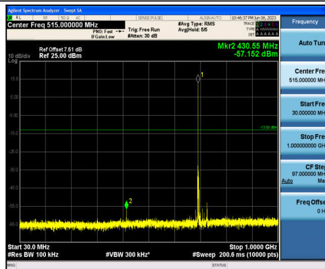
Band12-5MHz-16QAM-23035-1-0-Low-30-1000--57.15-PASS
