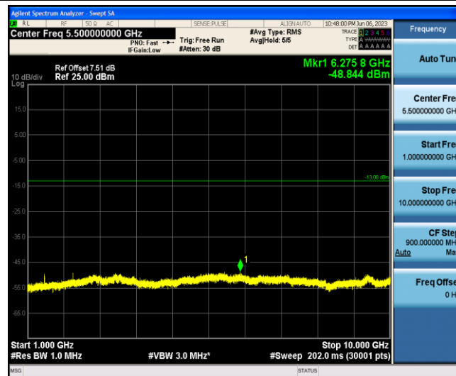
Band12-5MHz-16QAM-23155-1-0-Low-1000-10000--48.84-PASS
