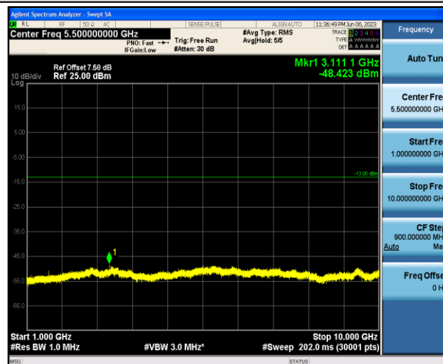
Band13-10MHz-16QAM-23230-1-0-Low-1000-10000--48.42-PASS
