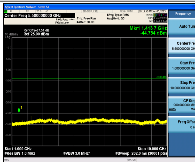
Band12-1.4MHz-QPSK-23095-1-0-Low-1000-10000--44.75-PASS
