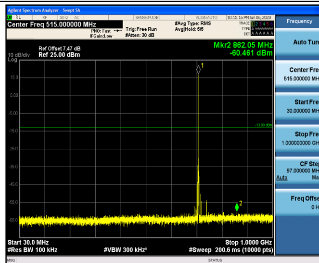
Band12-1.4MHz-QPSK-23173-1-0-Low-30-1000--60.46-PASS
