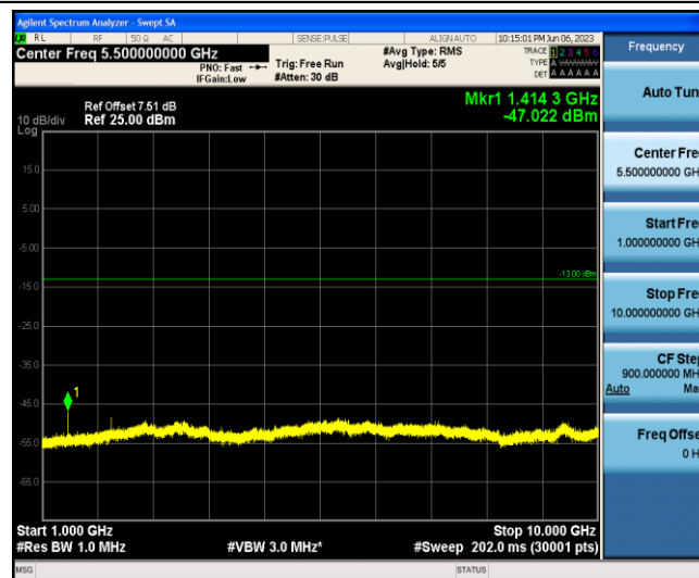
Band12-1.4MHz-16QAM-23095-1-0-Low-1000-10000--47.02-PASS
