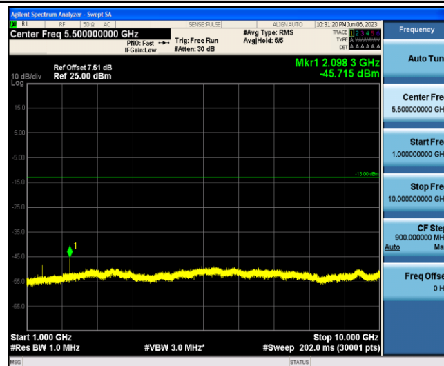
Band12-3MHz-16QAM-23025-1-0-Low-1000-10000--45.72-PASS
