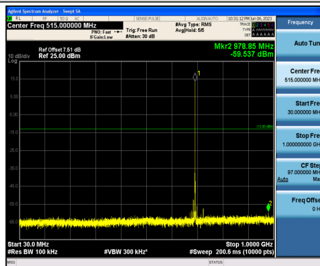
Band12-3MHz-16QAM-23025-1-0-Low-30-1000--59.54-PASS
