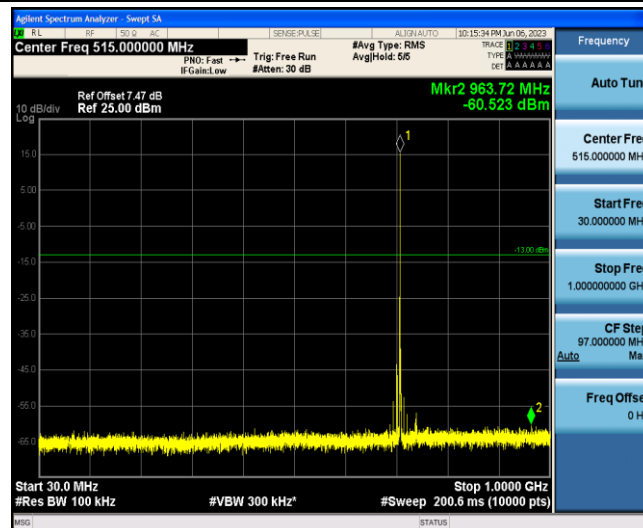
Band12-1.4MHz-16QAM-23173-1-0-Low-30-1000--60.52-PASS
