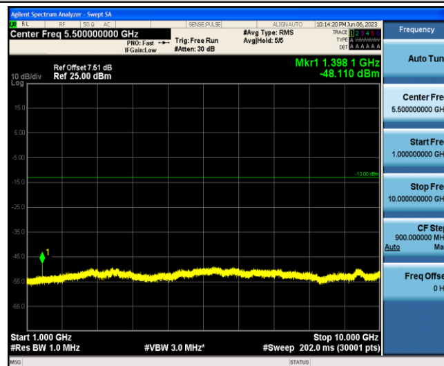
Band12-1.4MHz-16QAM-23017-1-0-Low-1000-10000--48.11-PASS
