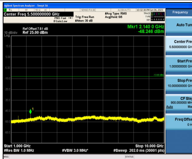
Band12-3MHz-16QAM-23165-1-0-Low-1000-10000--48.25-PASS
