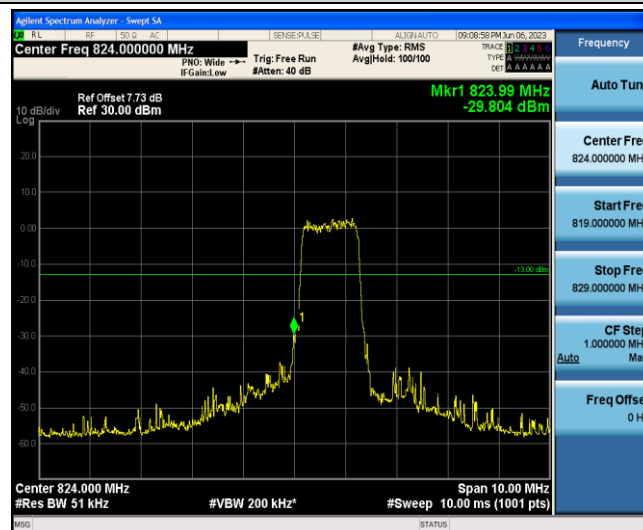
Band5-1.4MHz-16QAM-20407-6-0-Low--29.80-PASS
