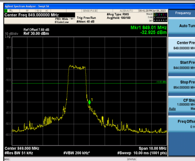
Band5-5MHz-16QAM-20625-6-0-High--32.93-PASS
