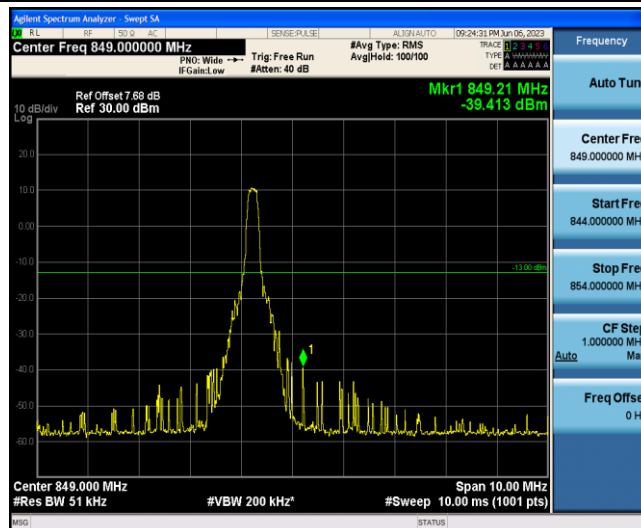
Band5-3MHz-16QAM-20635-1-5-High--39.41-PASS
