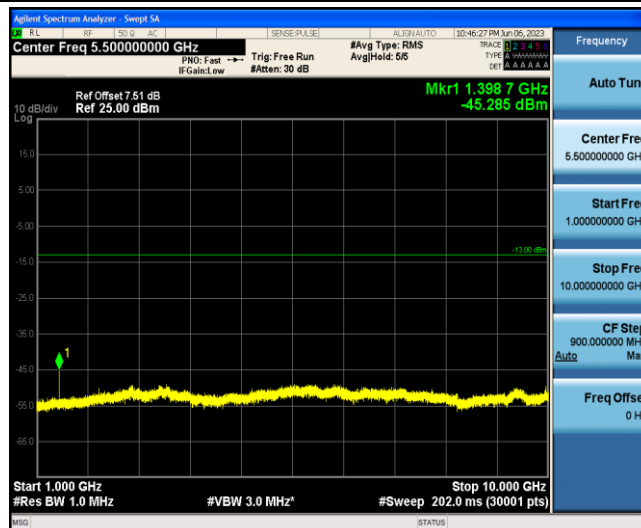
Band12-5MHz-QPSK-23035-1-0-Low-1000-10000--45.29-PASS
