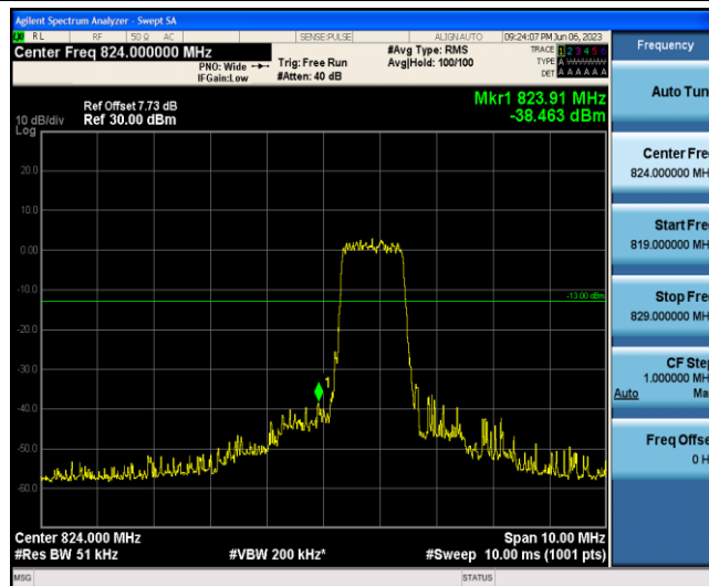
Band5-3MHz-16QAM-20415-6-0-Low--38.46-PASS
