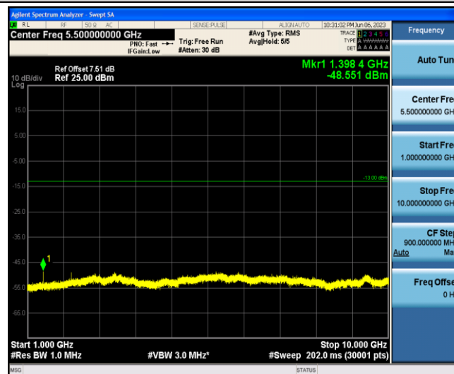
Band12-3MHz-QPSK-23025-1-0-Low-1000-10000--48.55-PASS
