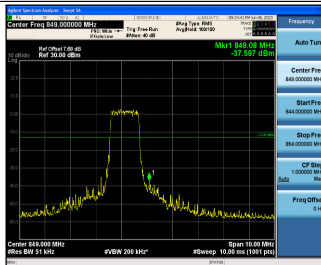
Band5-3MHz-QPSK-20635-6-0-High--37.60-PASS
