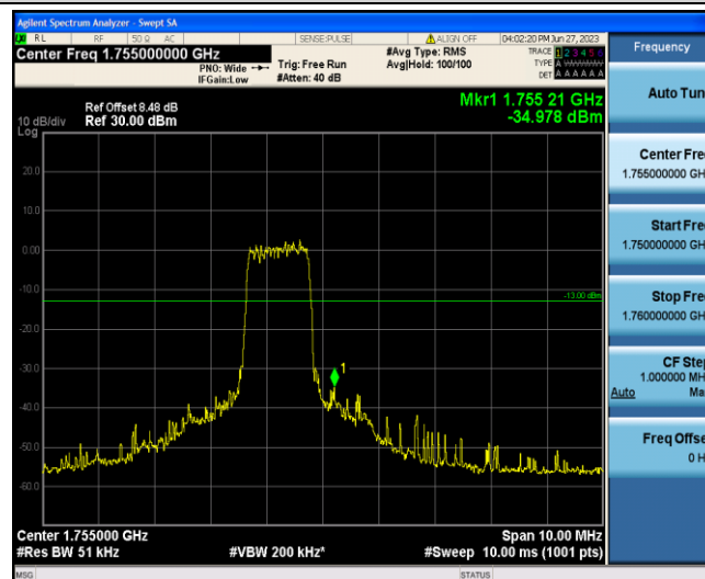
Band4-5MHz-16QAM-20375-6-0-High--34.98-PASS
