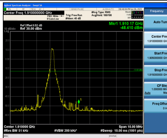
Band2-20MHz-16QAM-19100-1-5-High--48.41-PASS
