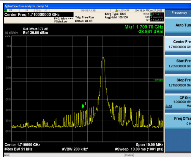
Band4-15MHz-QPSK-20025-1-0-Low--38.96-PASS
