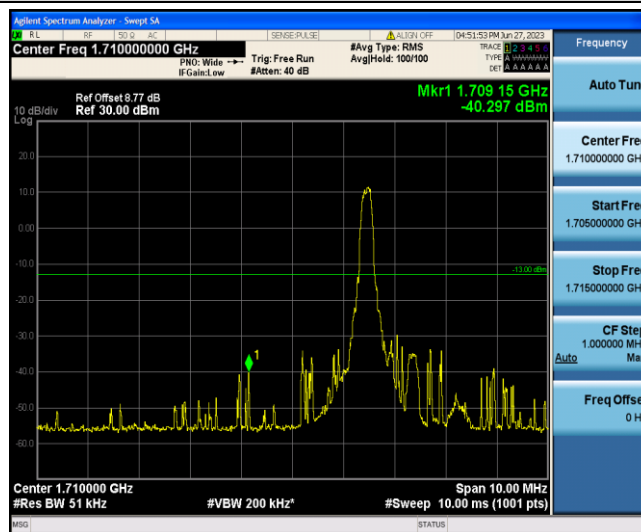
Band4-20MHz-QPSK-20050-1-0-Low--40.30-PASS
