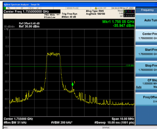
Band4-15MHz-QPSK-20325-6-0-High--35.95-PASS
