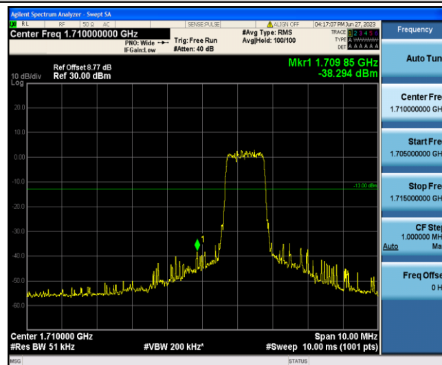
Band4-10MHz-16QAM-20000-6-0-Low--38.29-PASS
