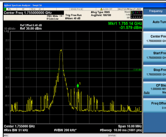
Band4-10MHz-QPSK-20350-1-5-High--31.58-PASS
