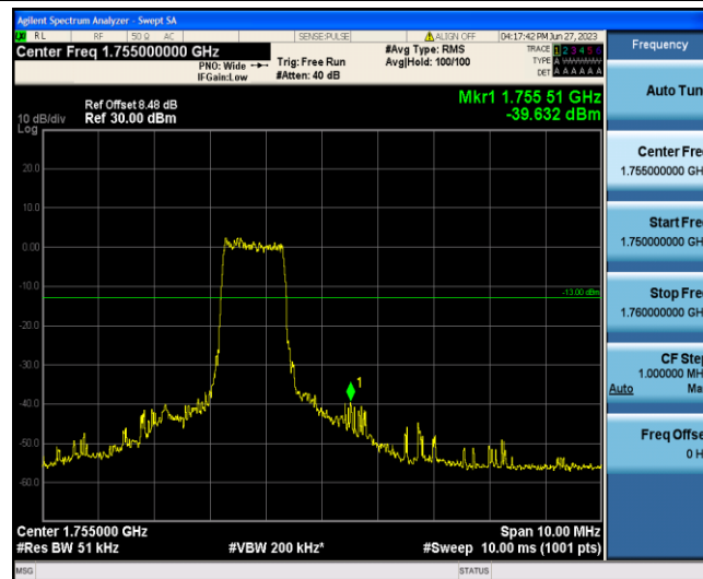
Band4-10MHz-QPSK-20350-6-0-High--39.63-PASS
