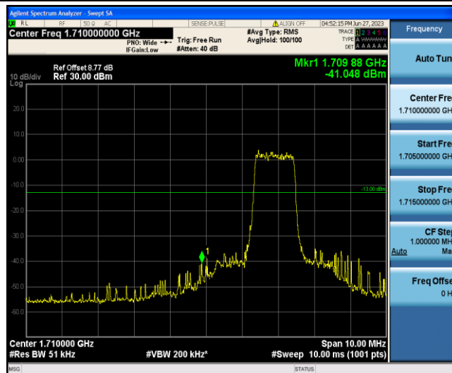
Band4-20MHz-QPSK-20050-6-0-Low--41.05-PASS
