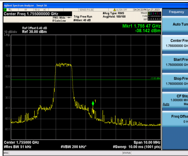
Band4-15MHz-16QAM-20325-6-0-High--38.14-PASS
