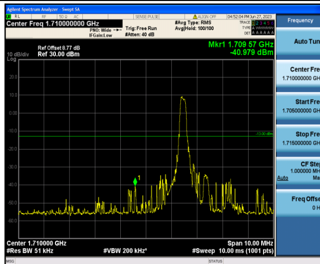
Band4-20MHz-16QAM-20050-1-0-Low--40.98-PASS
