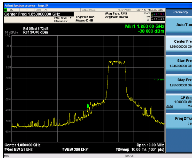
Band2-20MHz-16QAM-18700-6-0-Low--38.88-PASS
