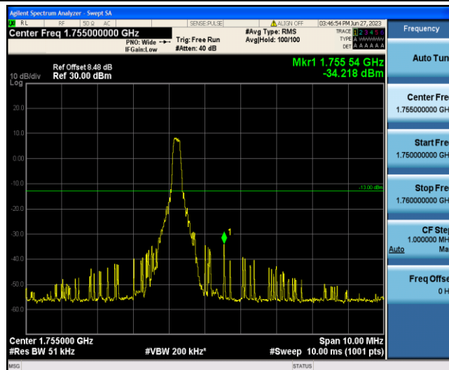
Band4-3MHz-16QAM-20385-1-5-High--34.22-PASS
