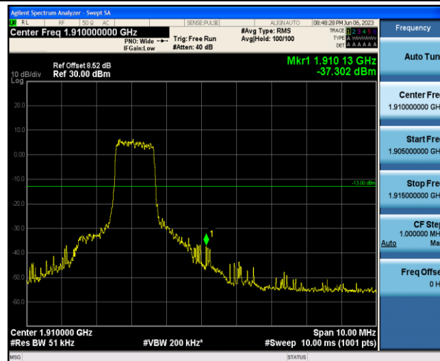
Band2-20MHz-16QAM-19100-6-0-High--37.30-PASS
