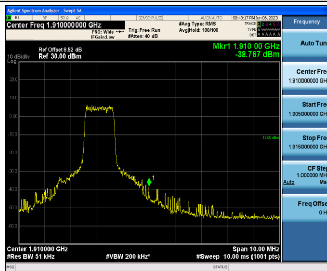
Band2-20MHz-QPSK-19100-6-0-High--38.77-PASS
