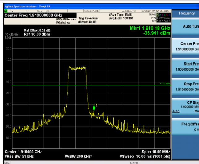
Band2-3MHz-QPSK-19185-6-0-High--35.94-PASS
