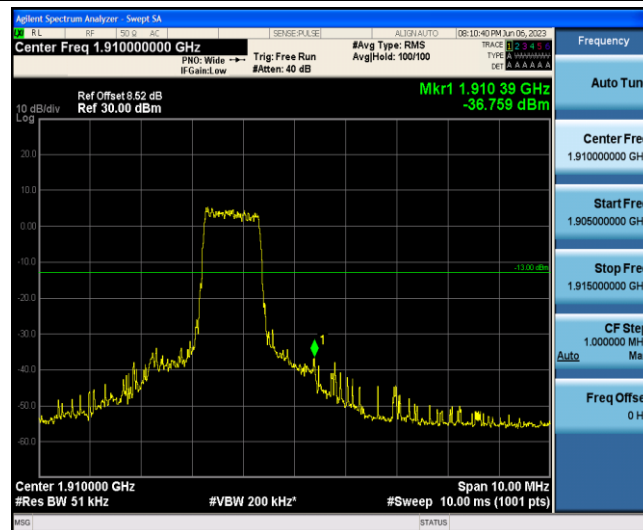
Band2-10MHz-QPSK-19150-6-0-High--36.76-PASS
