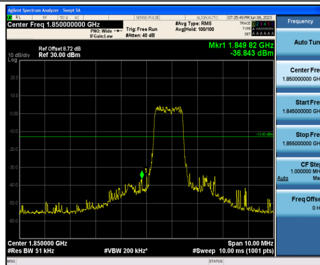
Band2-3MHz-16QAM-18615-6-0-Low--36.84-PASS
