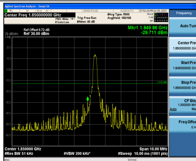
Band2-5MHz-16QAM-18625-1-0-Low--29.71-PASS
