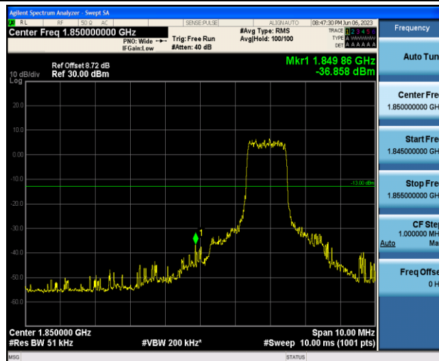
Band2-20MHz-QPSK-18700-6-0-Low--36.86-PASS
