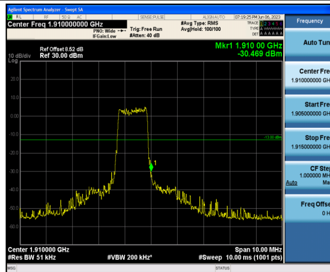
Band2-1.4MHz-QPSK-19193-6-0-High--30.47-PASS
