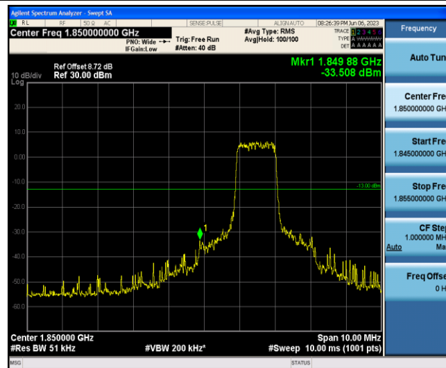
Band2-15MHz-QPSK-18675-6-0-Low--33.51-PASS
