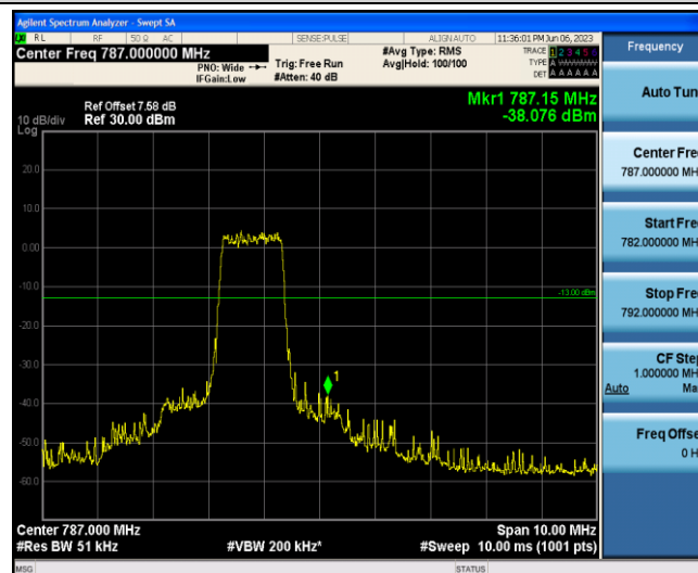
Band13-10MHz-16QAM-23230-6-0-High--38.08-PASS
