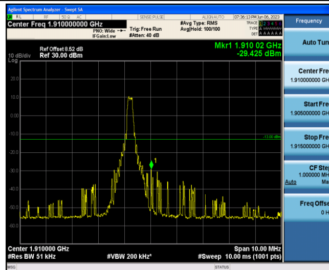
Band2-3MHz-16QAM-19185-1-5-High--29.42-PASS
