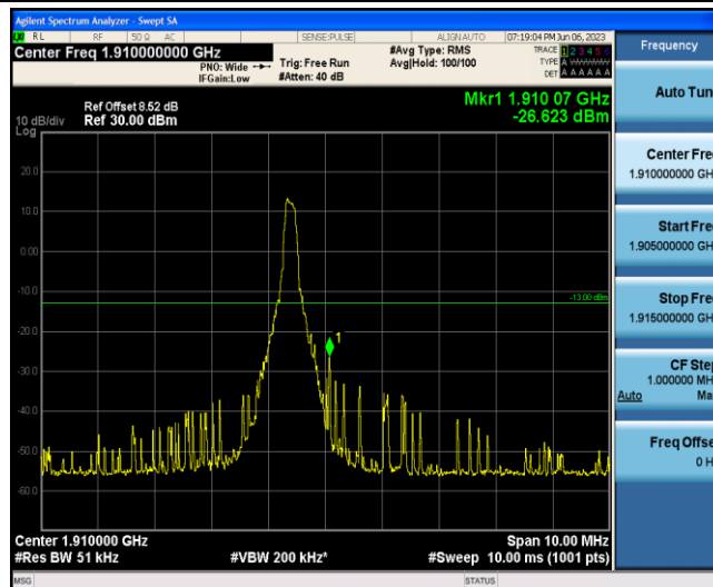
Band2-1.4MHz-QPSK-19193-1-5-High--26.62-PASS
