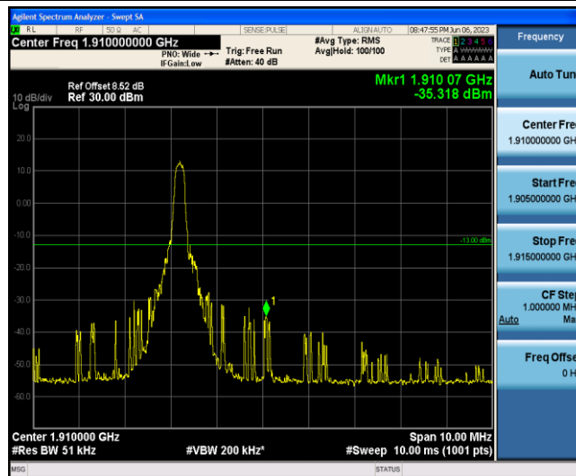
Band2-20MHz-QPSK-19100-1-5-High--35.32-PASS
