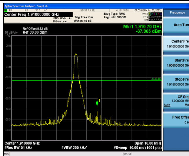
Band2-5MHz-16QAM-19175-1-5-High--37.06-PASS
