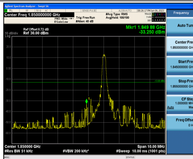
Band2-15MHz-QPSK-18675-1-0-Low--33.25-PASS
