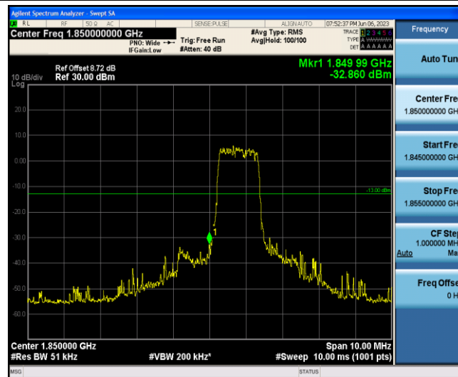
Band2-5MHz-16QAM-18625-6-0-Low--32.86-PASS
