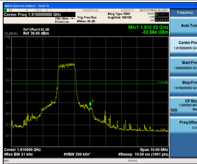
Band2-15MHz-16QAM-19125-6-0-High--33.68-PASS
