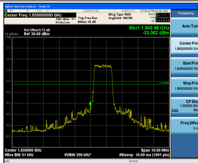
Band2-5MHz-QPSK-18625-6-0-Low--33.06-PASS
