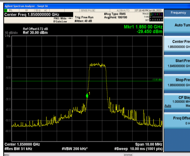
Band2-1.4MHz-16QAM-18607-6-0-Low--29.45-PASS
