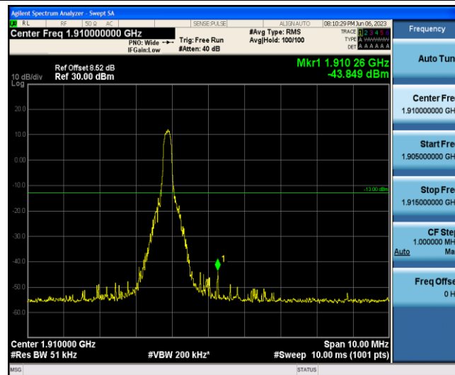
Band2-10MHz-16QAM-19150-1-5-High--43.85-PASS
