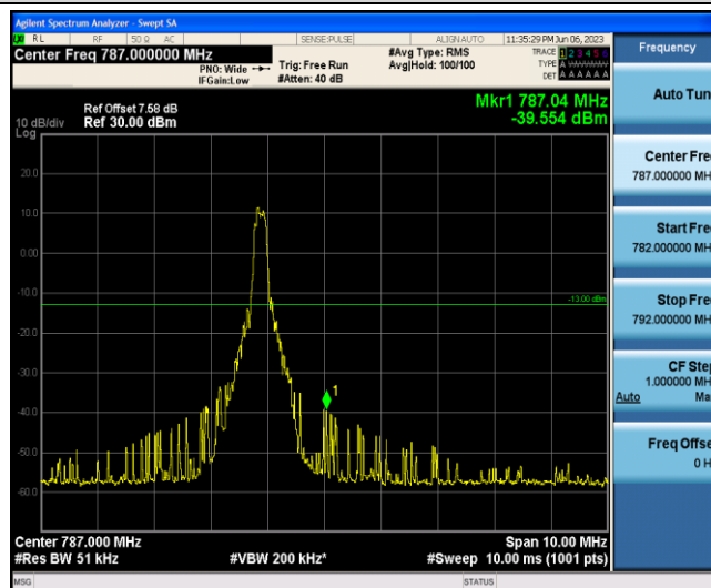
Band13-10MHz-QPSK-23230-1-5-High--39.55-PASS
