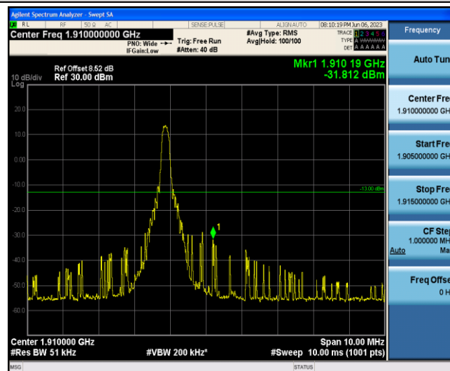
Band2-10MHz-QPSK-19150-1-5-High--31.81-PASS
