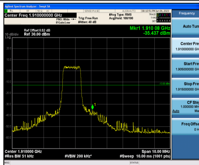
Band2-10MHz-16QAM-19150-6-0-High--35.44-PASS
