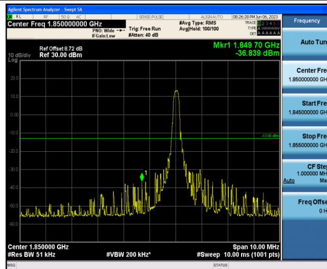
Band2-15MHz-16QAM-18675-1-0-Low--36.84-PASS
