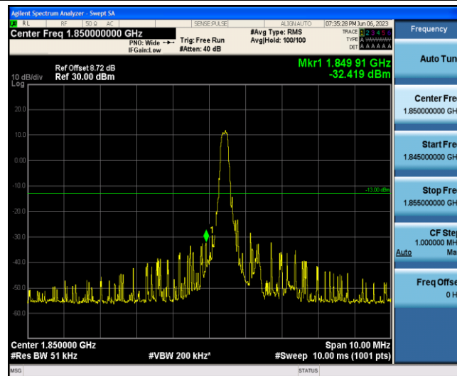
Band2-3MHz-16QAM-18615-1-0-Low--32.42-PASS
