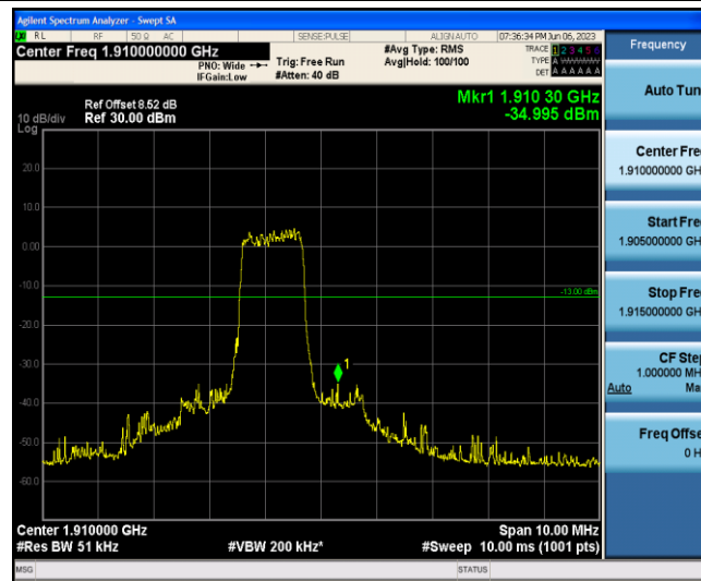
Band2-3MHz-16QAM-19185-6-0-High--34.99-PASS
