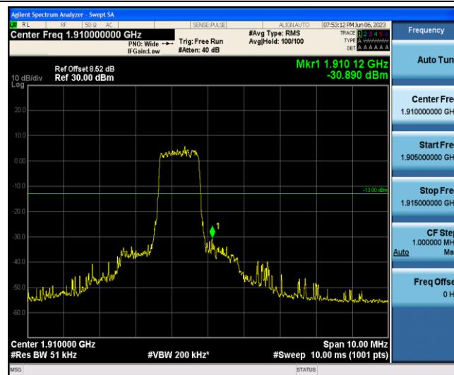
Band2-5MHz-QPSK-19175-6-0-High--30.89-PASS
