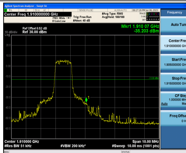
Band2-15MHz-QPSK-19125-6-0-High--35.20-PASS
