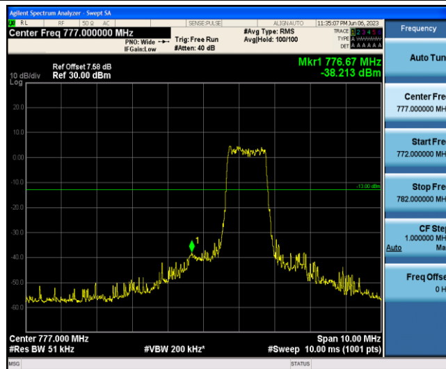
Band13-10MHz-QPSK-23230-6-0-Low--38.21-PASS
