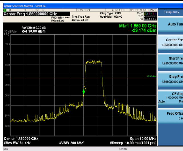
Band2-1.4MHz-QPSK-18607-6-0-Low--29.17-PASS
