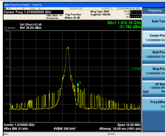
Band2-1.4MHz-16QAM-19193-1-5-High--31.78-PASS
