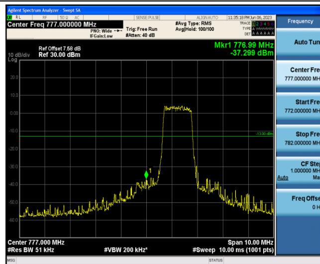
Band13-10MHz-16QAM-23230-6-0-Low--37.30-PASS
