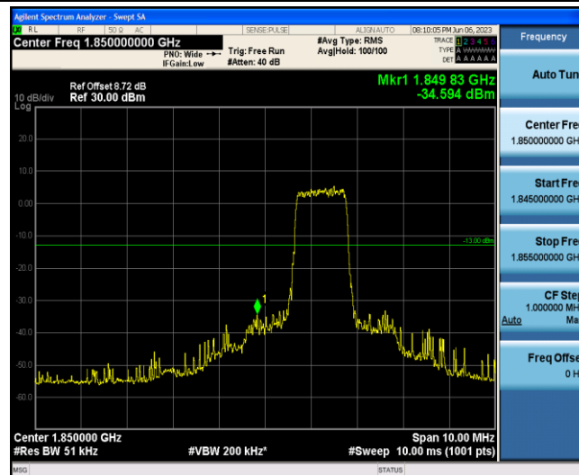
Band2-10MHz-16QAM-18650-6-0-Low--34.59-PASS
