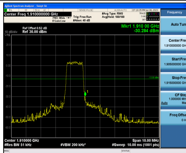
Band2-1.4MHz-16QAM-19193-6-0-High--30.28-PASS
