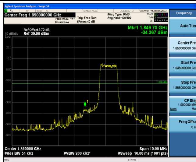
Band2-10MHz-QPSK-18650-6-0-Low--34.37-PASS
