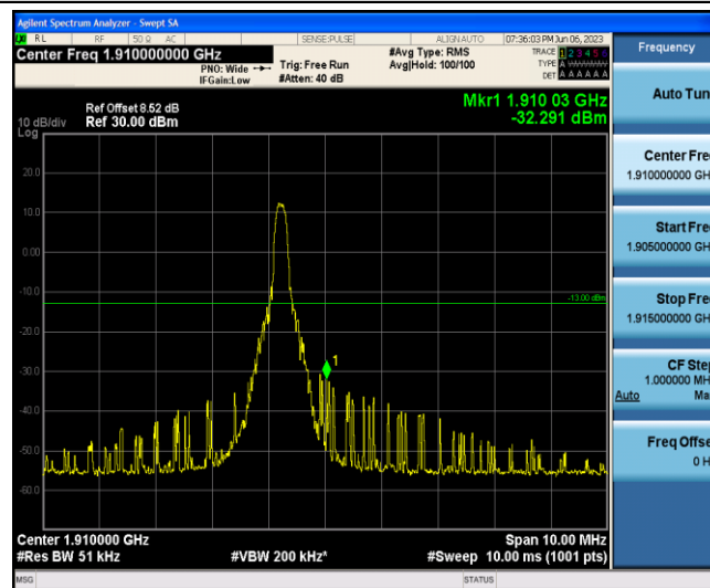
Band2-3MHz-QPSK-19185-1-5-High--32.29-PASS
