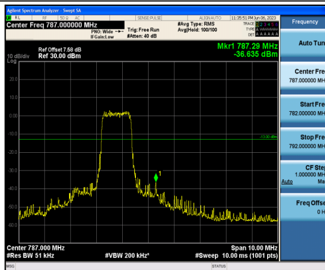
Band13-10MHz-QPSK-23230-6-0-High--36.64-PASS
