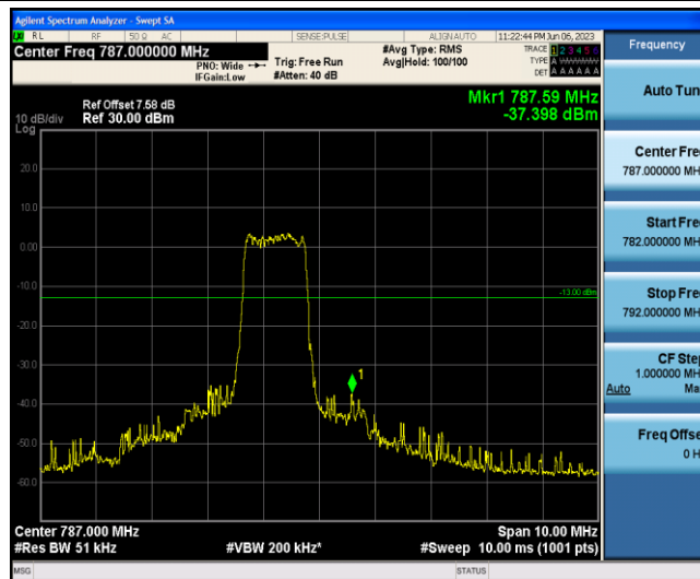
Band13-5MHz-16QAM-23255-6-0-High--37.40-PASS
