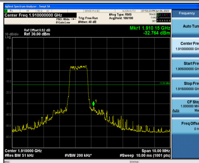
Band2-5MHz-16QAM-19175-6-0-High--32.76-PASS
