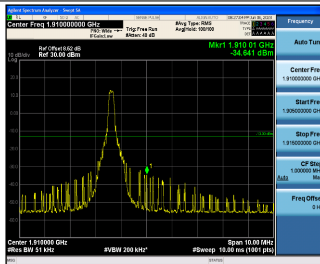
Band2-15MHz-QPSK-19125-1-5-High--34.64-PASS
