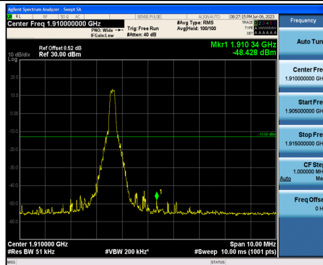
Band2-15MHz-16QAM-19125-1-5-High--48.43-PASS
