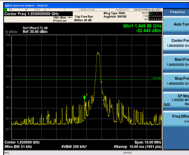
Band2-10MHz-QPSK-18650-1-0-Low--32.45-PASS
