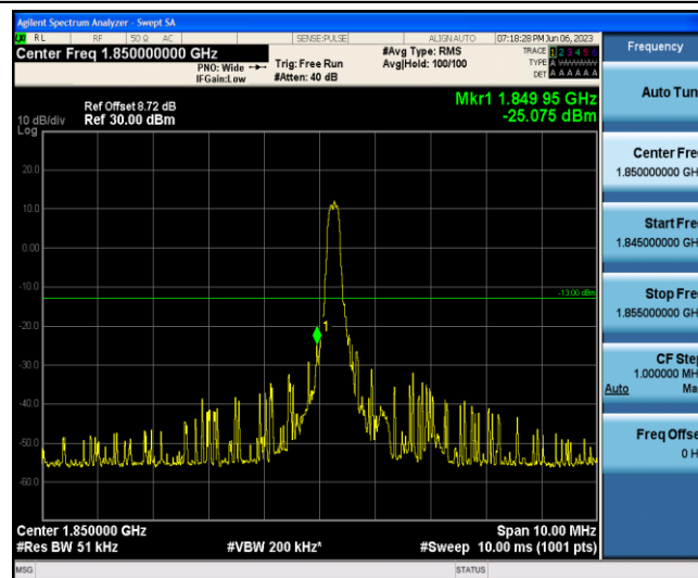
Band2-1.4MHz-16QAM-18607-1-0-Low--25.08-PASS
