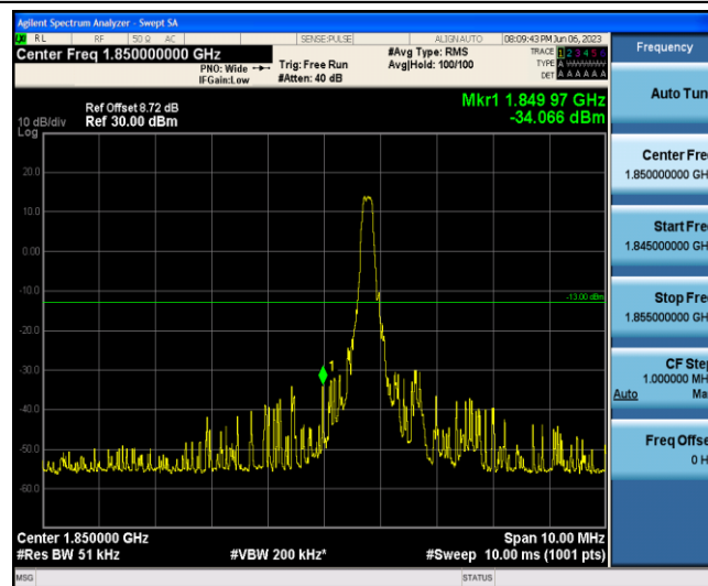
Band2-10MHz-16QAM-18650-1-0-Low--34.07-PASS
