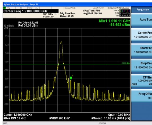
Band2-5MHz-QPSK-19175-1-5-High--31.69-PASS
