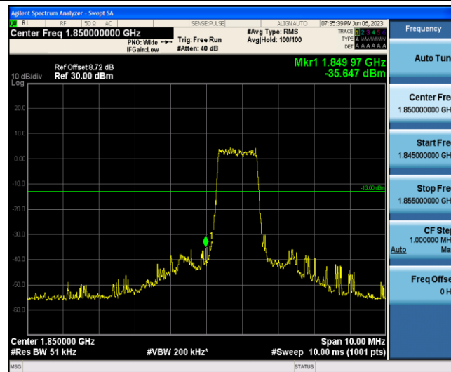
Band2-3MHz-QPSK-18615-6-0-Low--35.65-PASS
