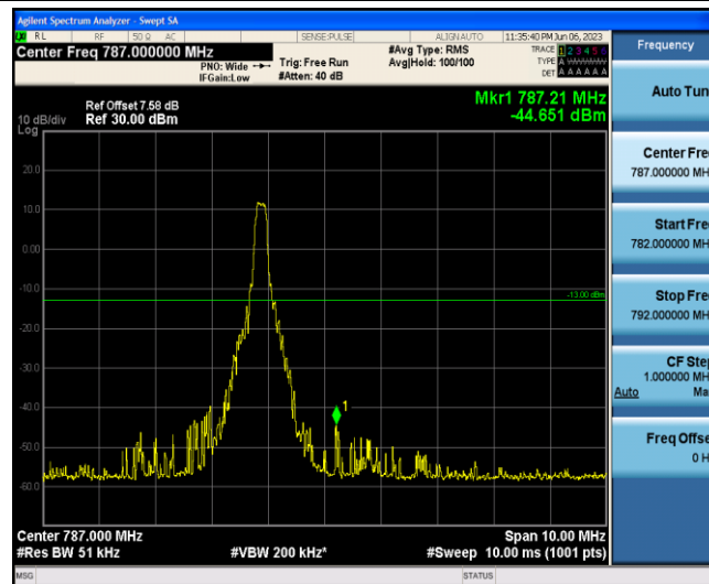
Band13-10MHz-16QAM-23230-1-5-High--44.65-PASS
