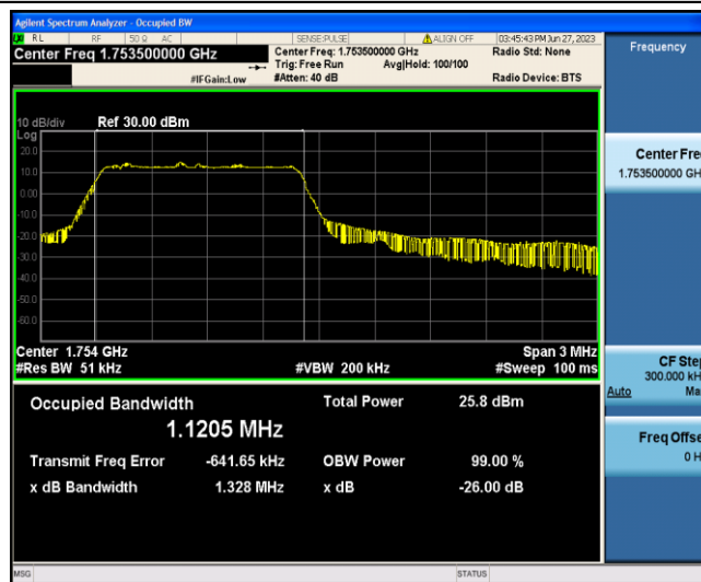
Band4-3MHz-16QAM-20385-6-0-Low-1.1205-1.328-PASS
