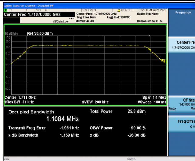
Band4-1.4MHz-16QAM-19957-6-0-Low-1.1084-1.359-PASS
