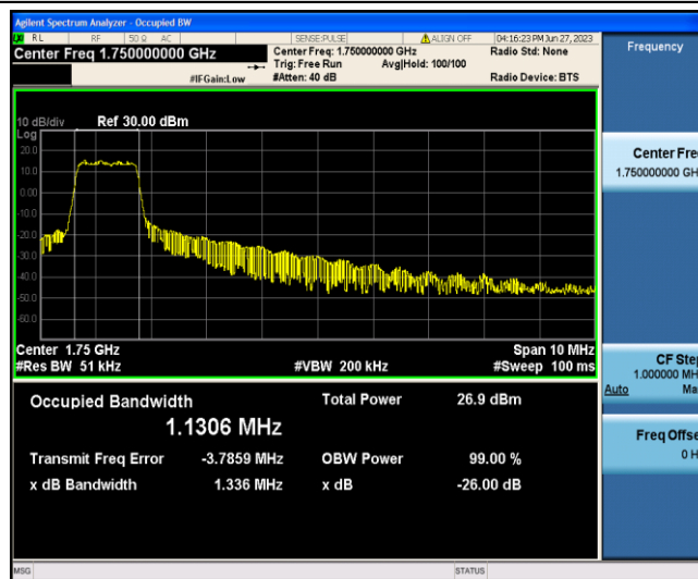
Band4-10MHz-16QAM-20350-6-0-Low-1.1306-1.336-PASS
