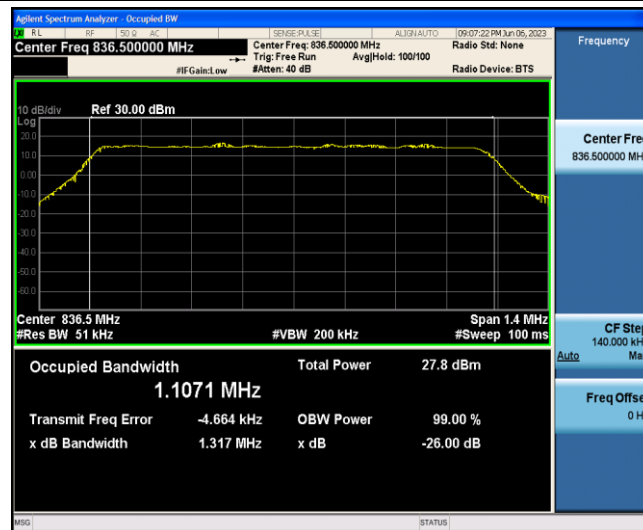
Band5-1.4MHz-QPSK-20525-6-0-Low-1.1071-1.317-PASS
