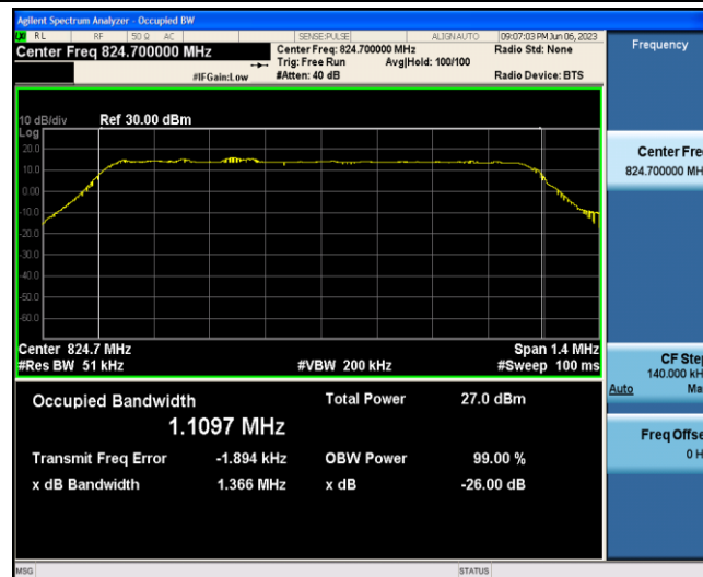
Band5-1.4MHz-16QAM-20407-6-0-Low-1.1097-1.366-PASS
