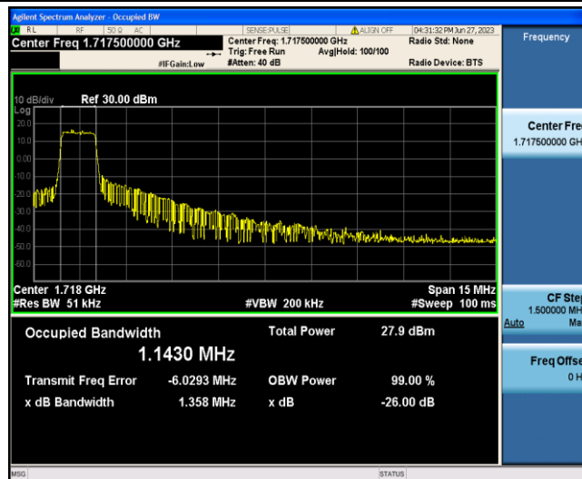
Band4-15MHz-QPSK-20025-6-0-Low-1.1430-1.358-PASS
