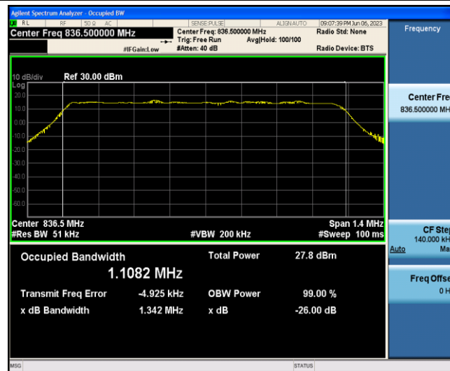
Band5-1.4MHz-16QAM-20525-6-0-Low-1.1082-1.342-PASS
