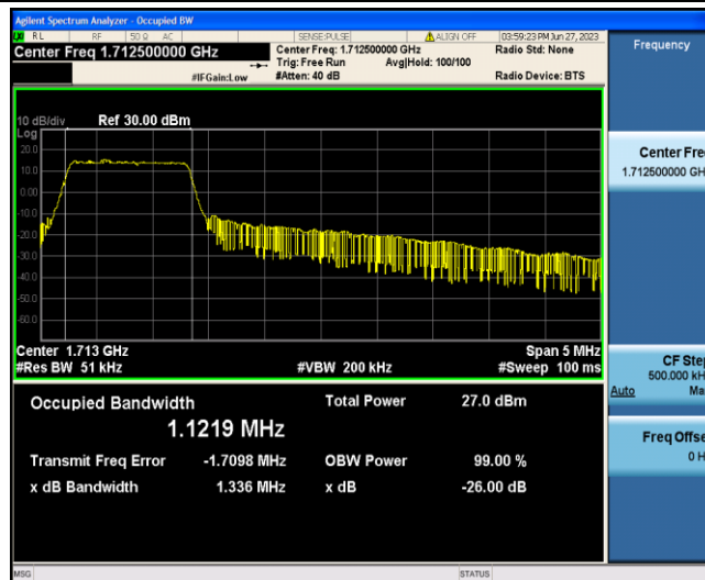
Band4-5MHz-QPSK-19975-6-0-Low-1.1219-1.336-PASS
