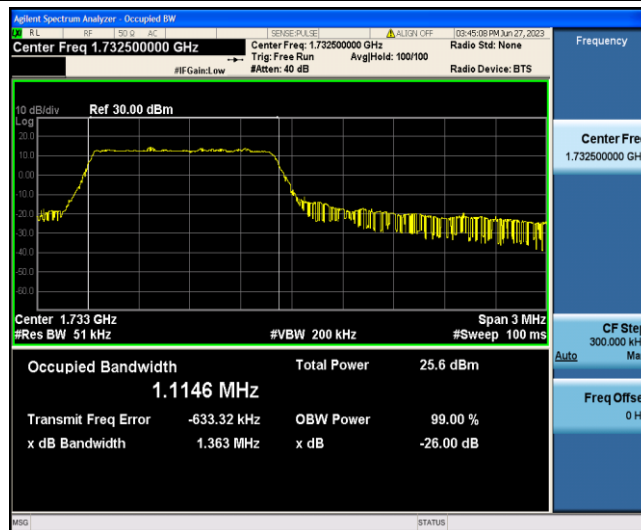
Band4-3MHz-16QAM-20175-6-0-Low-1.1146-1.363-PASS
