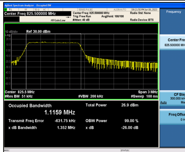
Band5-3MHz-QPSK-20415-6-0-Low-1.1159-1.352-PASS
