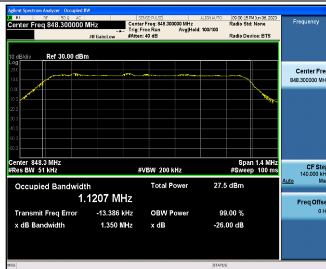
Band5-1.4MHz-16QAM-20643-6-0-Low-1.1207-1.350-PASS
