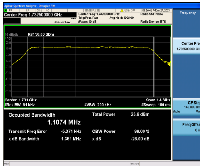
Band4-1.4MHz-QPSK-20175-6-0-Low-1.1074-1.361-PASS
