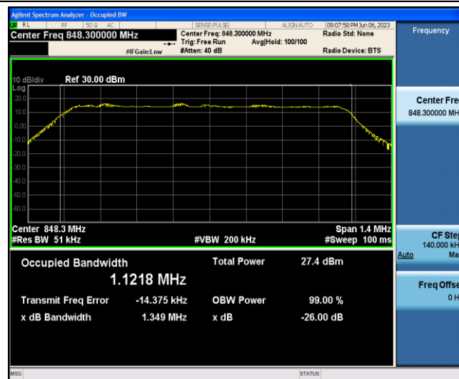
Band5-1.4MHz-QPSK-20643-6-0-Low-1.1218-1.349-PASS
