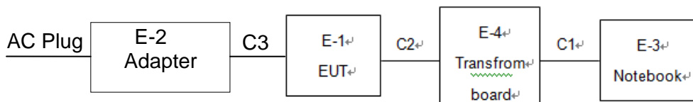
Block diagram of EUT configuration(TX Mode)
