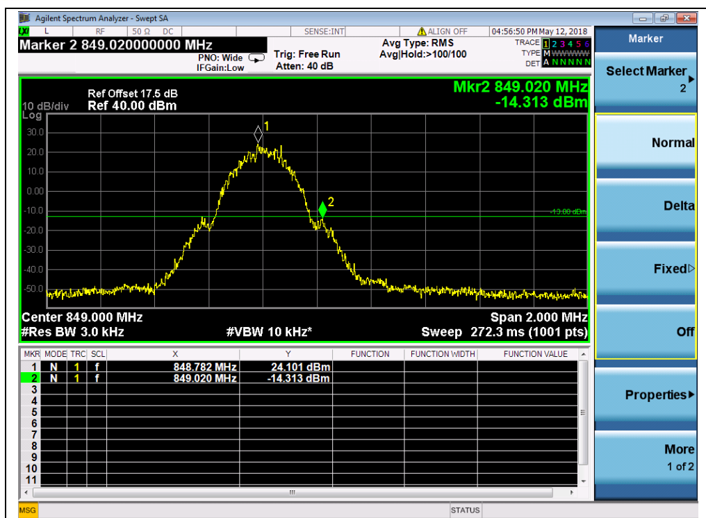
(Plot A2, GSM 850, Channel = 251)
