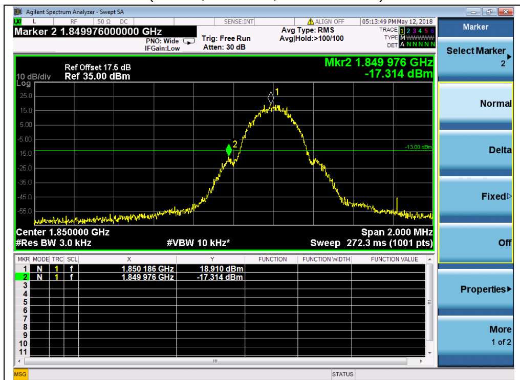
(Plot B1, GSM 1900, Channel = 512)
