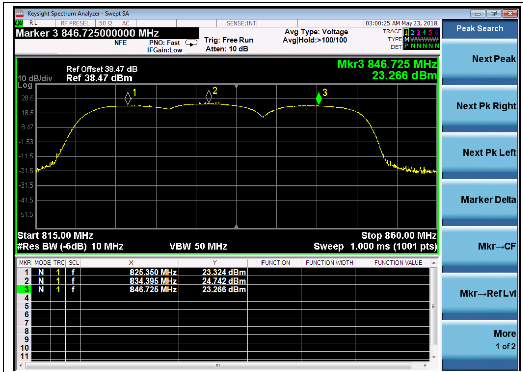
(Plot G, WCDMA 850 MHz, Channel = 4132, 4175, 4233)
