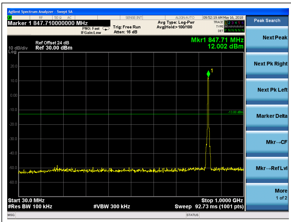
(Plot M3, HSUPA 850MHz, Channel = 4233, 30MHz to 1GHz)
