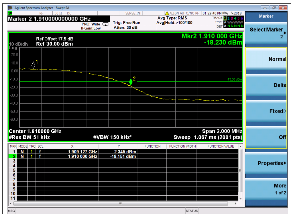
(Plot P2, HSPA+ 1900, Channel = 9538)
