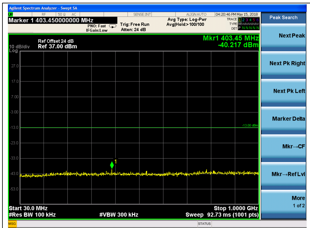
(Plot I3, WCDMA1900MHz, Channel = 9538, 30MHz to 1GHz)
