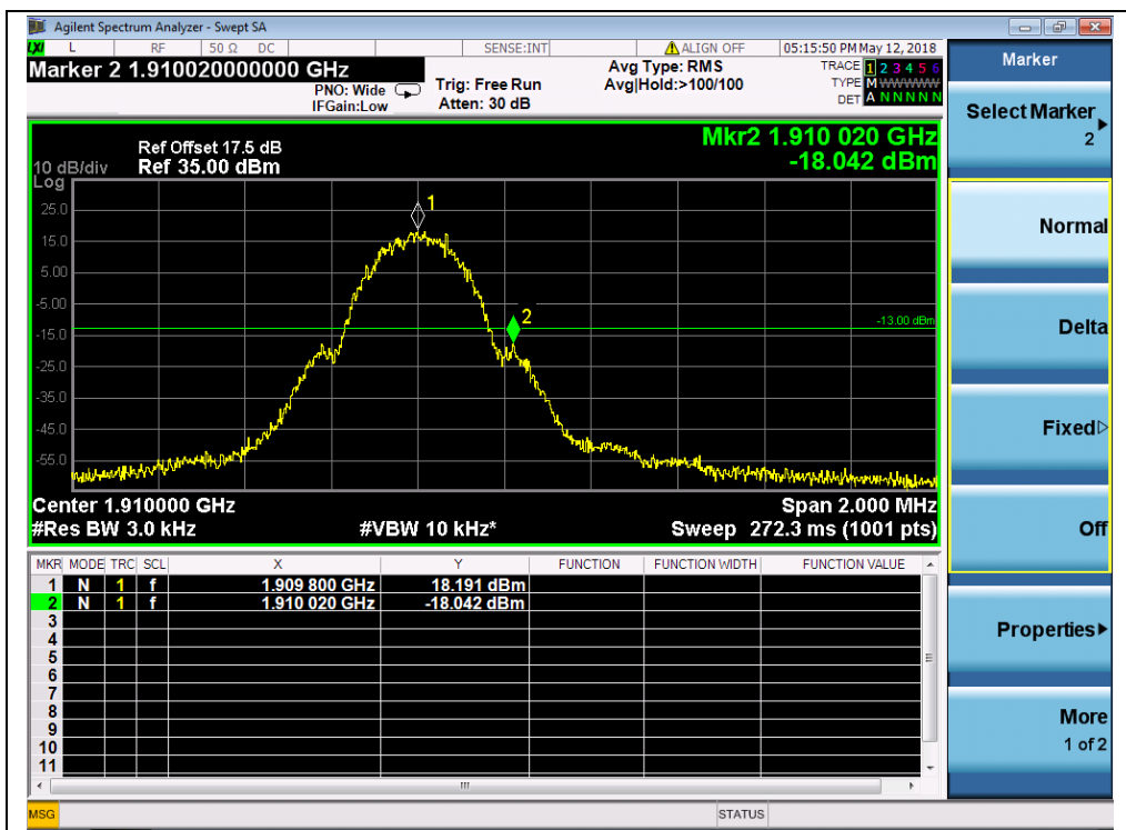
(Plot B2, GSM 1900, Channel = 810)
