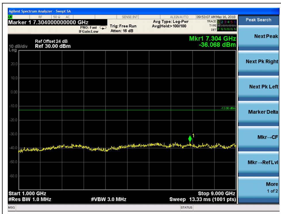
(Plot M3.1, HSUPA 850MHz, Channel = 4233, 1GHz to 9GHz)
