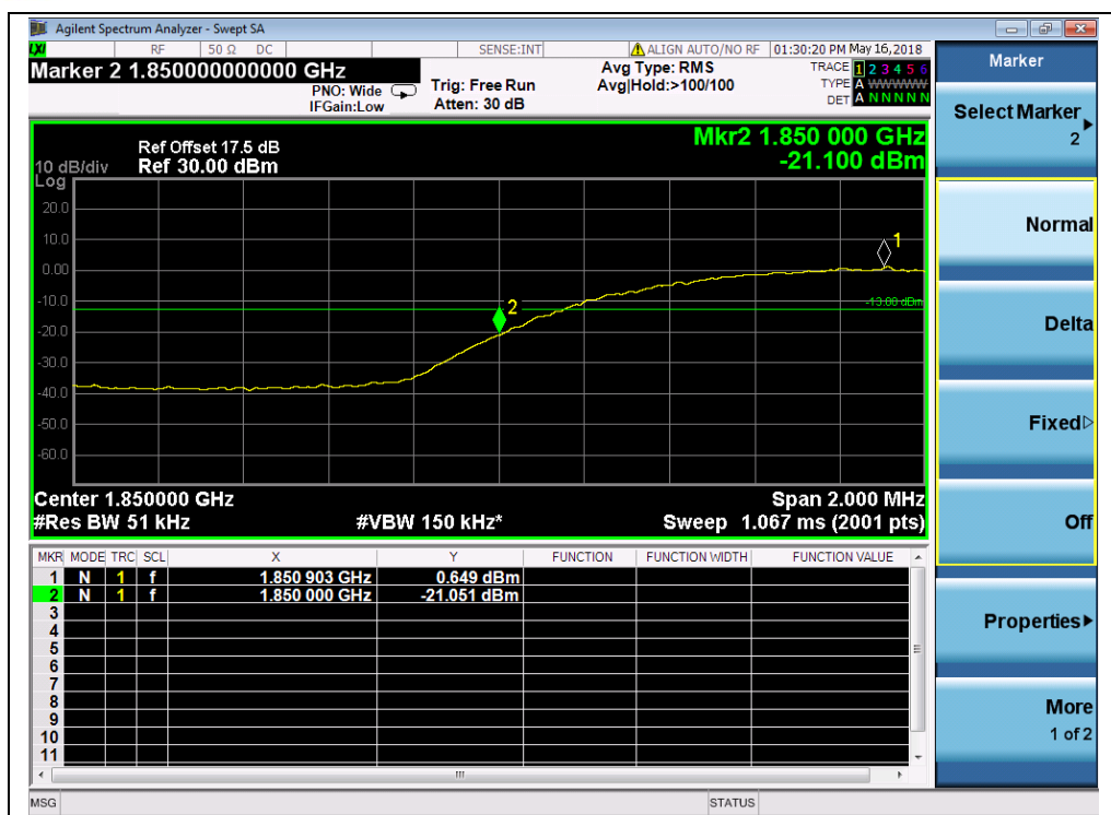
(Plot P1, HSPA+ 1900, Channel = 9262)
