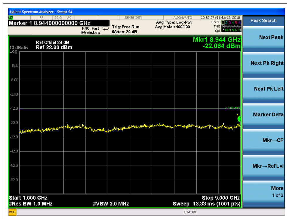
(Plot M2.1, HSUPA 850MHz, Channel = 4175, 1GHz to 9GHz)
