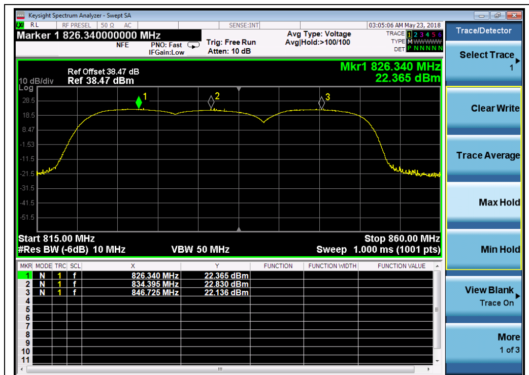
(Plot H, HSDPA 850 MHz, Channel = 4132, 4175, 4233)
