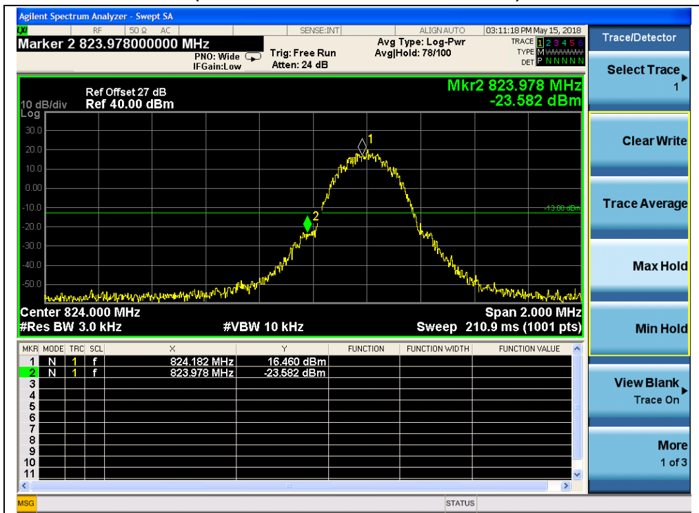
(Plot C1, EGPRS 850, Channel = 128)
