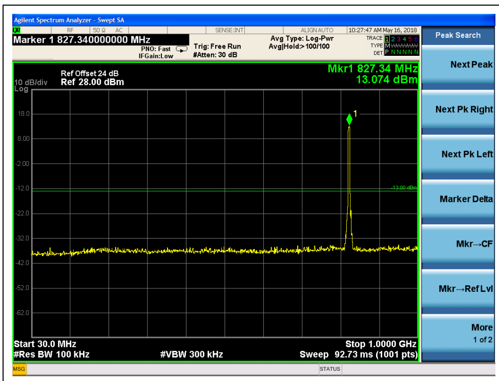
(Plot M1, HSUPA 850MHz, Channel = 4132, 30MHz to 1GHz)
