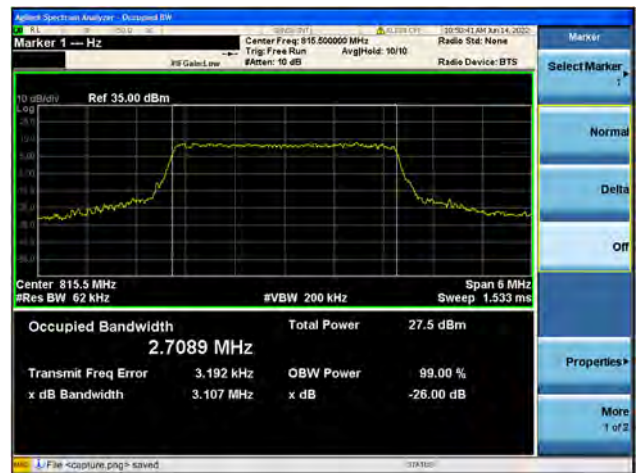
B26Part90 / 3MHz / 64QAM/ Low CH
