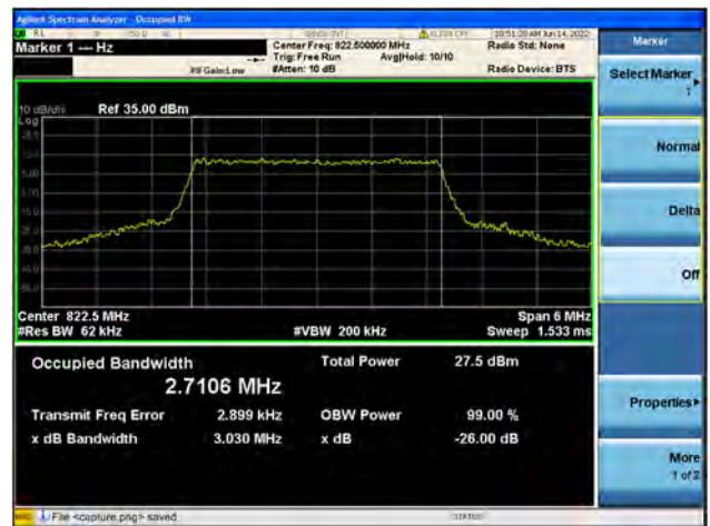
B26Part90 / 3MHz / 64QAM/ High CH
