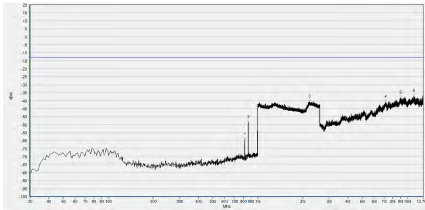
LTE Band 26, 5MHz BW, Low Channel, QPSK
