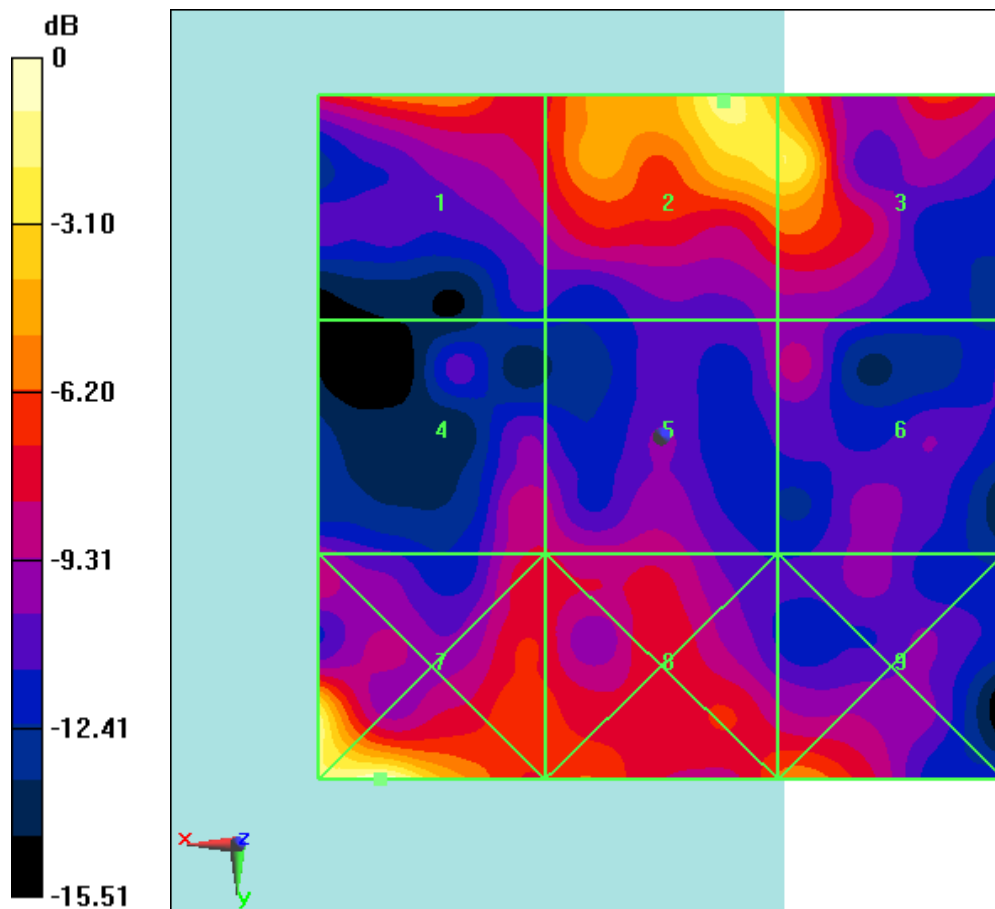
Fig B.11 HAC RF E-Field CDMA BC1 Middle
