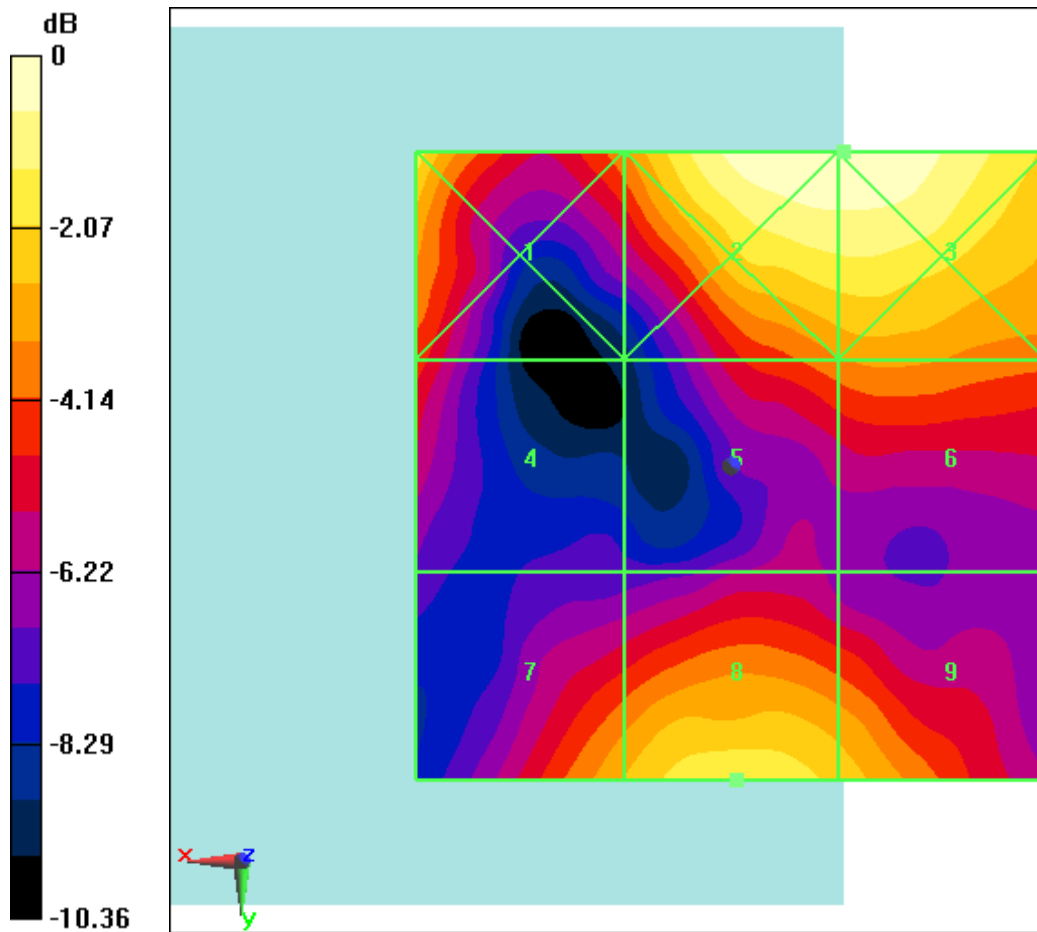
Fig B.35 HAC RF E-Field LTE Band41 Power Class 3 QPSK CH39750
