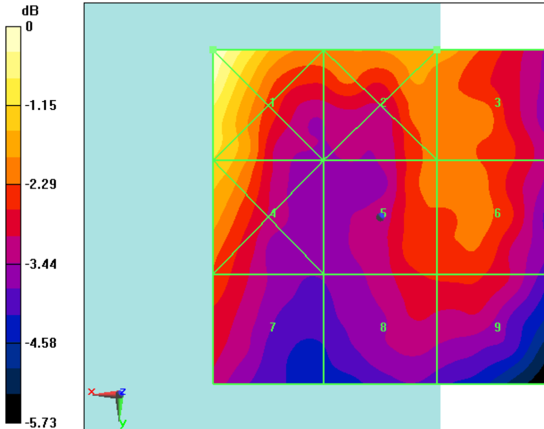
Fig B.30 HAC RF E-Field LTE Band41 Power Class 2 64QAM CH39750
