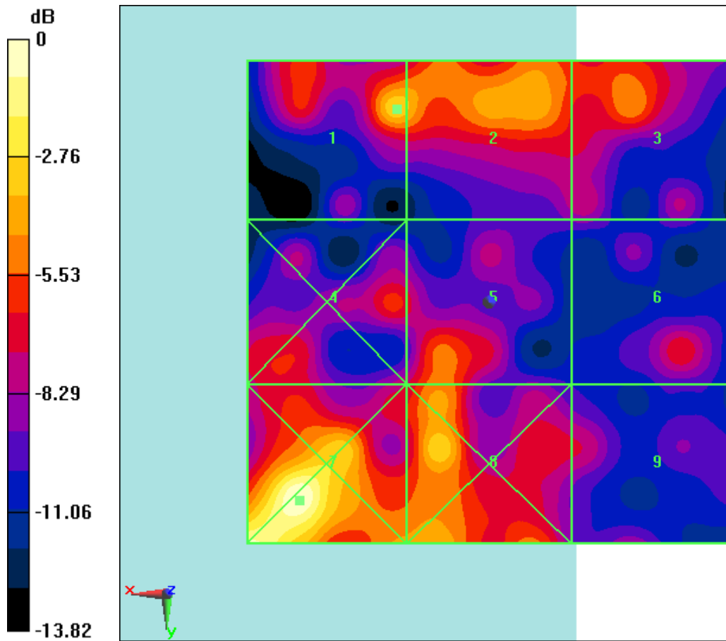
Fig B.12 HAC RF E-Field CDMA BC1 Low
