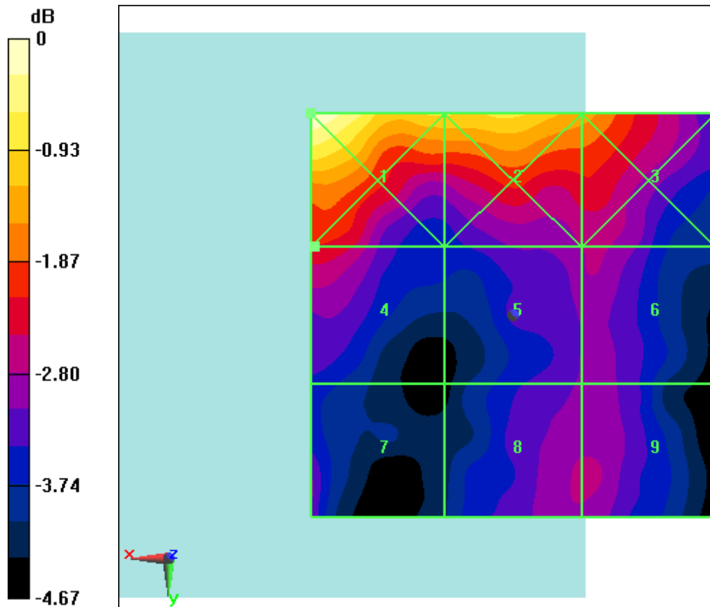
Fig B.23 HAC RF E-Field LTE Band41 Power Class 2 16QAM CH40620
