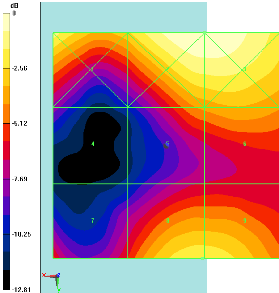
Fig B.16 HAC RF E-Field LTE Band41 Power Class 2 QPSK CH41490
