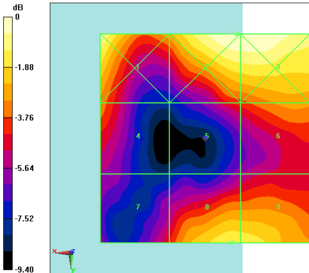
Fig B.34 HAC RF E-Field LTE Band41 Power Class 3 QPSK CH40185
