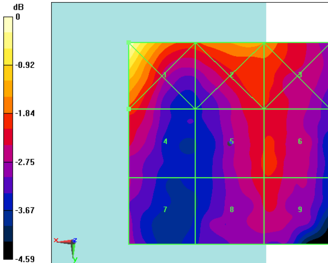
Fig B.24 HAC RF E-Field LTE Band41 Power Class 2 16QAM CH40185
