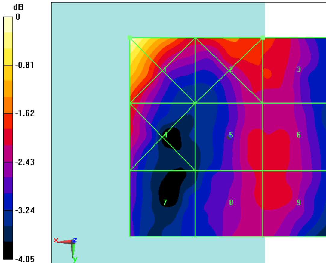
Fig B.21 HAC RF E-Field LTE Band41 Power Class 2 16QAM CH41490
