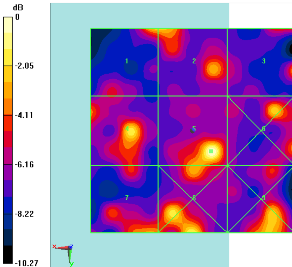
Fig B.13 HAC RF E-Field CDMA BC10 High
