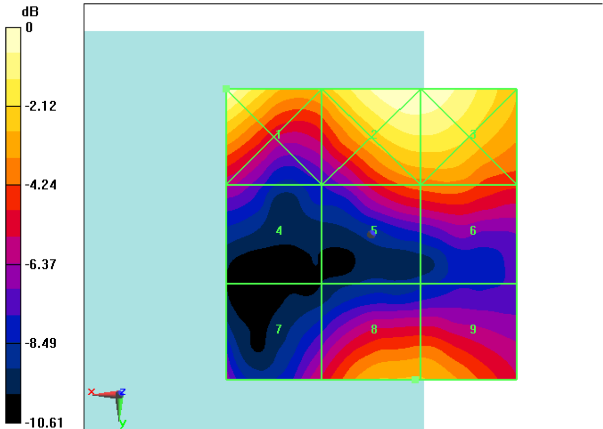
Fig B.17 HAC RF E-Field LTE Band41 Power Class 2 QPSK CH41055
