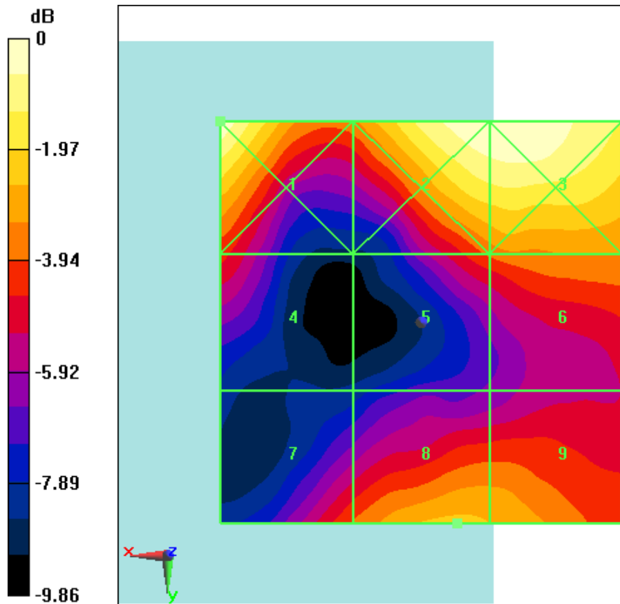
Fig B.19 HAC RF E-Field LTE Band41 Power Class 2 QPSK CH40185
