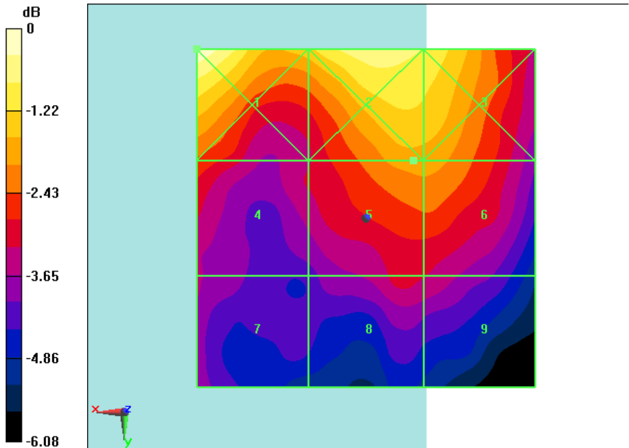
Fig B.27 HAC RF E-Field LTE Band41 Power Class 2 64QAM CH41055
