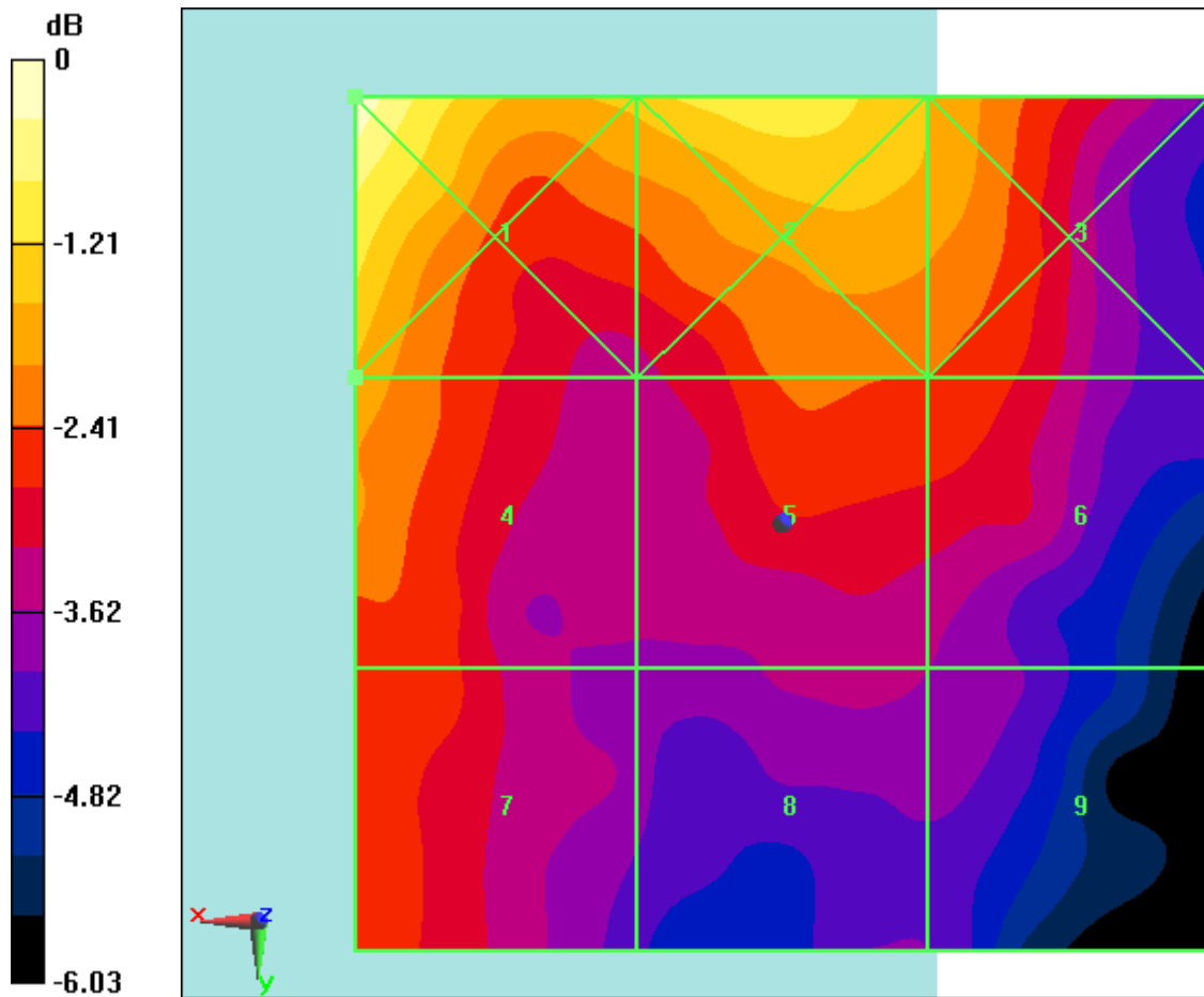
Fig B.37 HAC RF E-Field LTE Band41 Power Class 3 16QAM CH41055
