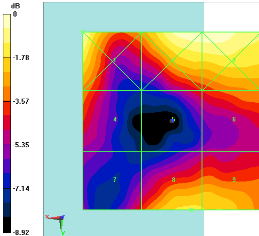
Fig B.39 HAC RF E-Field LTE Band41 Power Class 3 16QAM CH40185
