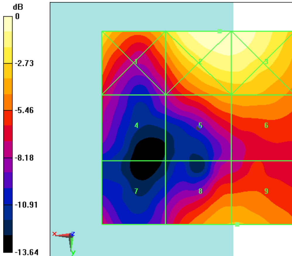
Fig B.41 HAC RF E-Field LTE Band41 Power Class 3 64QAM CH41490
