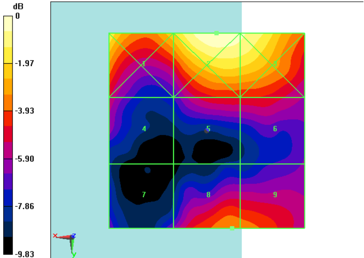
Fig B.42 HAC RF E-Field LTE Band41 Power Class 3 64QAM CH41055
