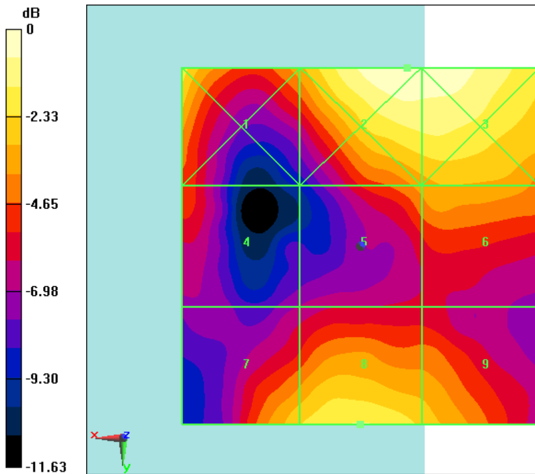
Fig B.40 HAC RF E-Field LTE Band41 Power Class 3 16QAM CH39750
