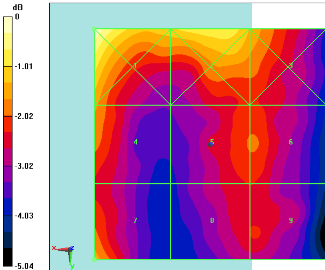
Fig B.36 HAC RF E-Field LTE Band41 Power Class 3 16QAM CH41490
