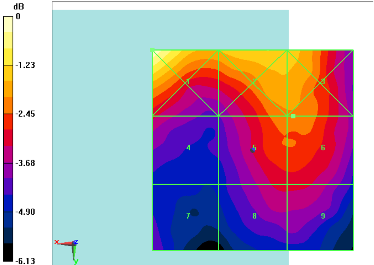
Fig B.22 HAC RF E-Field LTE Band41 Power Class 2 16QAM CH41055
