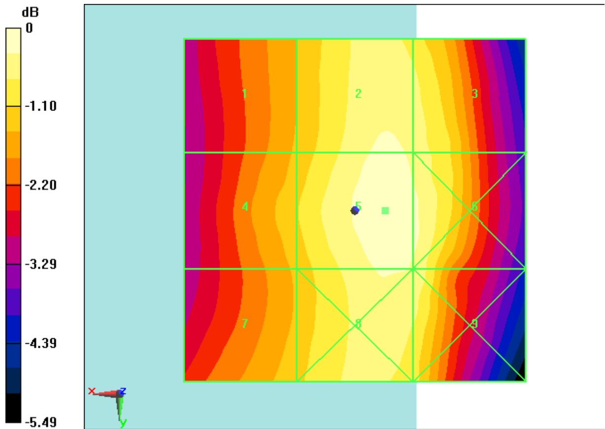
Fig B.2 HAC RF E-Field GSM 850 Middle
