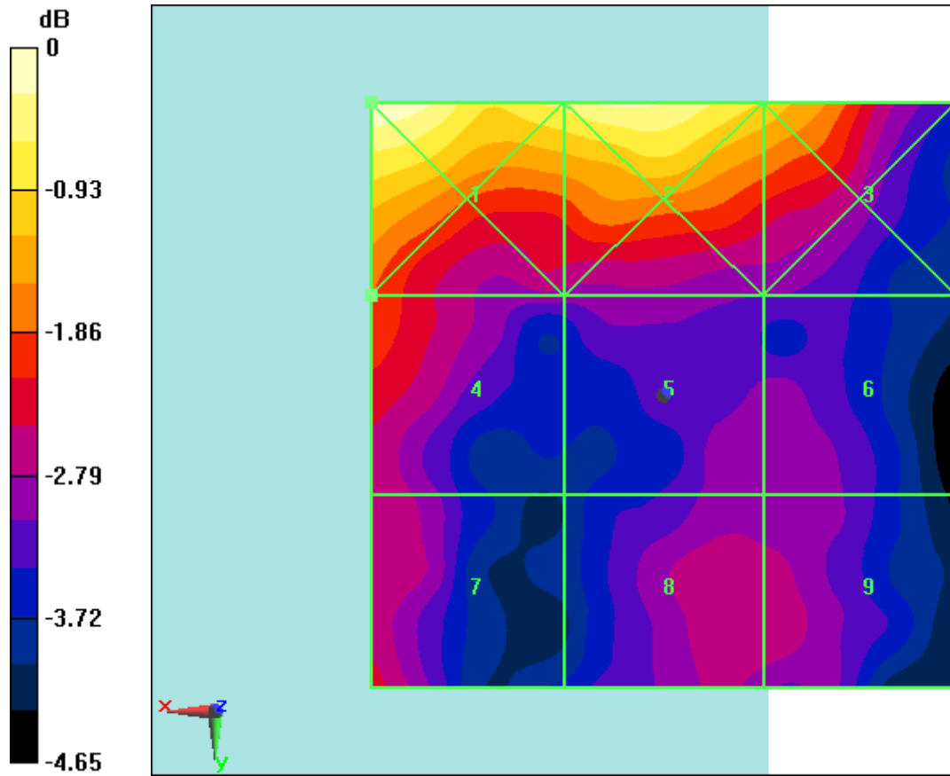
Fig B.28 HAC RF E-Field LTE Band41 Power Class 2 64QAM CH40620
