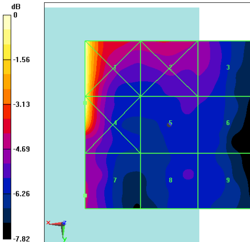
Fig B.38 HAC RF E-Field LTE Band41 Power Class 3 16QAM CH40620
