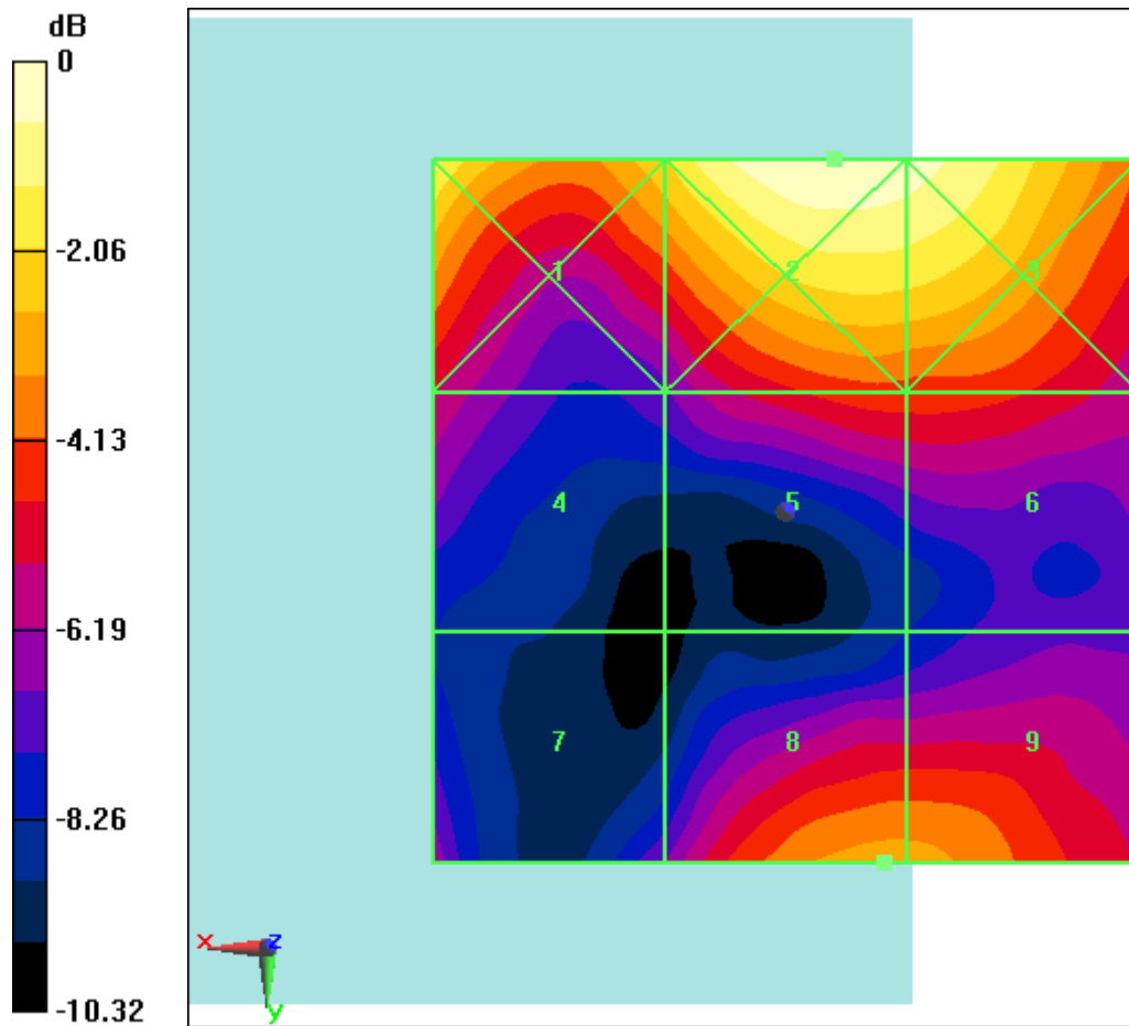
Fig B.32 HAC RF E-Field LTE Band41 Power Class 3 QPSK CH41055
