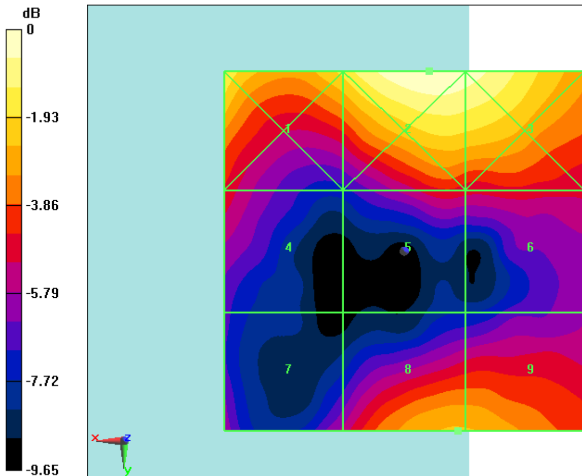
Fig B.33 HAC RF E-Field LTE Band41 Power Class 3 QPSK CH40620
