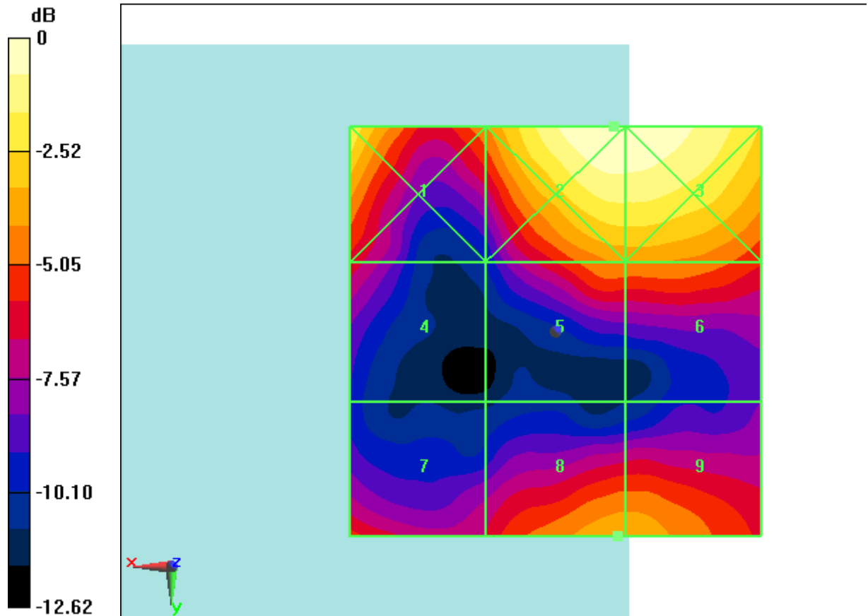
Fig B.20 HAC RF E-Field LTE Band41 Power Class 2 QPSK CH39750
