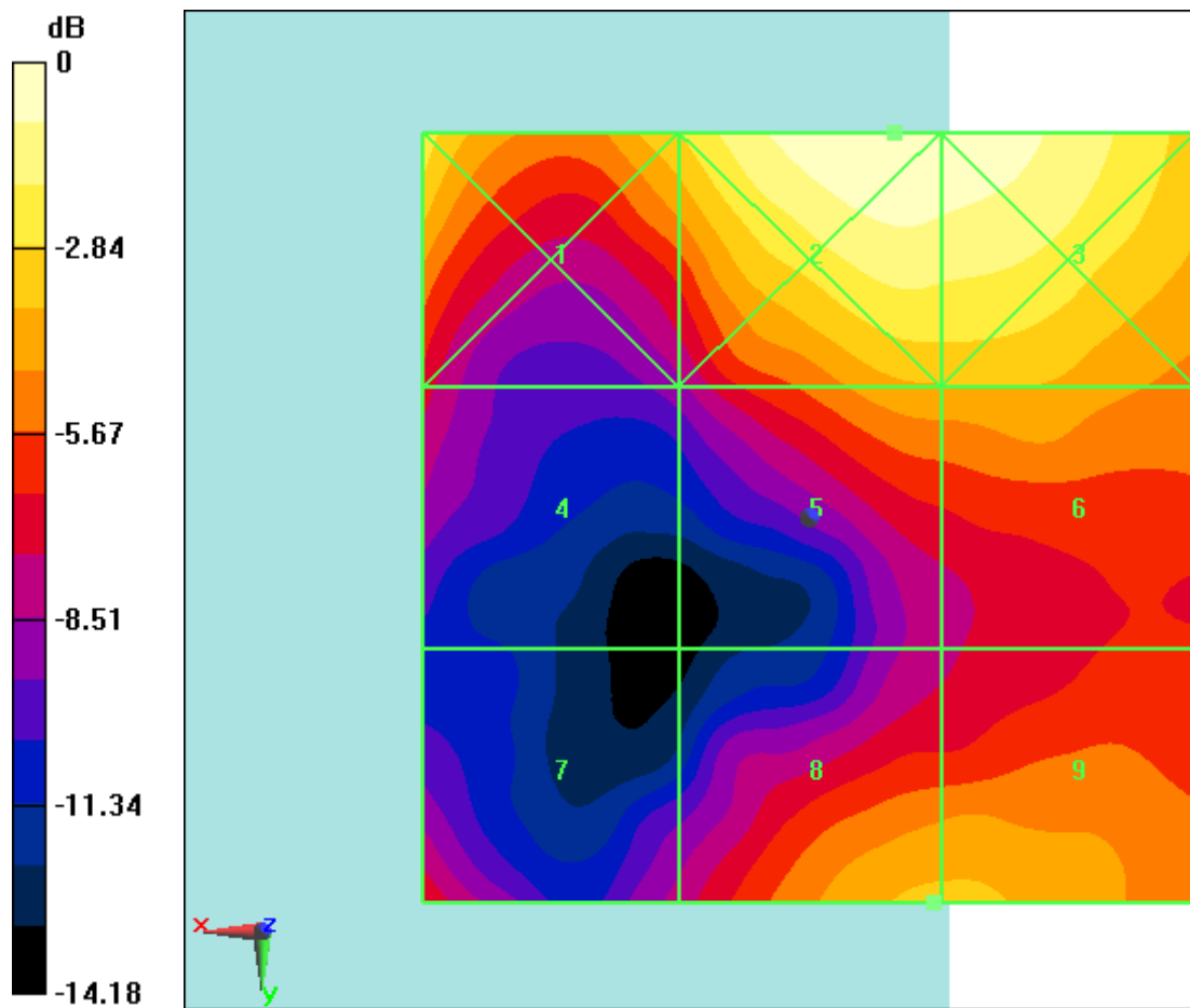
Fig B.31 HAC RF E-Field LTE Band41 Power Class 3 QPSK CH41490
