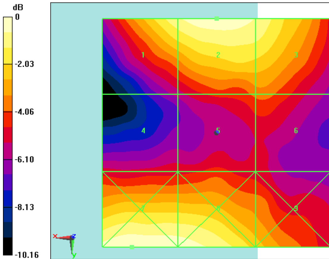
Fig B.6 HAC RF E-Field GSM 1900 Low
