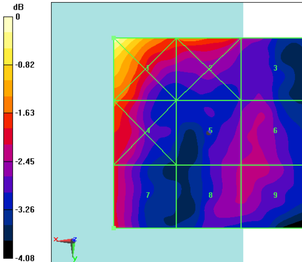
Fig B.29 HAC RF E-Field LTE Band41 Power Class 2 64QAM CH40185
