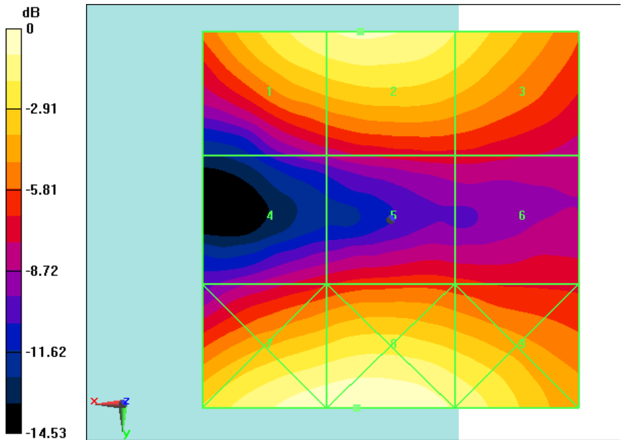
Fig B.4 HAC RF E-Field GSM 1900 High
