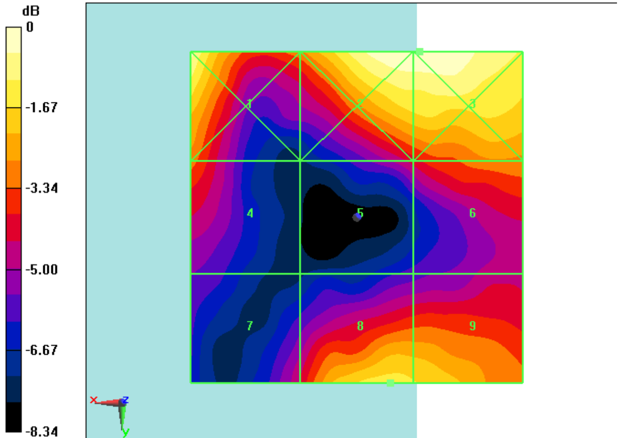
Fig B.44 HAC RF E-Field LTE Band41 Power Class 3 64QAM CH40185
