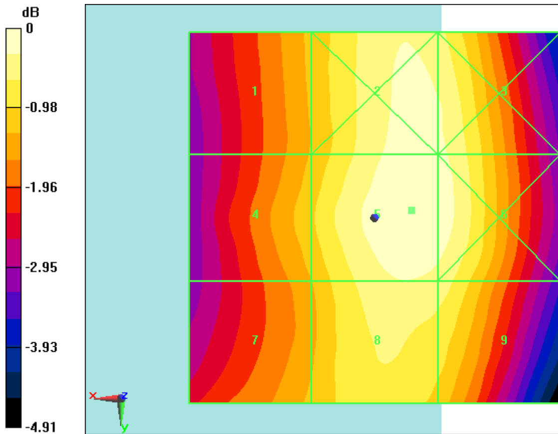
Fig B.1 HAC RF E-Field GSM 850 High
