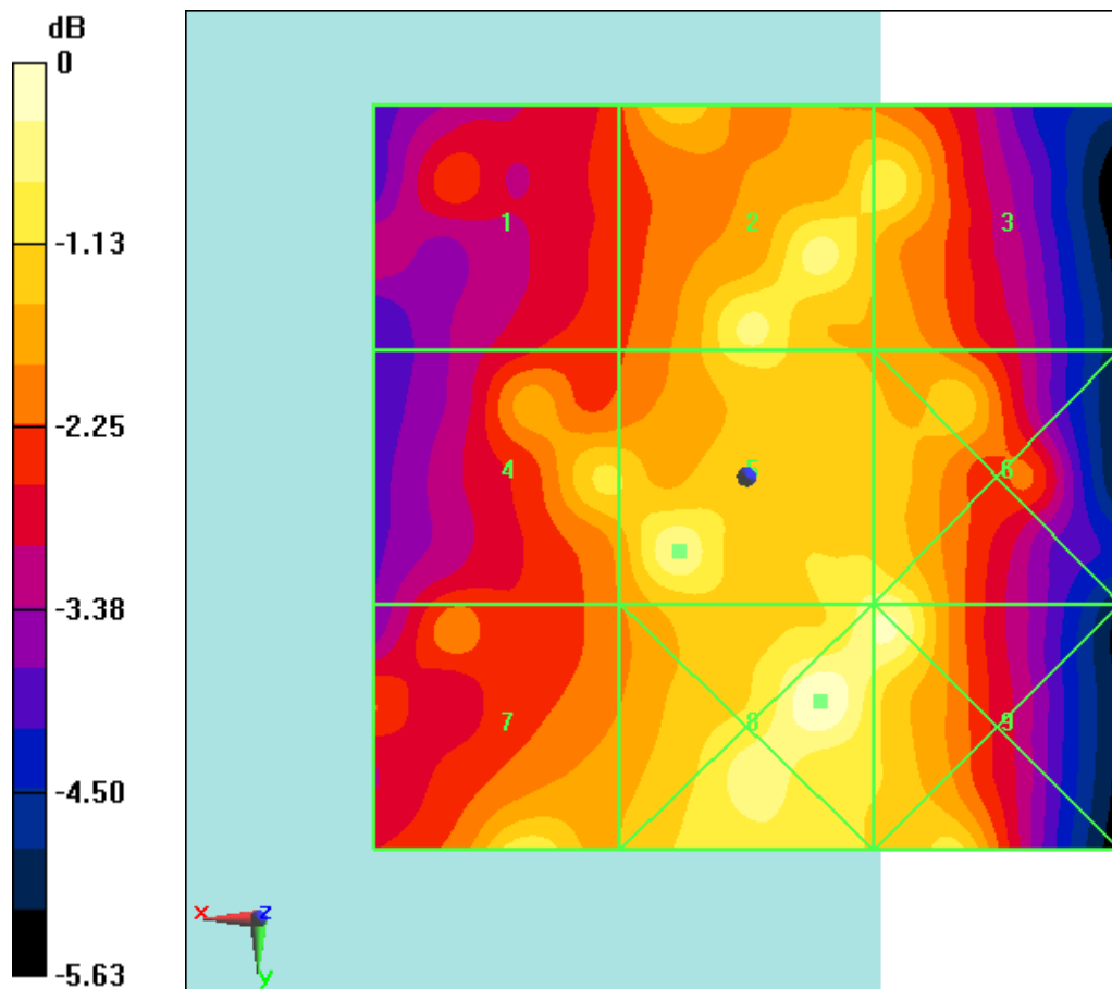
Fig B.7 HAC RF E-Field CDMA BC0 High
