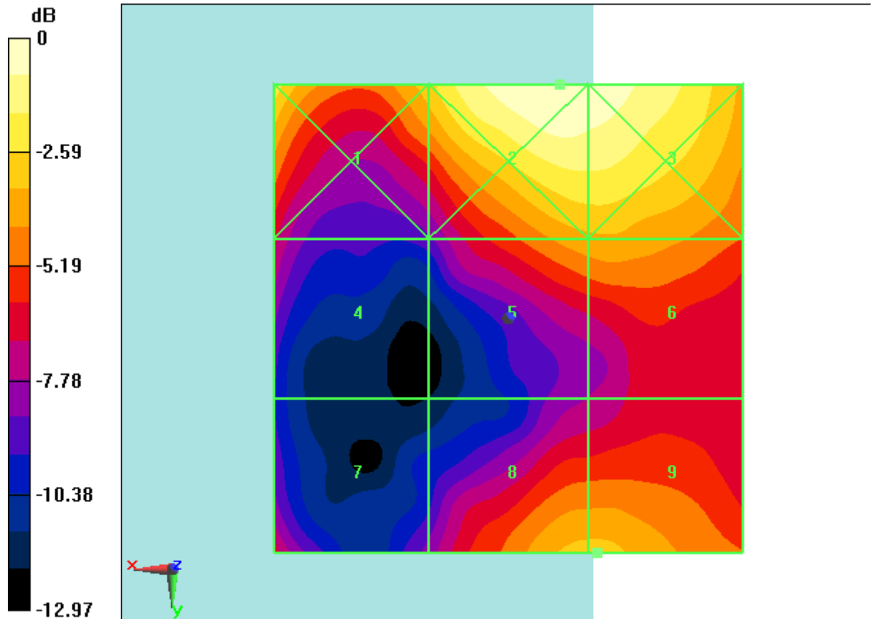
Fig B.45 HAC RF E-Field LTE Band41 Power Class 3 64QAM CH39750
