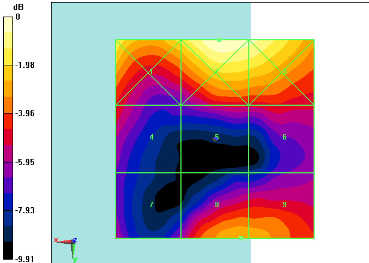
Fig B.43 HAC RF E-Field LTE Band41 Power Class 3 64QAM CH40620
