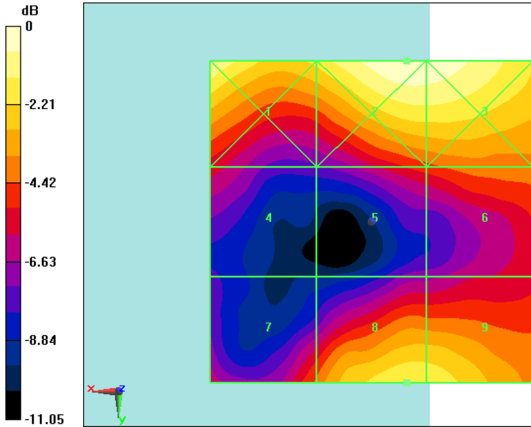
Fig B.18 HAC RF E-Field LTE Band41 Power Class 2 QPSK CH40620
