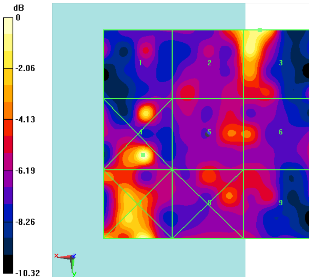
Fig B.14 HAC RF E-Field CDMA BC10 Middle
