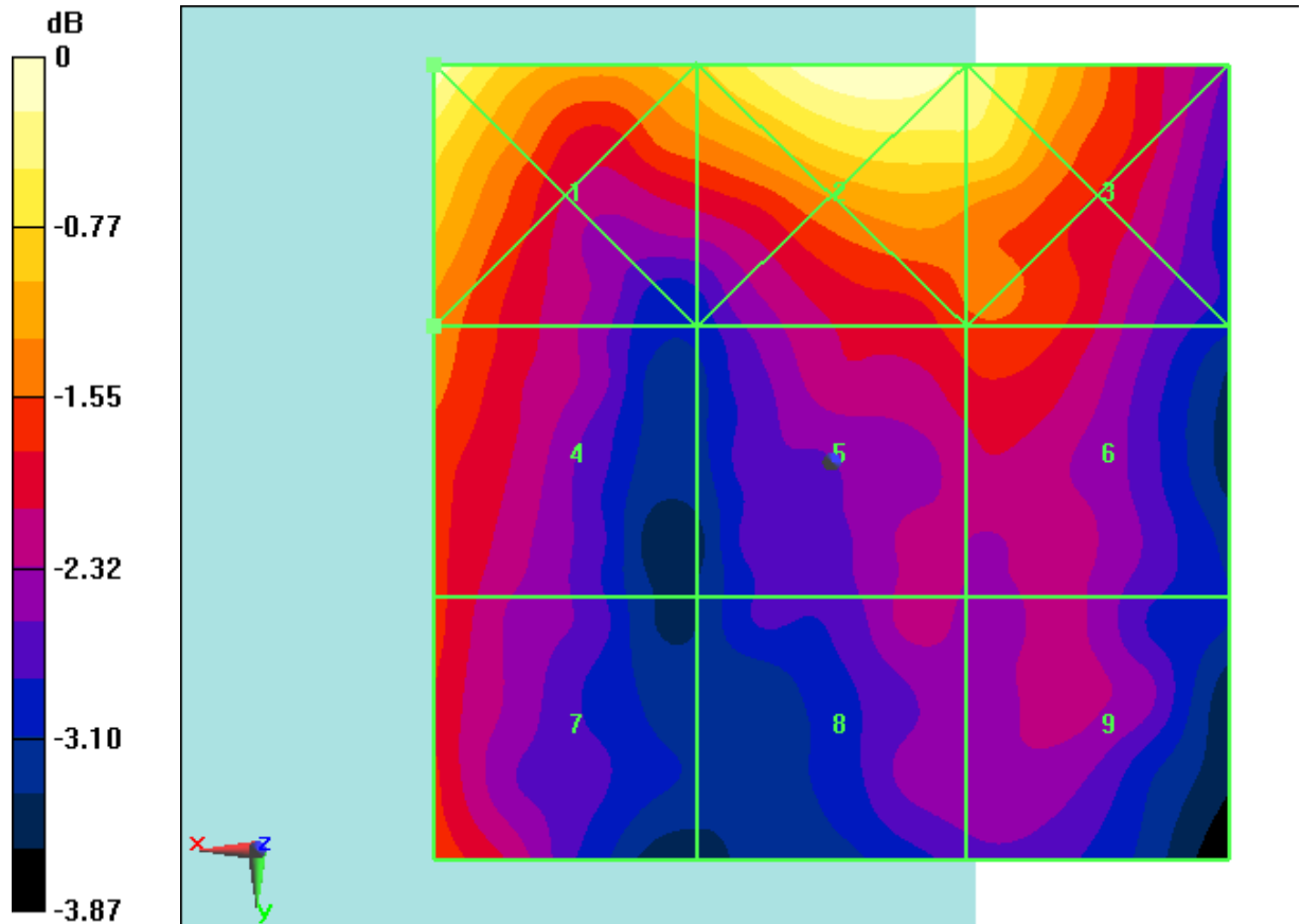
Fig B.25 HAC RF E-Field LTE Band41 Power Class 2 16QAM CH39750
