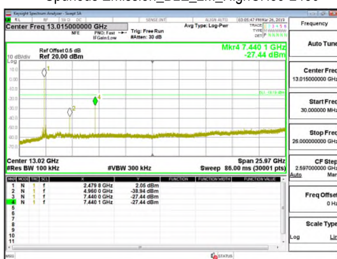
Spurious Emission_BLE_2M_HighCH39-2480
