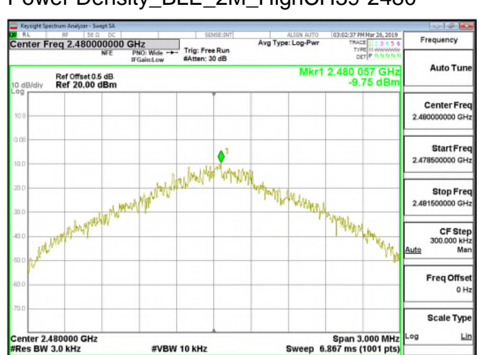
Power Density_BLE_2M_HighCH39-2480
