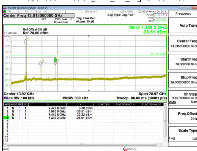
Spurious Emission_BLE_1M_HighCH39-2480
