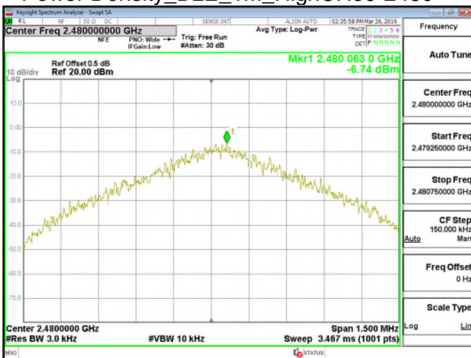
Power Density_BLE_1M_HighCH39-2480
