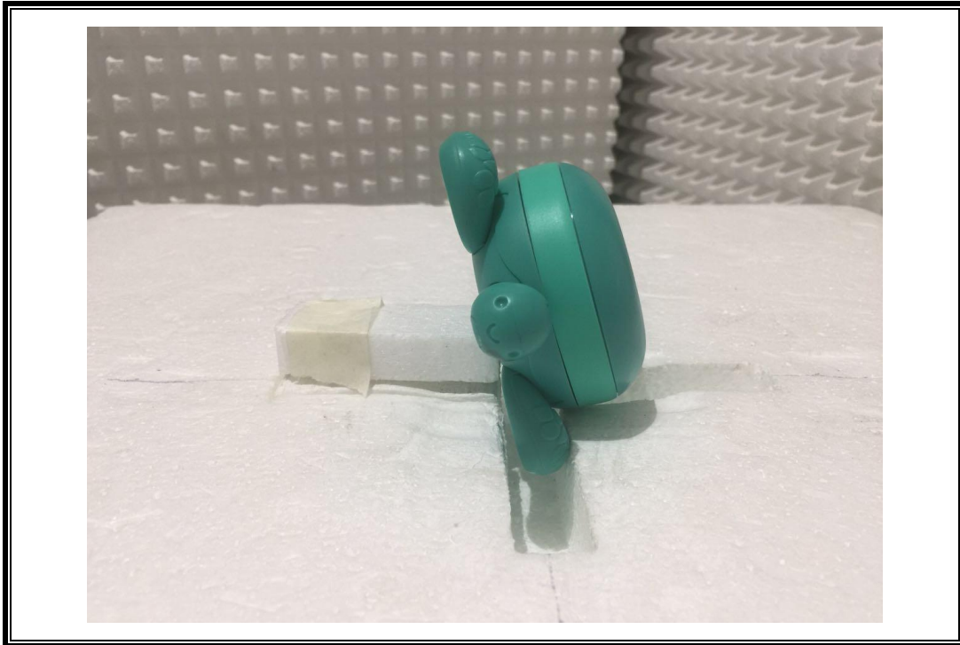
RADIATED RF MEASUREMENT POSITION (Z axis)
