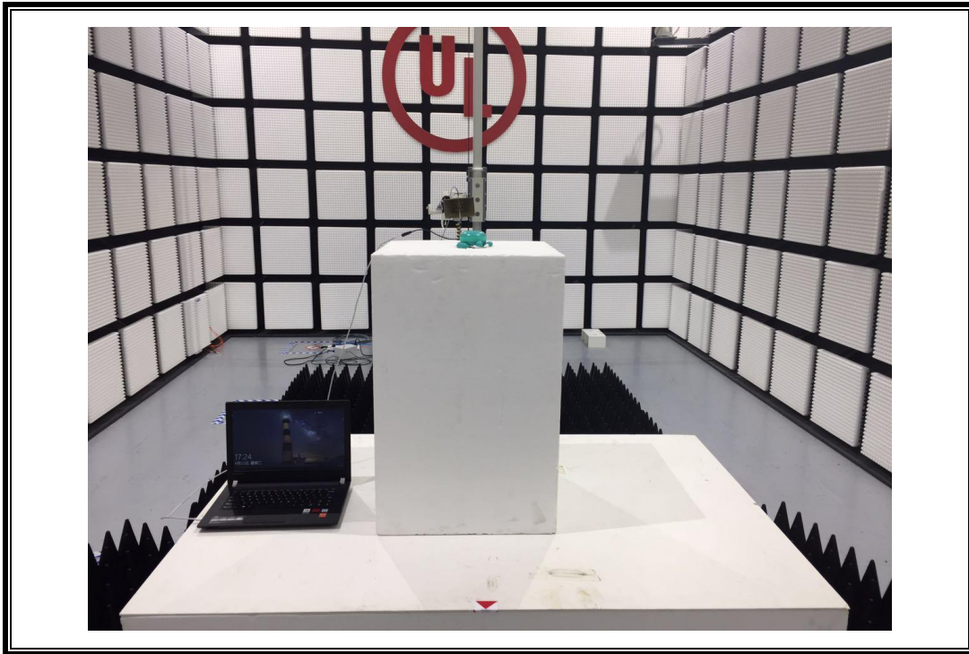
RADIATED RF MEASUREMENT POSITION (X axis)
