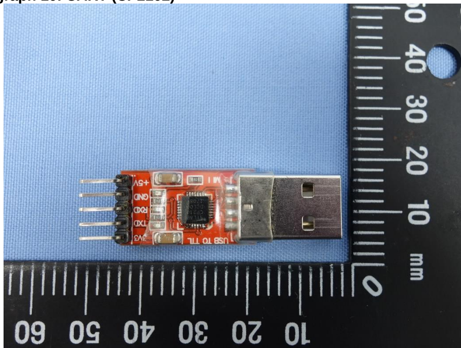
Photograph 10: UART (CP2102)
