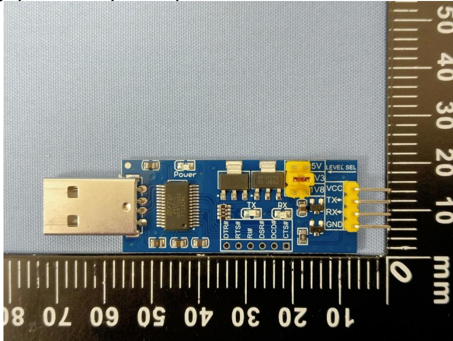
Photograph 11: UART (FT232RL)
