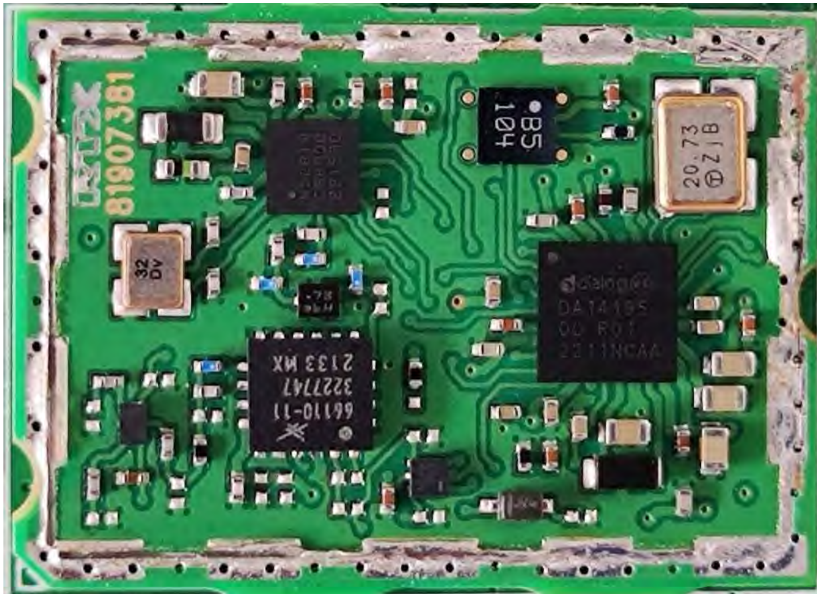
RTX1290 without shield case
