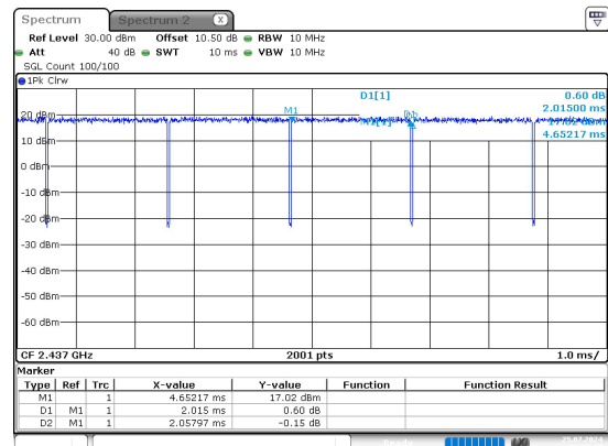
g_2437MHz_Chain 0
