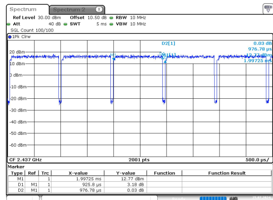
n40_2437MHz_Chain 0
