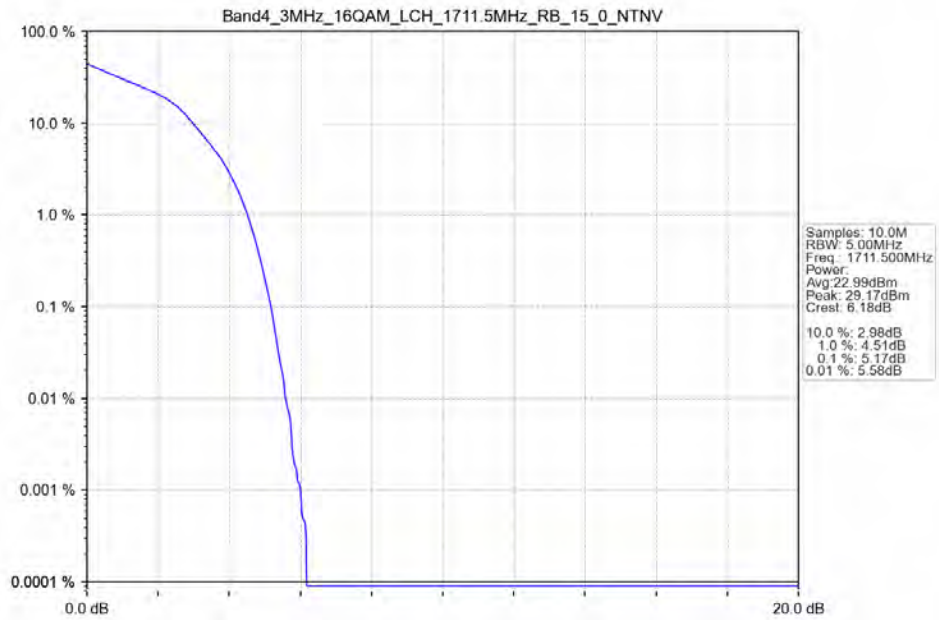
Band4_3MHz_16QAM_LCH_1711.5MHz_RB_15_0_NTNV
