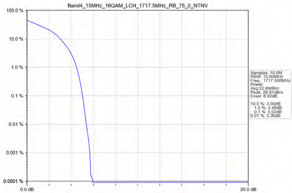
Band4_15MHz_16QAM_LCH_1717.5MHz_RB_75_0_NTNV
