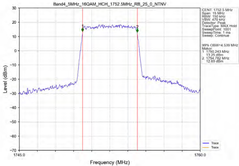
Band4_5MHz_16QAM_HCH_1752.5MHz_RB_25_0_NTNV
