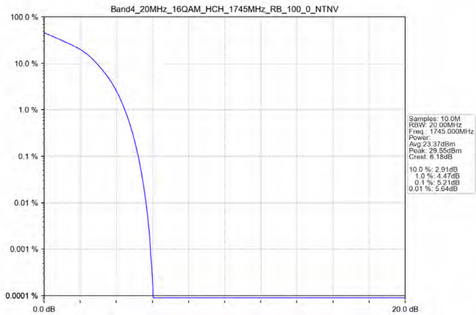
Band4_20MHz_16QAM_HCH_1745MHz_RB_100_0_NTNV
