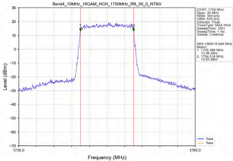
Band4_10MHz_16QAM_HCH_1750MHz_RB_50_0_NTNV
