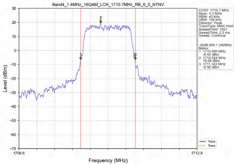
Band4_1.4MHz_16QAM_LCH_1710.7MHz_RB_6_0_NTNV
