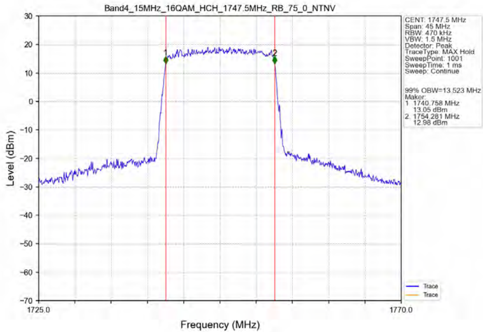
Band4_15MHz_16QAM_HCH_1747.5MHz_RB_75_0_NTNV
