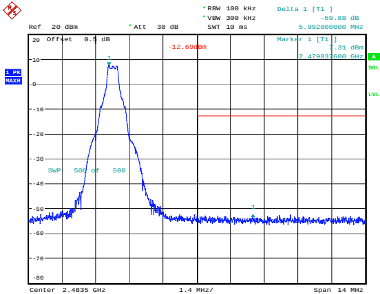
GFSK_High 59.88dB
