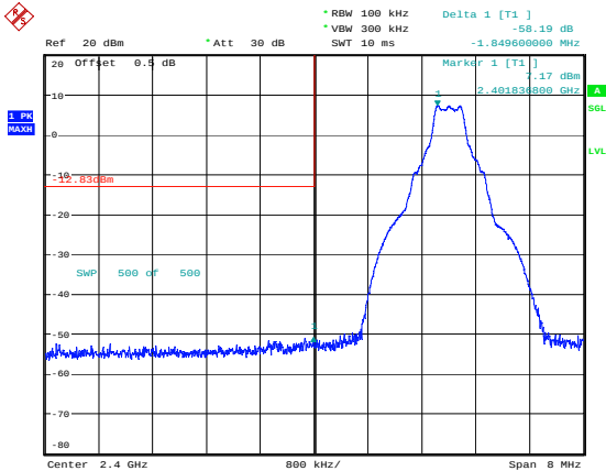
GFSK_Low 58.19dB
