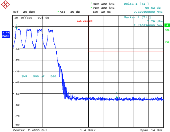
GFSK_Hopping_Upper 60.63dB
