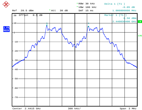
GFSK_Middle 1.001MHz
