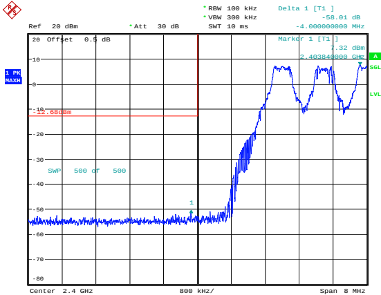
GFSK_Hopping_Lower 58.01dB
