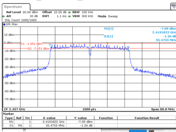
n40_2437MHz_Chain 0 35.475MHz
