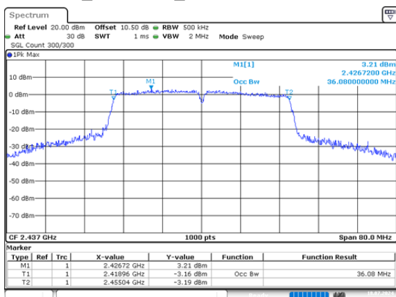
n40_2437MHz_Chain 0 36.080MHz
