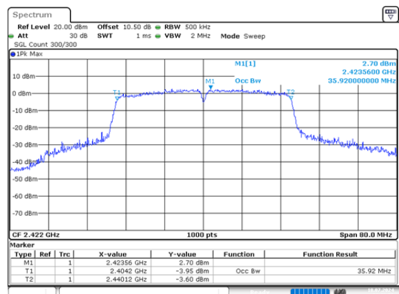
n40_2422MHz_Chain 0 35.920MHz
