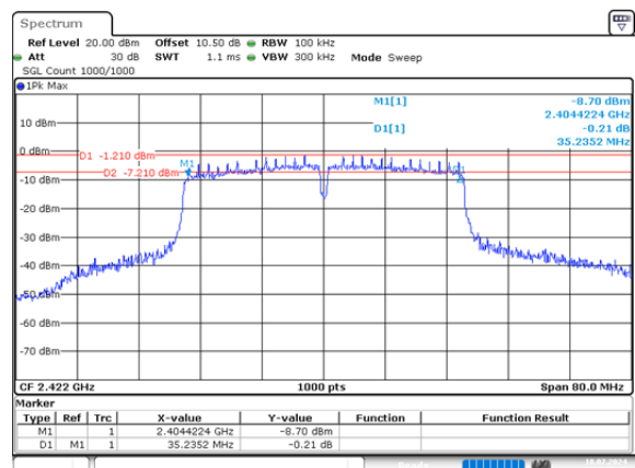
n40_2422MHz_Chain 0 35.235MHz
