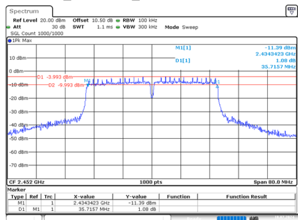
n40_2452MHz_Chain 0 35.716MHz
