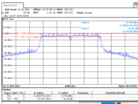
n20_2462MHz_Chain 0 17.017MHz
