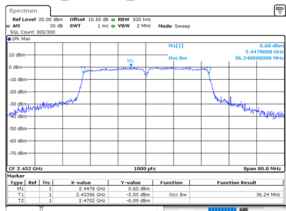
n40_2452MHz_Chain 0 36.240MHz
