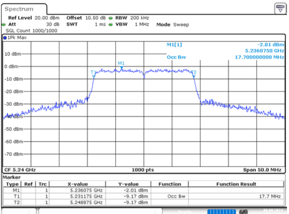
n20_5240MHz_Chain 0 17.700MHz
