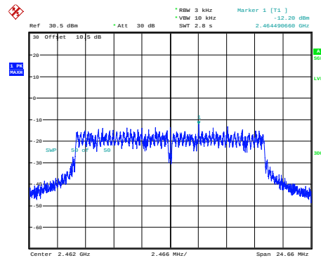
g_2462MHz_Chain 0
