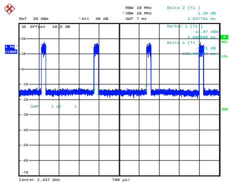
n20_2437MHz_Chain 0
