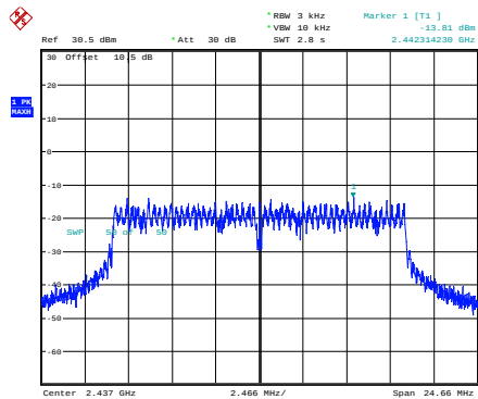
g_2437MHz_Chain 0
