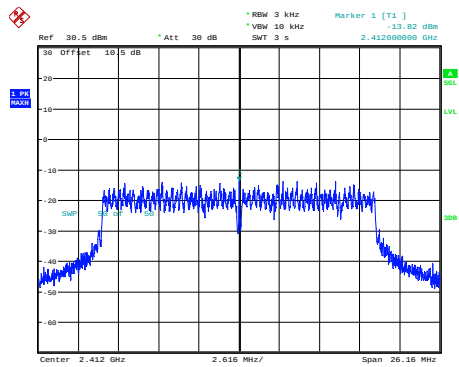
n20_2412MHz_Chain 0
