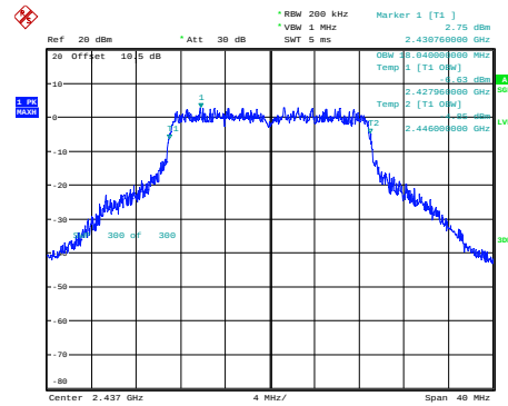
n20_2437MHz_Chain 0
