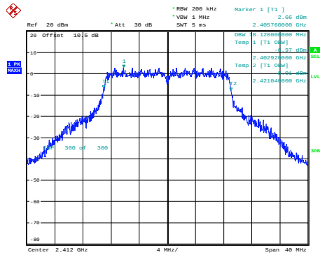
n20_2412MHz_Chain 0
