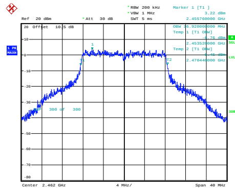
g_2462MHz_Chain 0
