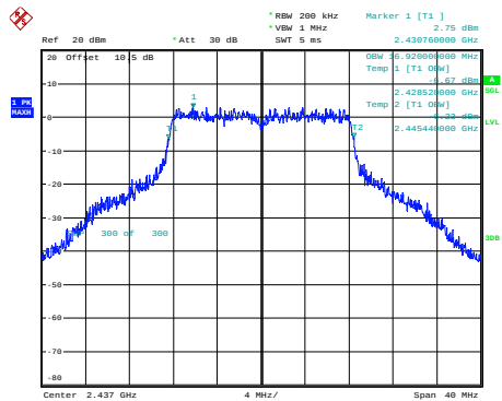
g_2437MHz_Chain 0
