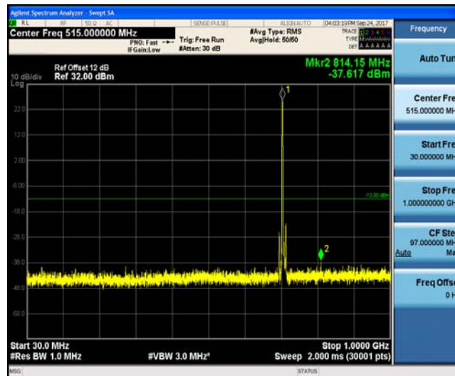
Band12_5MHz_16QAM_23155_1RB#0_Range4:1000~5000MHz_-45.32_PASS
