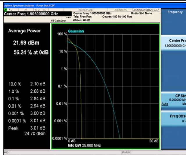
Band2_10MHz_16QAM_19150_1RB#0_3.81_13_PASS
