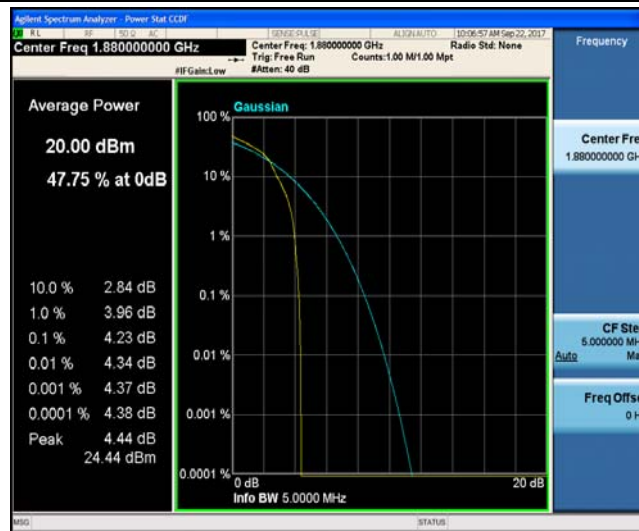
Band2_5MHz_QPSK_18900_25RB#0_5.18_13_PASS
