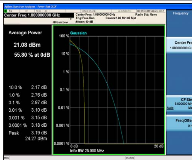
Band2_10MHz_16QAM_18900_1RB#0_3.93_13_PASS
