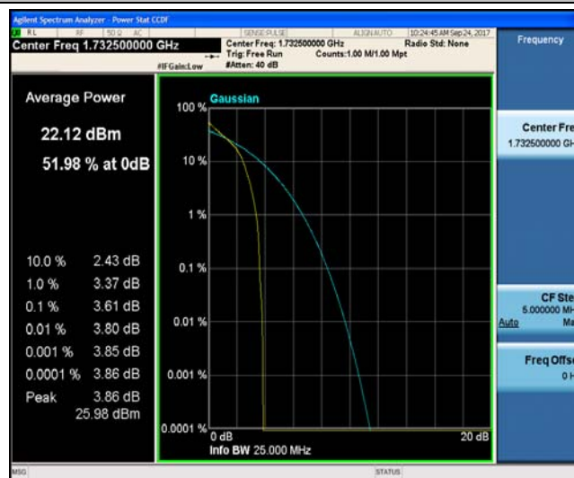
Band4_10MHz_16QAM_20175_1RB#0_4.54_13_PASS
