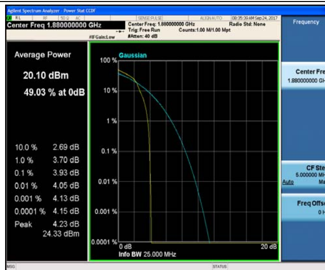
Band2_10MHz_QPSK_18900_50RB#0_4.70_13_PASS
