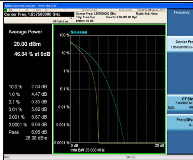
Band2_15MHz_16QAM_18675_75RB#0_6.08_13_PASS
