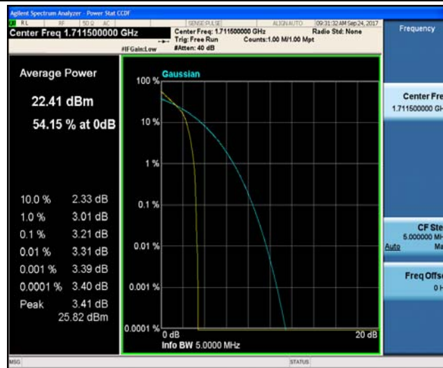
Band4_3MHz_16QAM_19965_1RB#0_4.16_13_PASS
