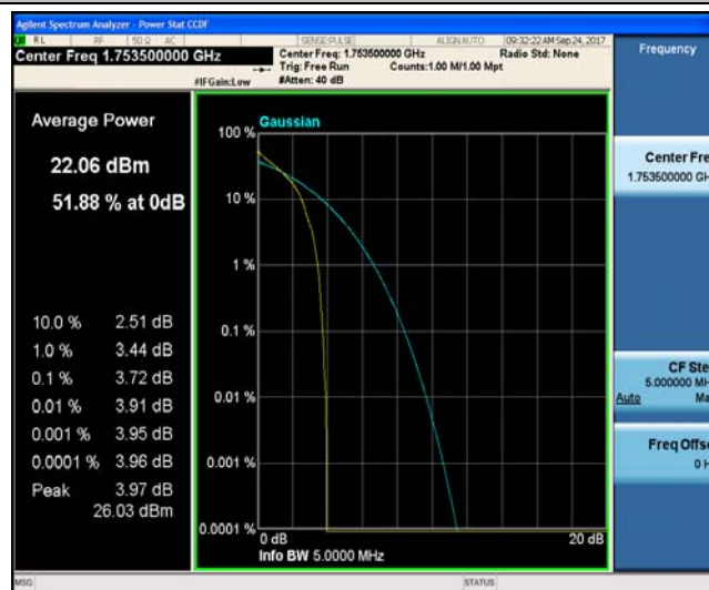
Band4_3MHz_16QAM_20385_1RB#0_4.66_13_PASS
