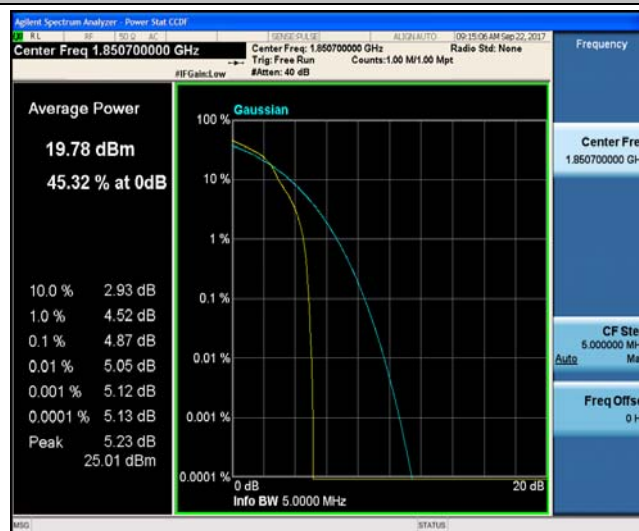
Band2_1.4MHz_QPSK_18607_6RB#0_4.98_13_PASS
