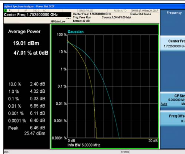
Band4_5MHz_16QAM_20375_25RB#0_6.07_13_PASS
