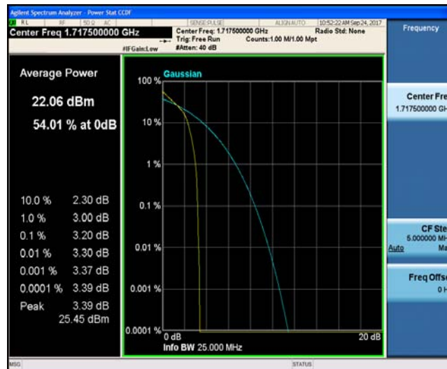
Band4_15MHz_16QAM_20025_1RB#0_4.12_13_PASS
