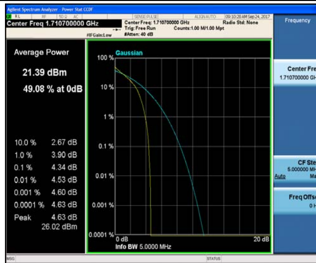
Band4_1.4MHz_16QAM_19957_6RB#0_5.29_13_PASS
