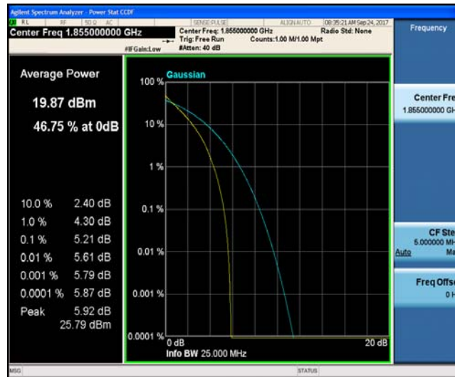
Band2_10MHz_16QAM_18650_50RB#0_6.01_13_PASS
