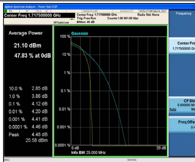
Band4_15MHz_QPSK_20025_75RB#0_5.24_13_PASS
