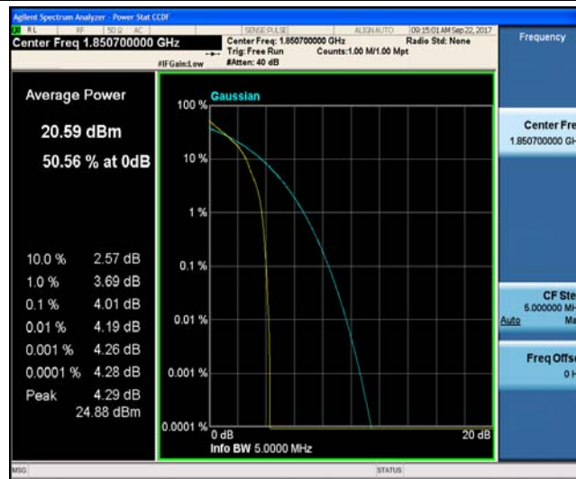
Band2_1.4MHz_16QAM_18607_1RB#0_4.87_13_PASS
