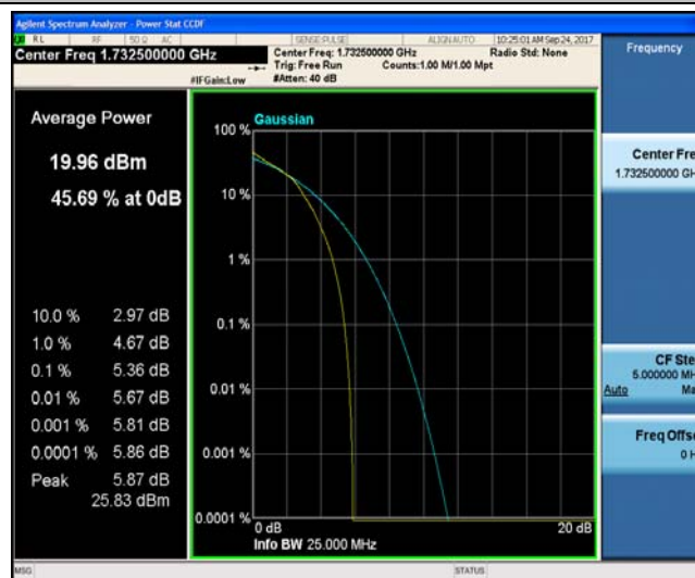
Band4_10MHz_QPSK_20350_1RB#0_3.60_13_PASS
