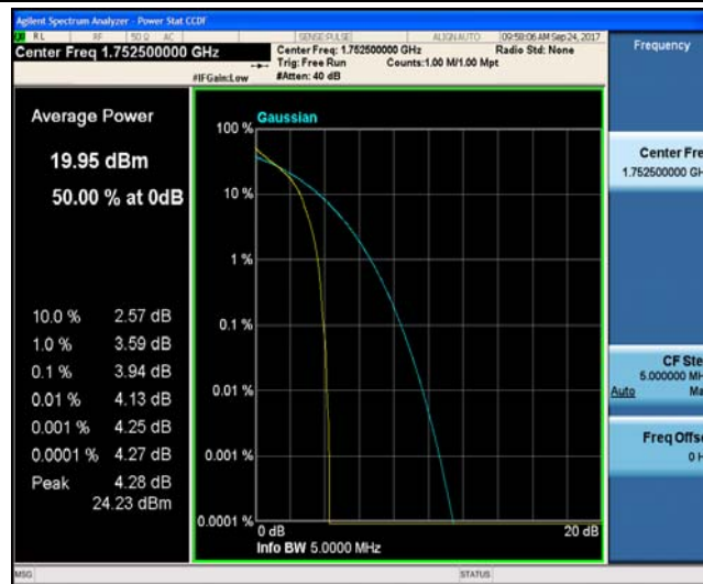
Band4_5MHz_16QAM_20375_1RB#0_4.80_13_PASS
