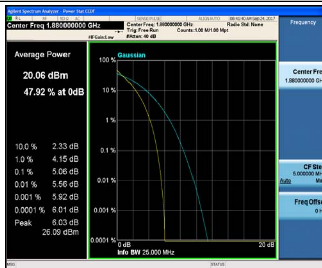
Band2_20MHz_16QAM_18900_100RB#0_5.86_13_PASS
