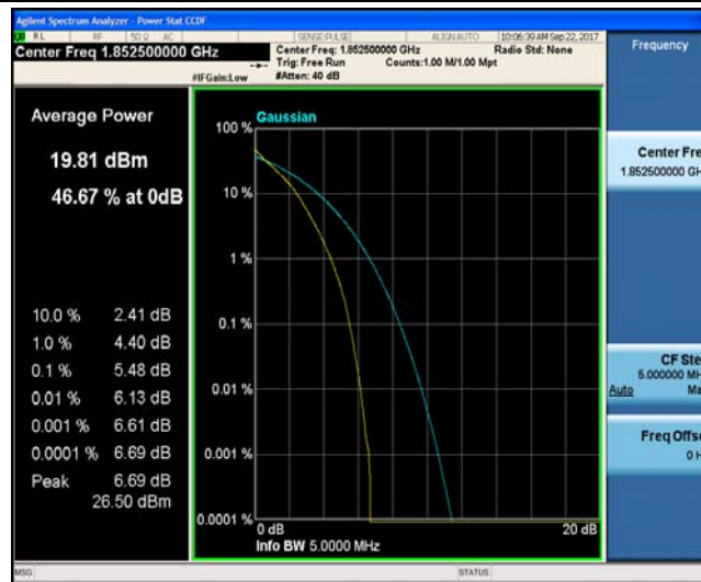
Band2_5MHz_16QAM_18625_25RB#0_6.15_13_PASS
