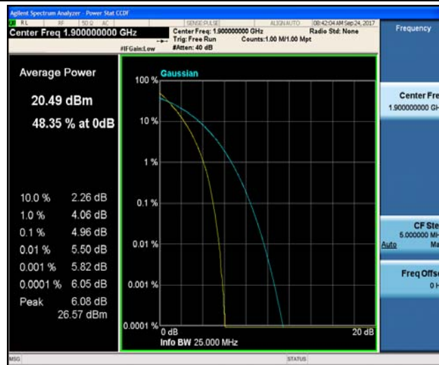
Band2_20MHz_16QAM_19100_100RB#0_5.73_13_PASS
