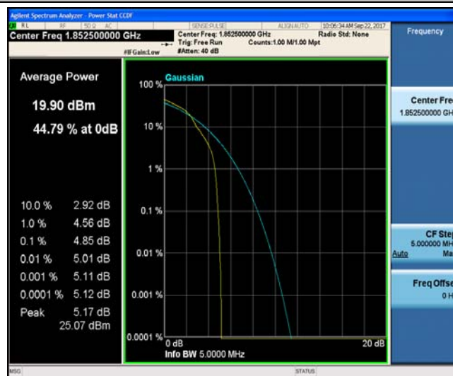
Band2_5MHz_QPSK_18625_25RB#0_5.48_13_PASS
