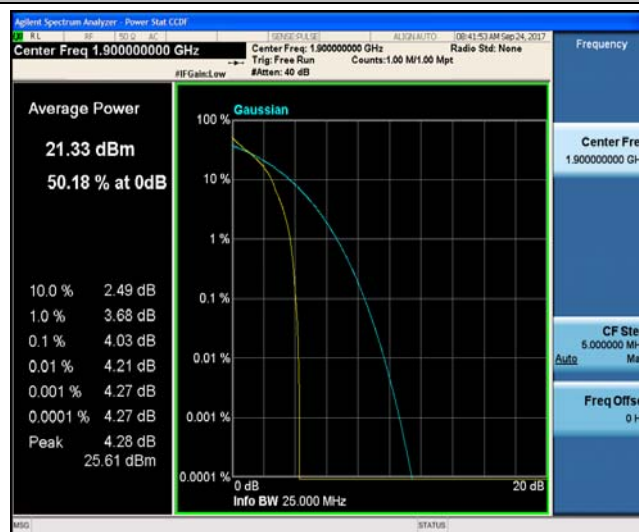
Band2_20MHz_16QAM_19100_1RB#0_4.82_13_PASS
