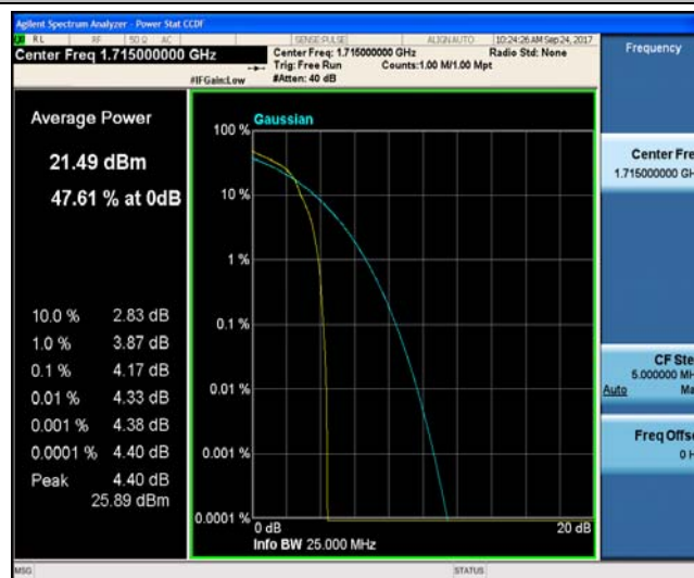
Band4_10MHz_QPSK_20000_50RB#0_4.87_13_PASS
