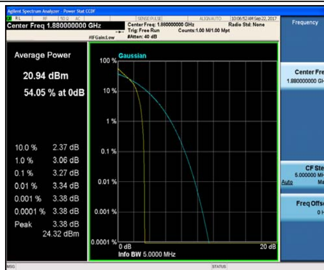
Band2_5MHz_16QAM_18900_1RB#0_4.23_13_PASS
