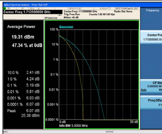
Band4_5MHz_16QAM_19975_25RB#0_5.92_13_PASS
