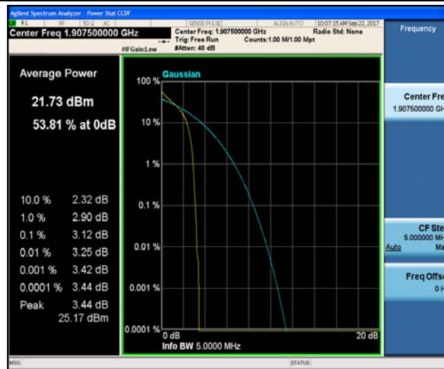
Band2_5MHz_16QAM_19175_1RB#0_3.96_13_PASS
