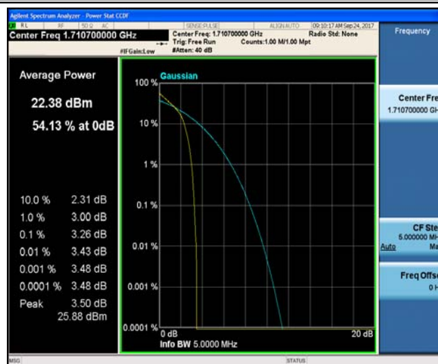
Band4_1.4MHz_16QAM_19957_1RB#0_4.27_13_PASS
