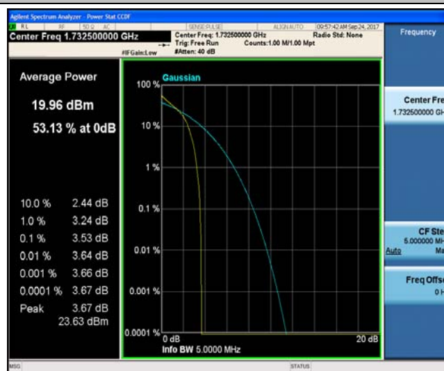
Band4_5MHz_16QAM_20175_1RB#0_4.50_13_PASS
