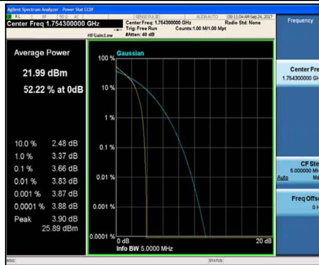
Band4_1.4MHz_16QAM_20393_1RB#0_4.59_13_PASS
