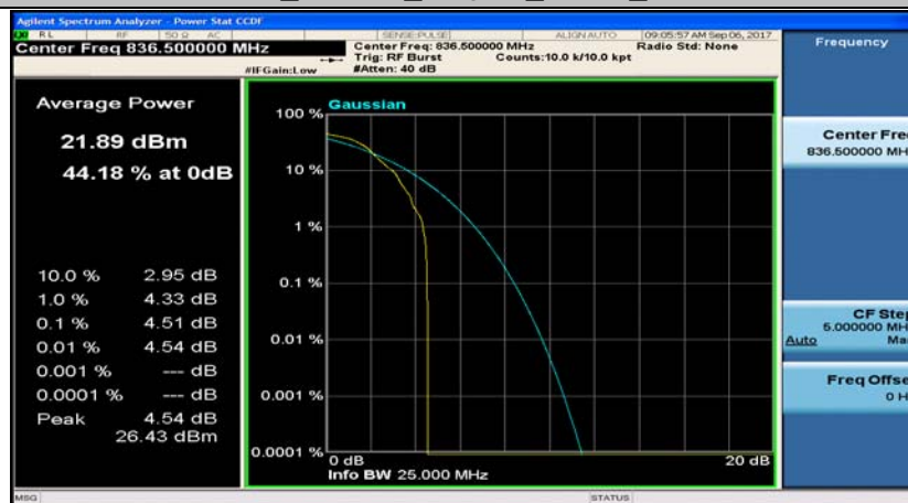
Band5_1.4MHz_QPSK_20525_6RB#0
