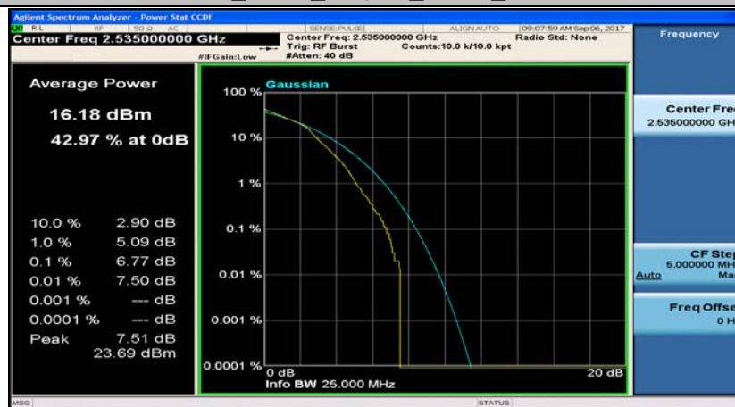
Band7_10MHz_QPSK_21100_1RB#0
