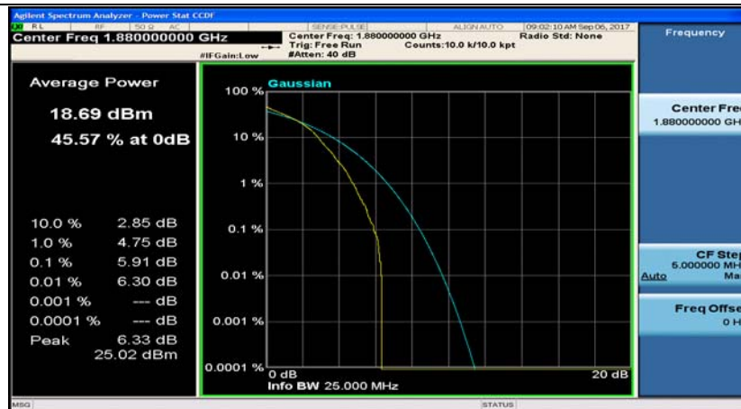
Band2_20MHz_QPSK_18900_1RB#0
