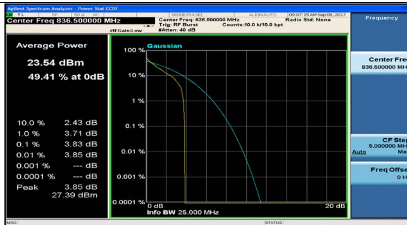
Band5_10MHz_16QAM_20525_1RB#0
