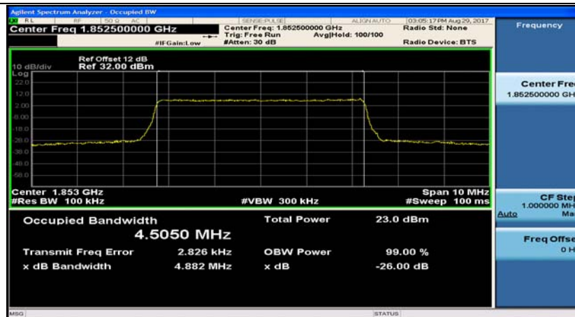
Band2_5MHz_16QAM_18625_25RB#0
