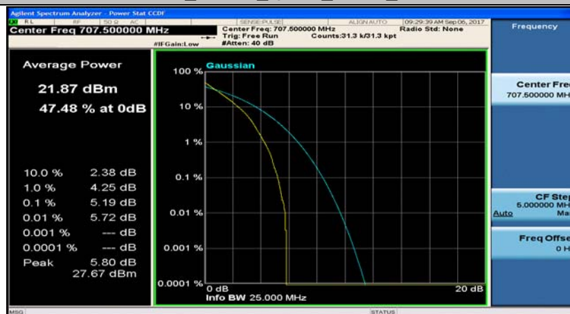
Band12_10MHz_16QAM_23095_50RB#0
