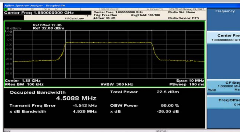
Band2_5MHz_16QAM_18900_25RB#0
