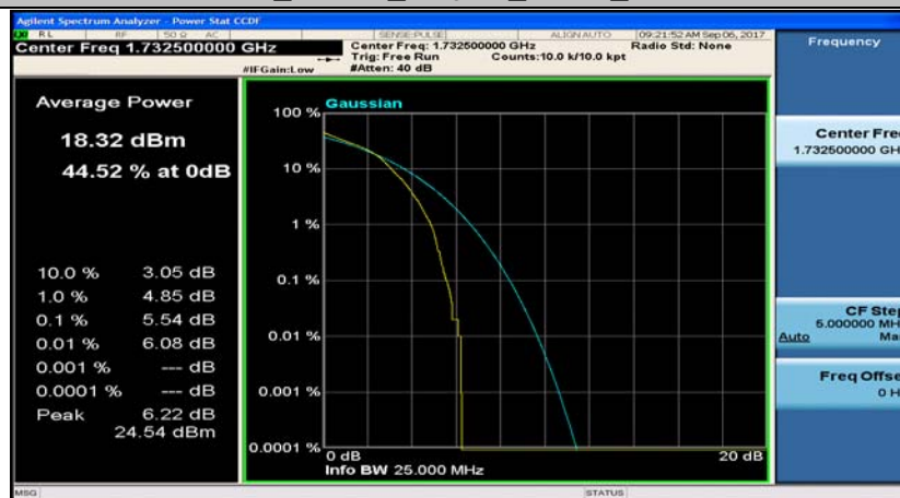
Band4_20MHz_QPSK_20175_100RB#0
