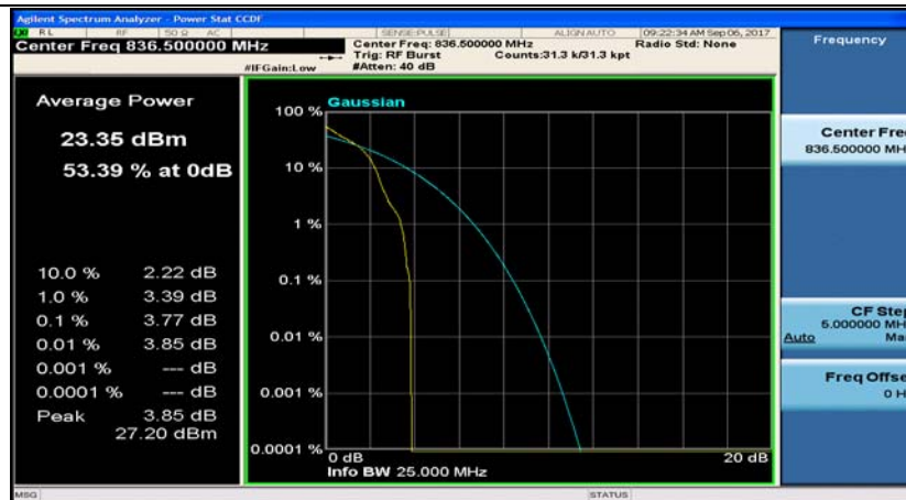
Band5_1.4MHz_16QAM_20525_1RB#0
