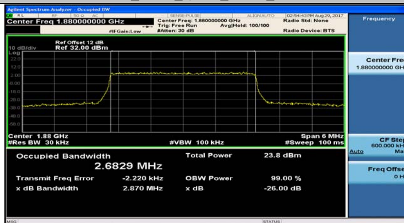
Band2_3MHz_16QAM_18900_15RB#0
