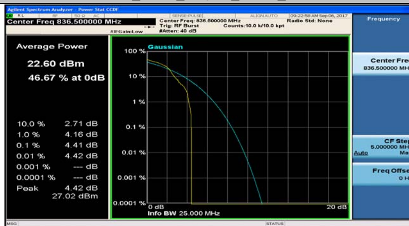
Band5_5MHz_QPSK_20525_1RB#0
