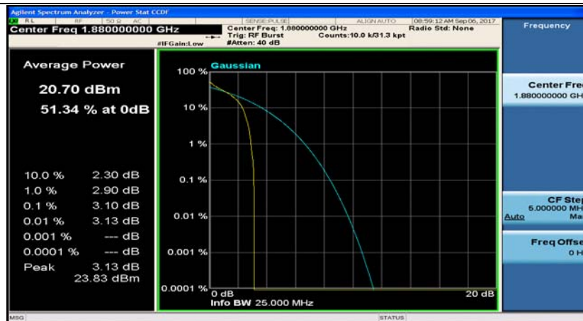
Band2_3MHz_16QAM_18900_1RB#0
