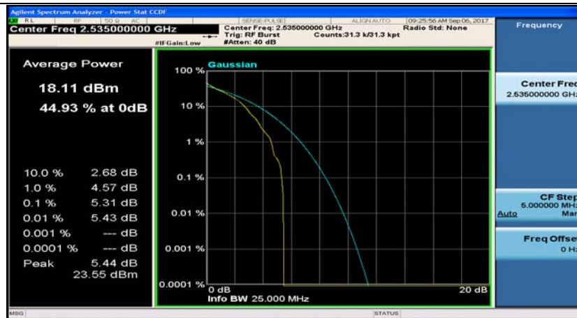
Band7_15MHz_16QAM_21100_1RB#0
