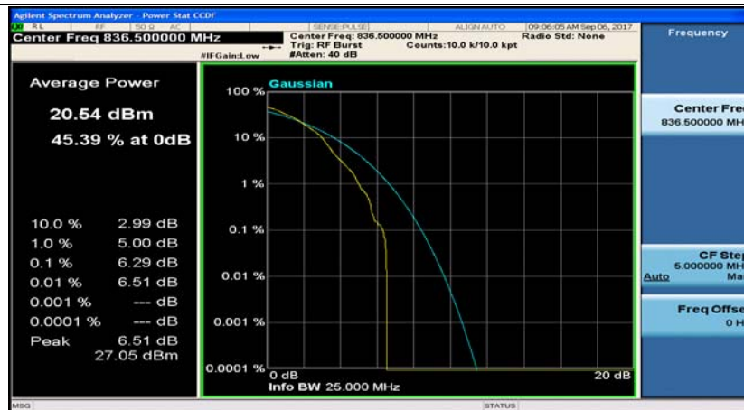
Band5_3MHz_QPSK_20525_15RB#0
