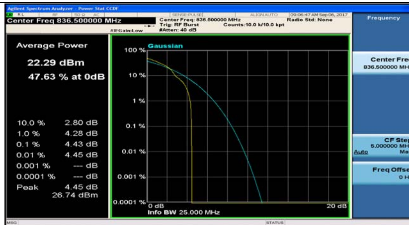
Band5_5MHz_QPSK_20525_25RB#0
