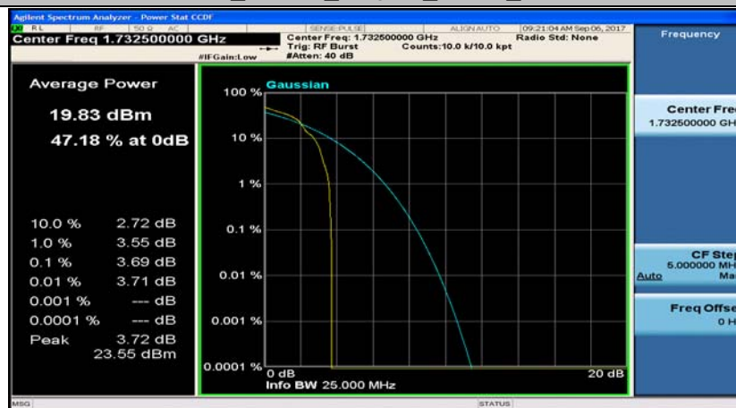
Band4_10MHz_QPSK_20175_50RB#0
