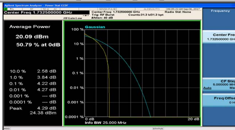
Band4_20MHz_16QAM_20175_1RB#0
