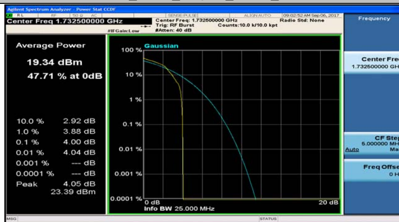
Band4_5MHz_QPSK_20175_1RB#0
