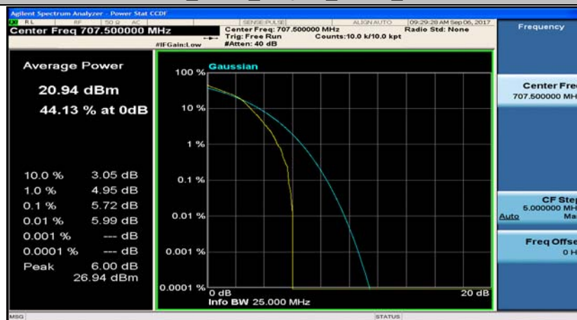
Band12_10MHz_QPSK_23095_50RB#0
