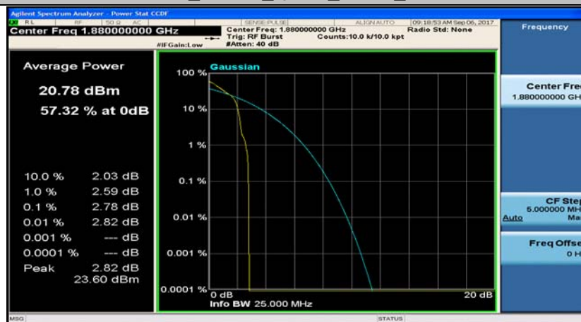
Band2_15MHz_16QAM_18900_1RB#0
