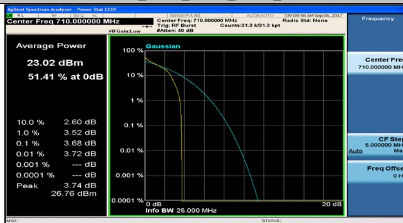
Band17_5MHz_16QAM_23790_1RB#0
