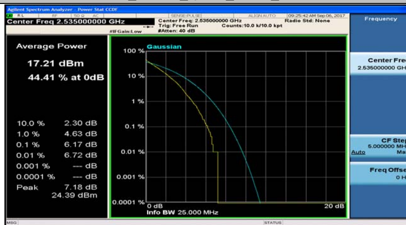
Band7_10MHz_16QAM_21100_50RB#0
