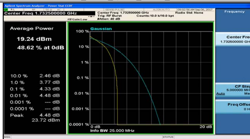
Band4_3MHz_16QAM_20175_15RB#0
