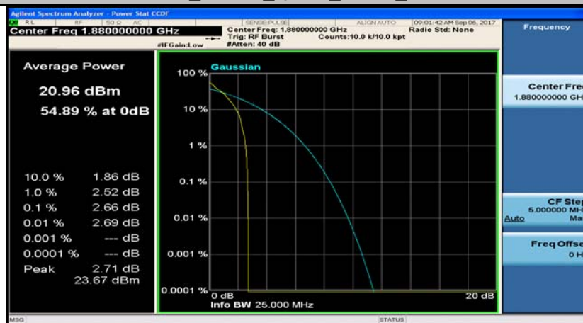
Band2_20MHz_16QAM_18900_1RB#0
