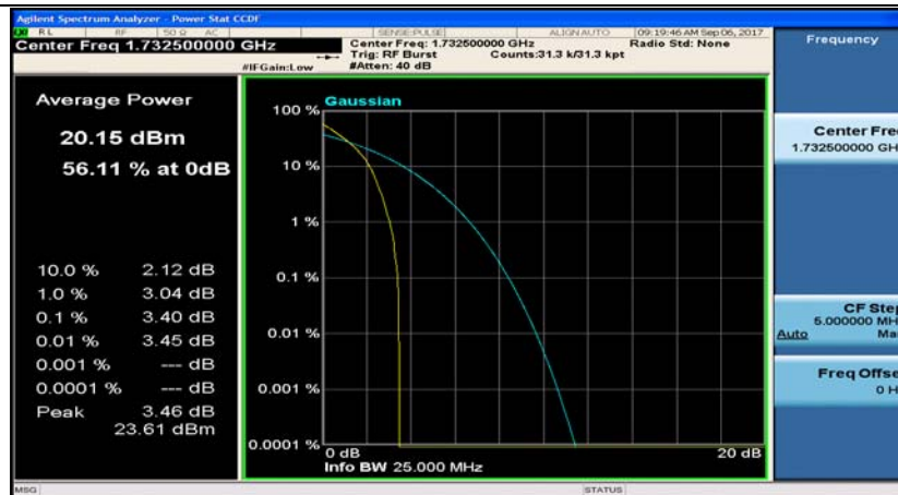
Band4_1.4MHz_16QAM_20175_1RB#0
