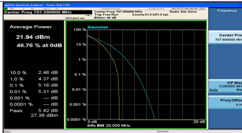
Band12_5MHz_16QAM_23095_25RB#0
