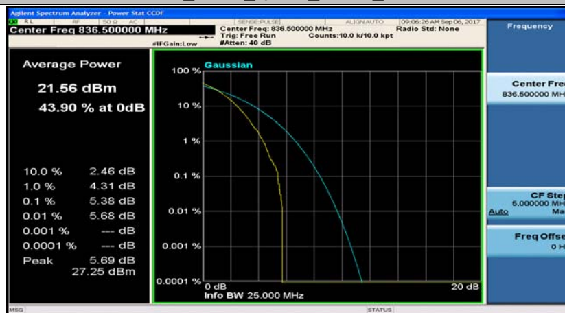
Band5_3MHz_16QAM_20525_15RB#0
