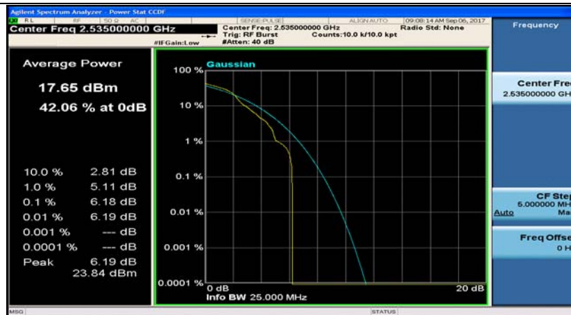
Band7_10MHz_QPSK_21100_50RB#0
