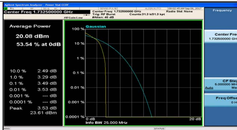
Band4_3MHz_16QAM_20175_1RB#0
