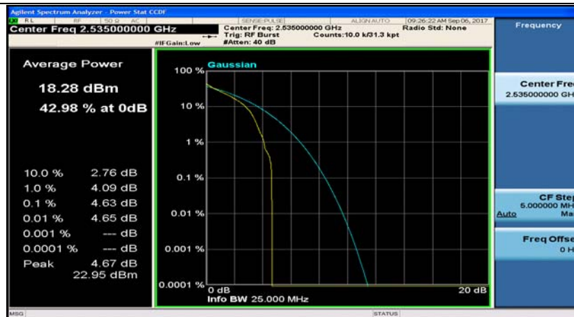
Band7_20MHz_16QAM_21100_1RB#0
