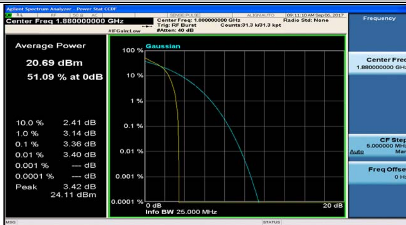
Band2_1.4MHz_16QAM_18900_1RB#0
