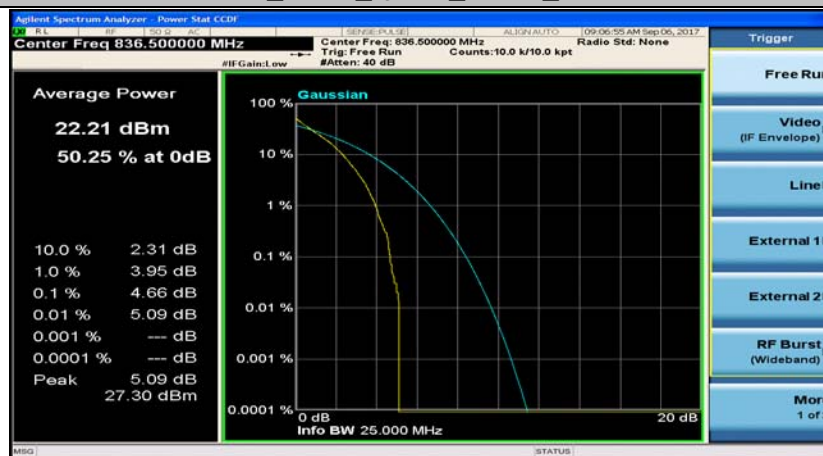
Band5_5MHz_16QAM_20525_25RB#0
