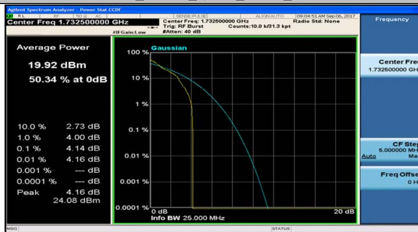
Band4_15MHz_16QAM_20175_1RB#0
