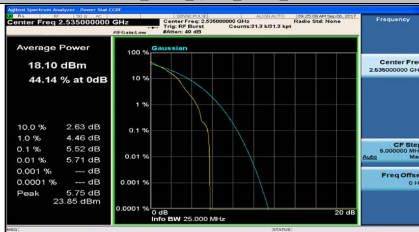
Band7_5MHz_16QAM_21100_1RB#0
