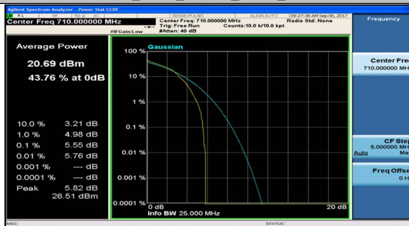
Band17_10MHz_QPSK_23790_1RB#0
