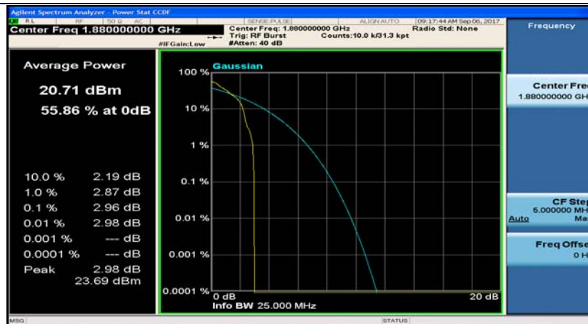
Band2_10MHz_16QAM_18900_1RB#0
