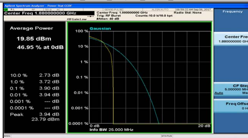
Band2_5MHz_QPSK_18900_1RB#0
