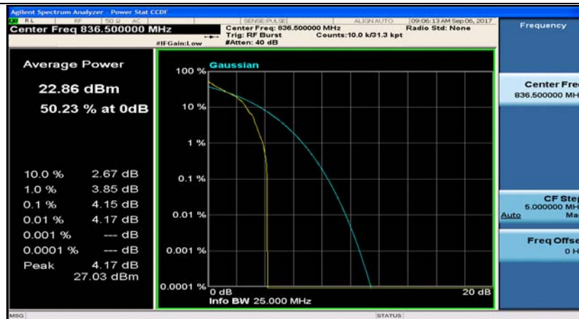
Band5_3MHz_16QAM_20525_1RB#0
