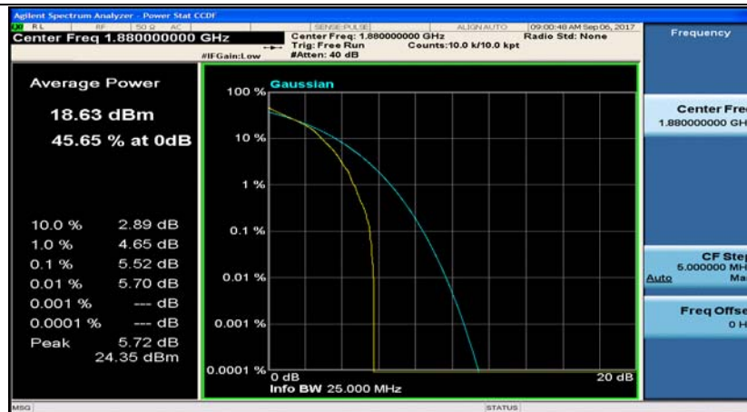
Band2_15MHz_QPSK_18900_1RB#0
