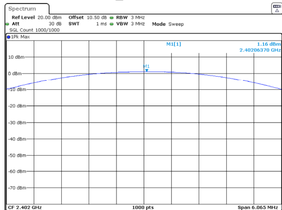
2DH1_Low 1.16dBm
