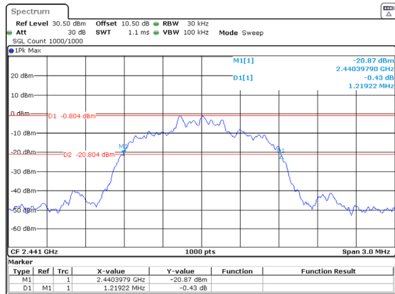
3DH1_Middle 1.219MHz
