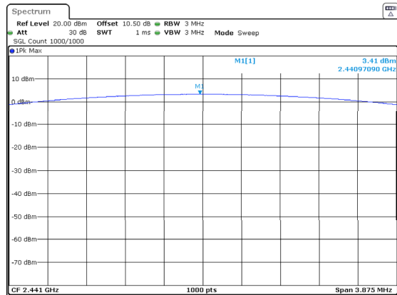
DH1_Middle 3.41dBm
