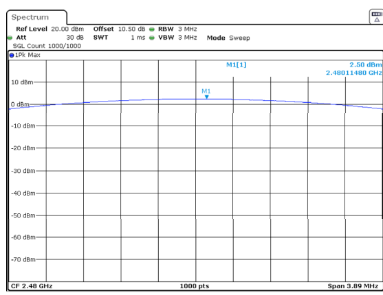
DH1_High 2.50dBm
