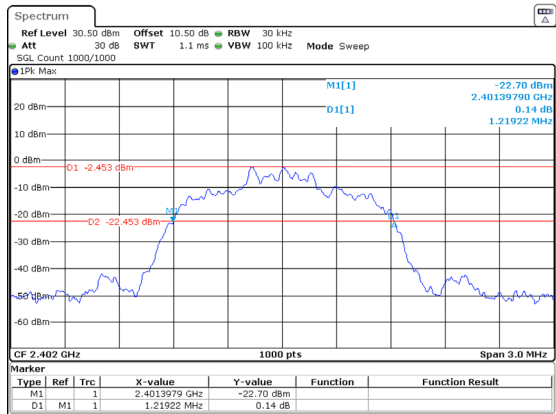
3DH1_Low 1.219MHz
