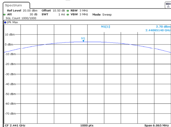
2DH1_Middle 2.70dBm
