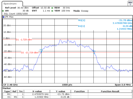
3DH1_High 1.219MHz
