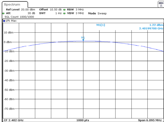
3DH1_Low 1.22dBm
