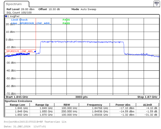
Band 2 15MHz/1857.5/Low QPSK 75@0
