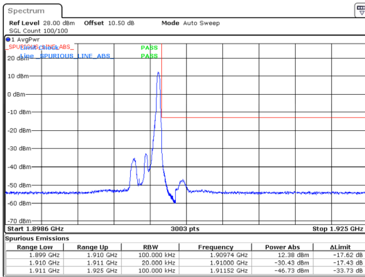
Band 2 1.4MHz/1909.3/High QPSK 1@5
