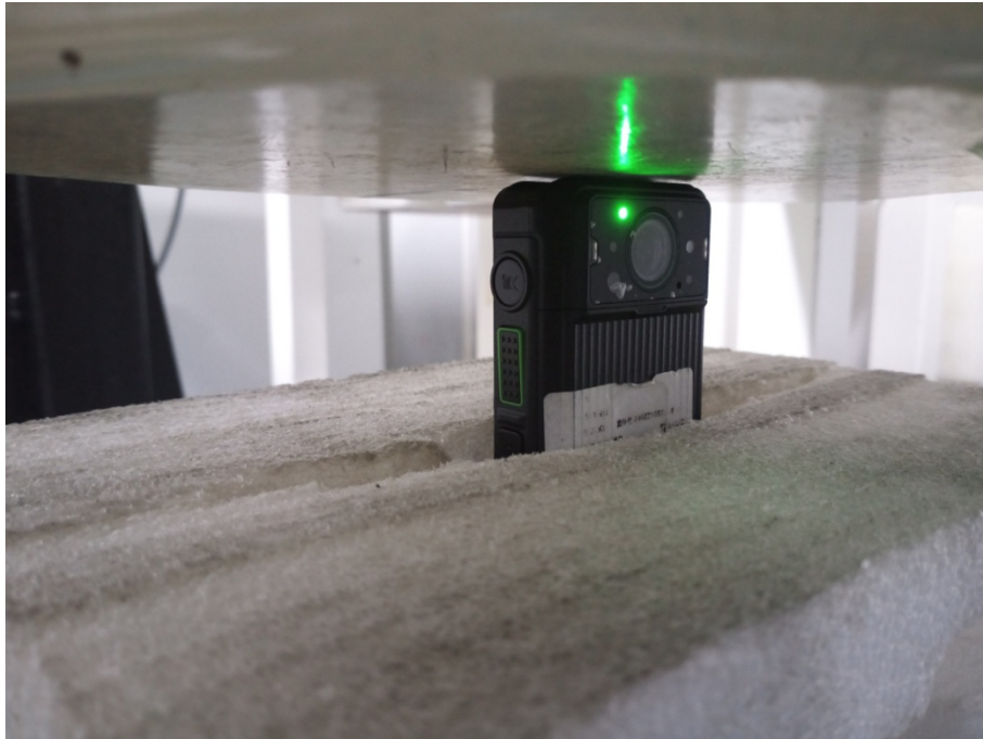
Limb Top Setup Photo(0mm)
