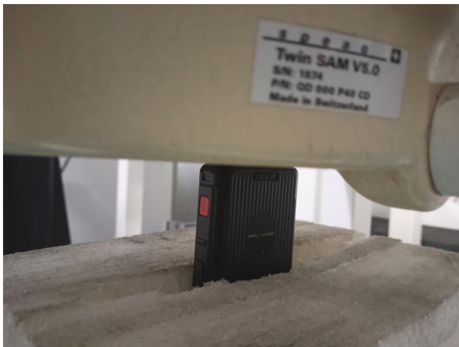
Limb Bottom Setup Photo(0mm)
