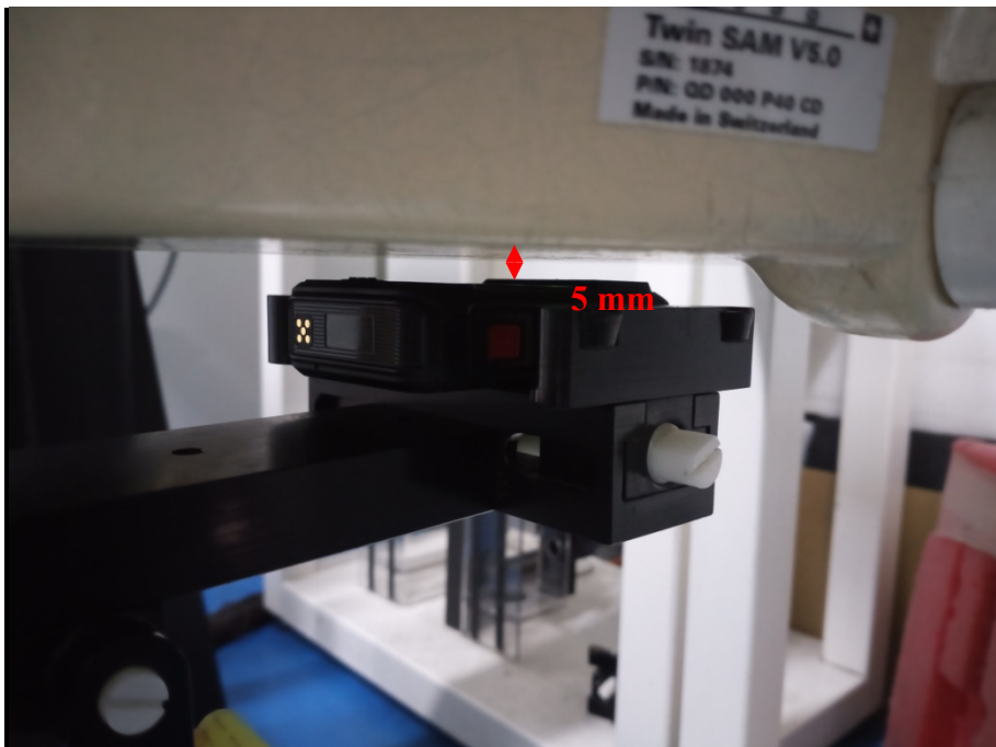
Body Front Setup Photo(5mm)
