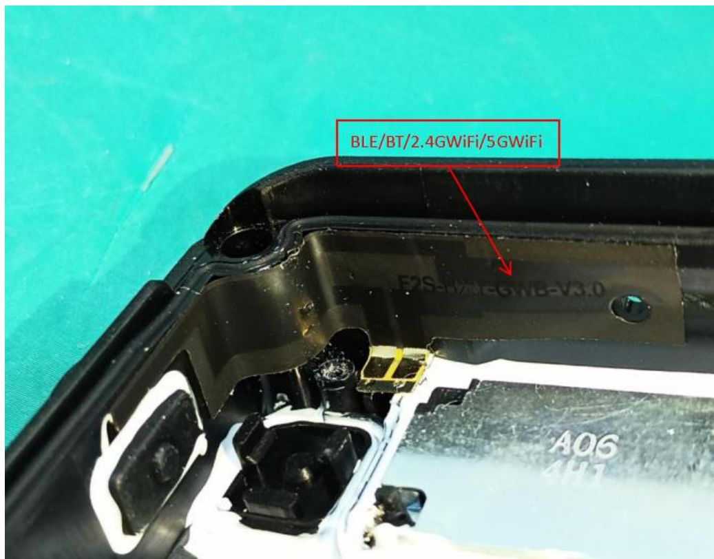
BT/Wi-Fi ANT
