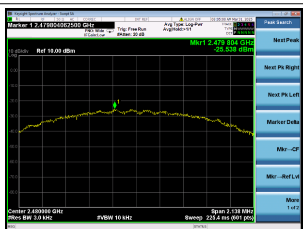
Bluetooth Low Energy 2Mbps 2480MHz
