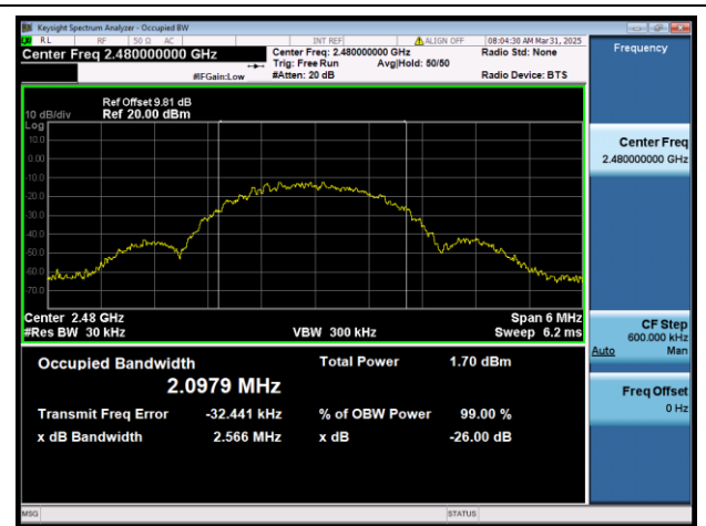
Bluetooth Low Energy 2Mbps 2480MHz
