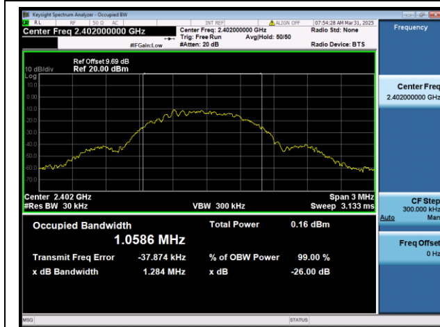
Bluetooth Low Energy 1Mbps 2402MHz
