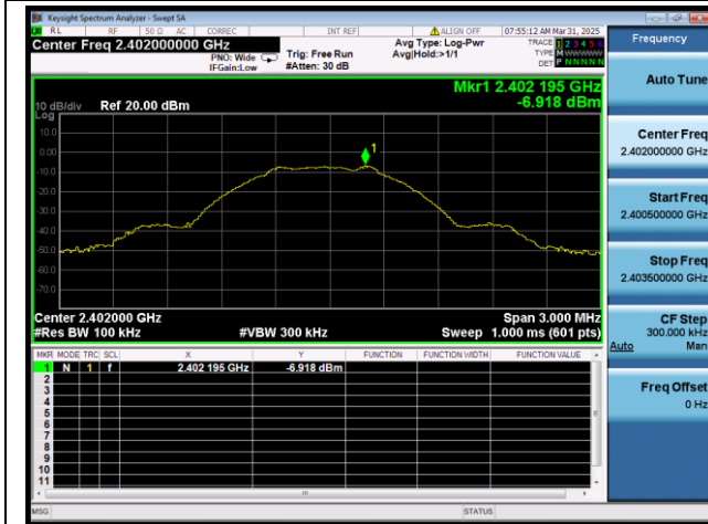
Bluetooth Low Energy 1Mbps
