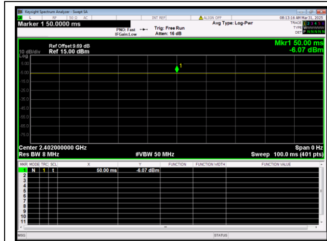
Bluetooth Low Energy 1Mbps 2402MHz
