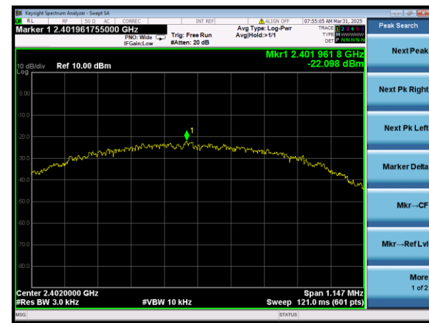
Bluetooth Low Energy 1Mbps 2402MHz
