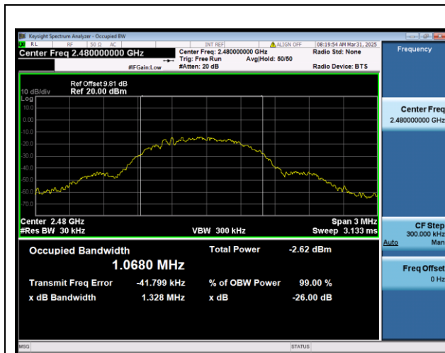
Bluetooth Low Energy 1Mbps 2480MHz
