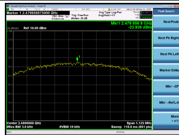
Bluetooth Low Energy 1Mbps 2480MHz
