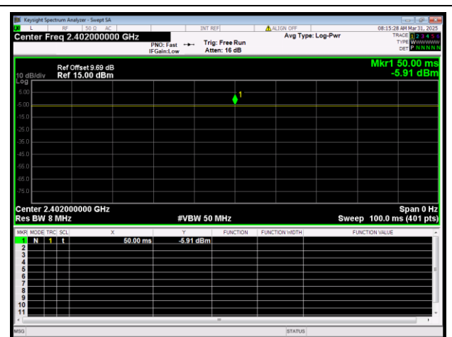
Bluetooth Low Energy 2Mbps 2402MHz
