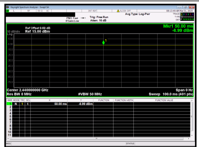
Bluetooth Low Energy 1Mbps 2440MHz
