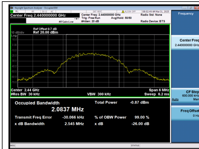
Bluetooth Low Energy 2Mbps 2440MHz
