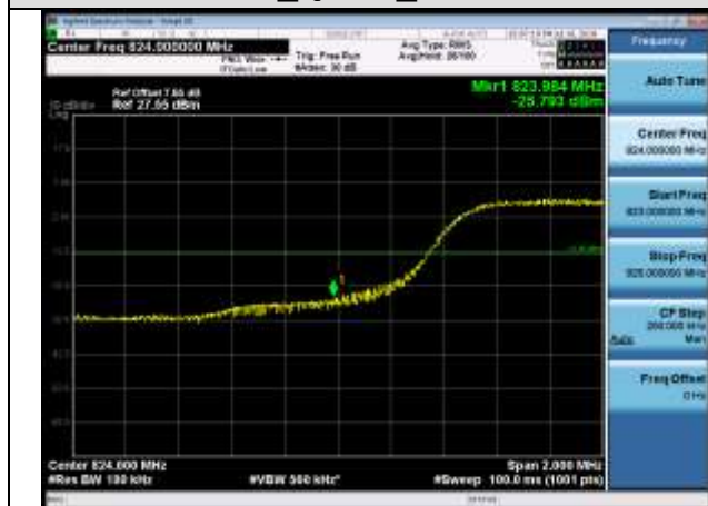
LCH_QPSK_50RB#0
