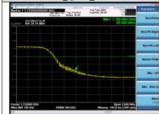
HCH_QPSK_50RB#0
