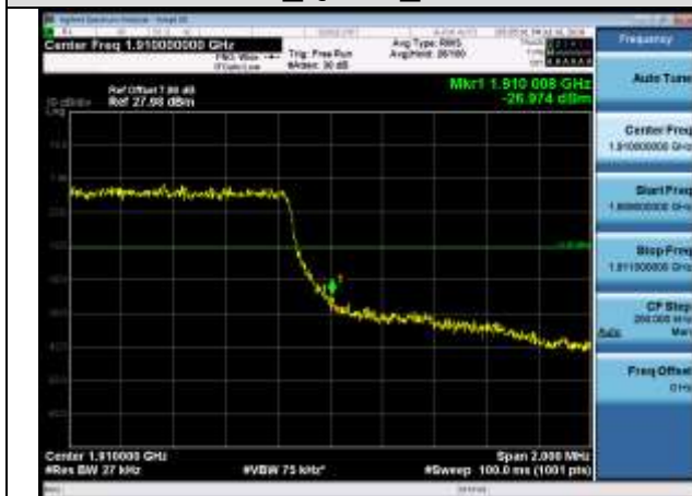
HCH_QPSK_6RB#0
