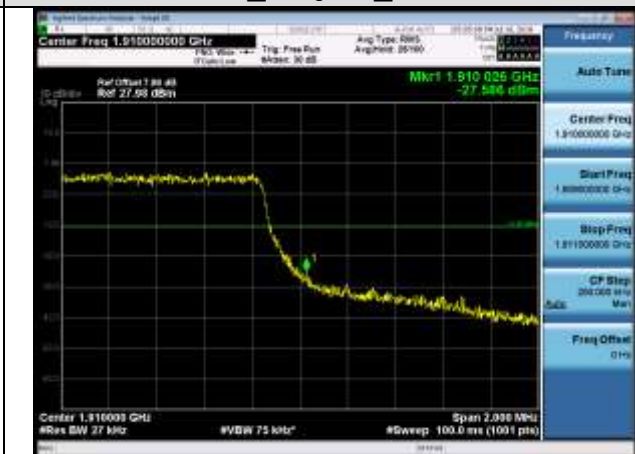
HCH_16QAM_6RB#0
