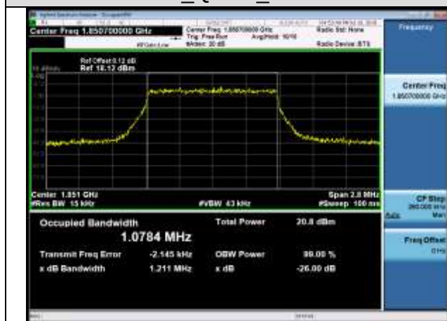
LCH_QPSK_6RB#0
