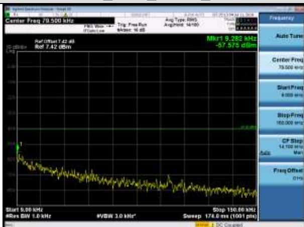
1.4MHz_HCH_QPSK_1RB#0
