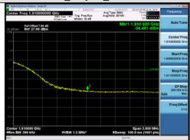
HCH_16QAM_100RB#0
