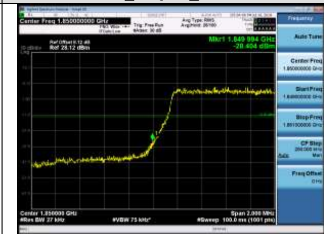
LCH_16QAM_6RB#0
