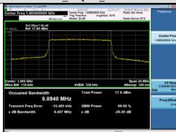
HCH_16QAM_50RB#0
