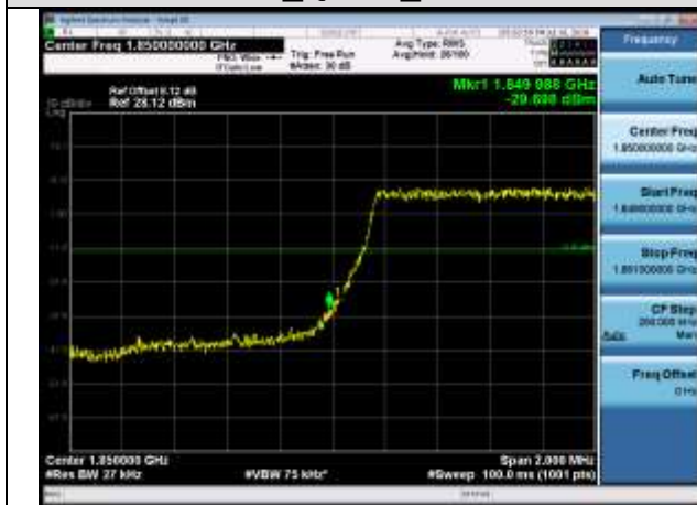
LCH_QPSK_6RB#0
