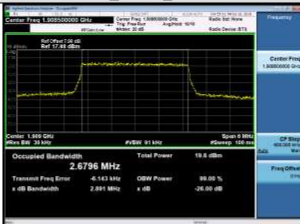
HCH_QPSK_15RB#0
