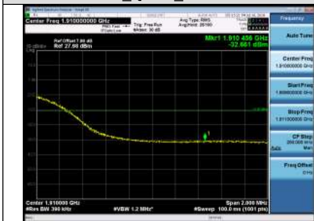
HCH_QPSK_100RB#0
