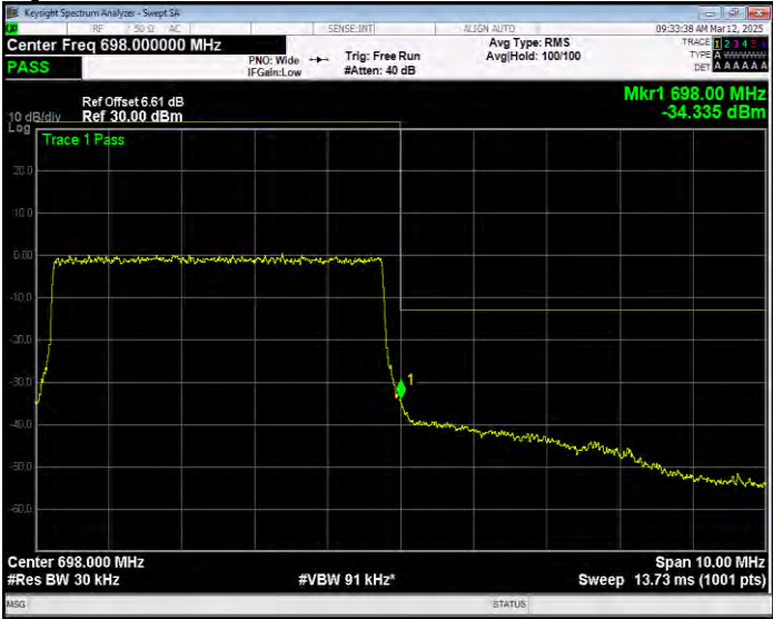
Band71 QPSK BW=5MHz Channel=133447 RB Size=1 Position=#Max Extended
