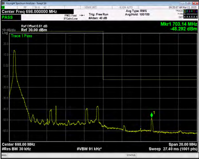
Band71 QPSK BW=15MHz Channel=133197 RB Size=1 Position=#0 Extended
